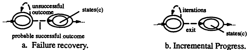
Figure 3. Completable repeat-loops.
