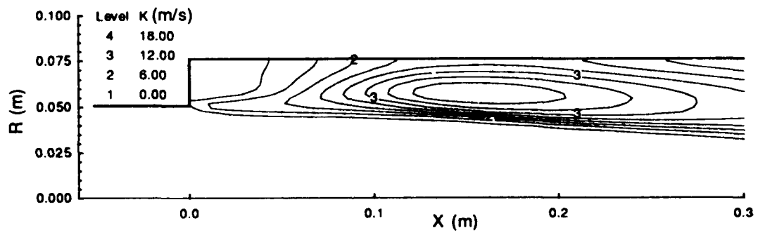
Figure 44: Calculated Turbulent Kinetic Energy Contours with C_\mu = 0.07 and C_{\epsilon 2} = 1.887 for S = 0.0 .
