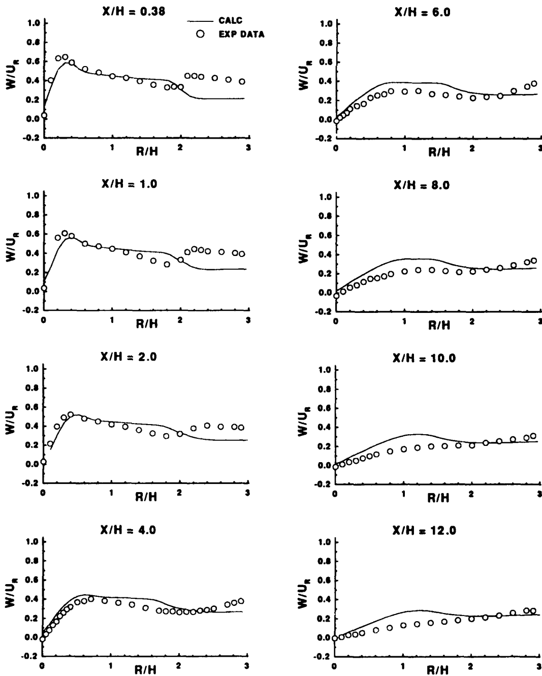
Figure 30: Swirl Velocity Profiles for S = 0.3 .
