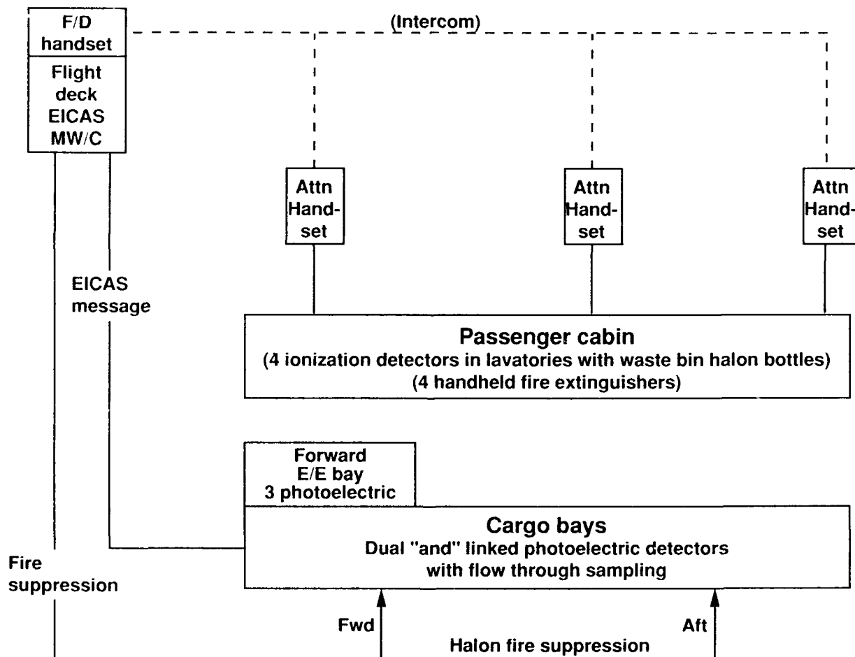
Figure 3-4. Existing 757-200 Fuselage Fire Protection System.
