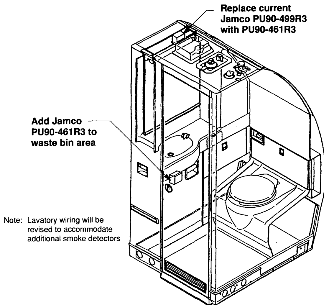
Figure 5-6. Concept A Modifications – Lavatory Features.
