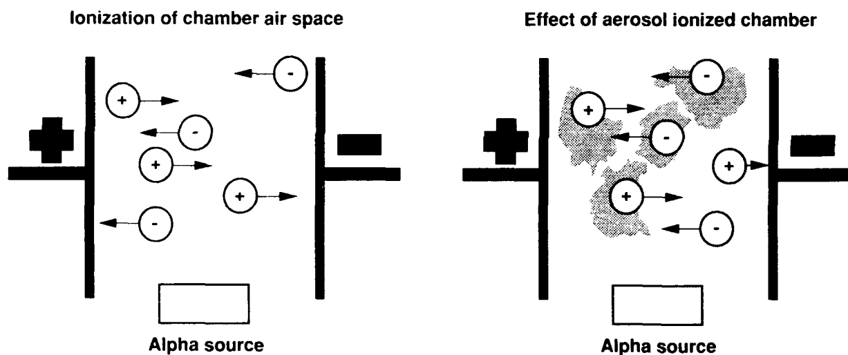
Figure 4-8. Ionization Detector.
