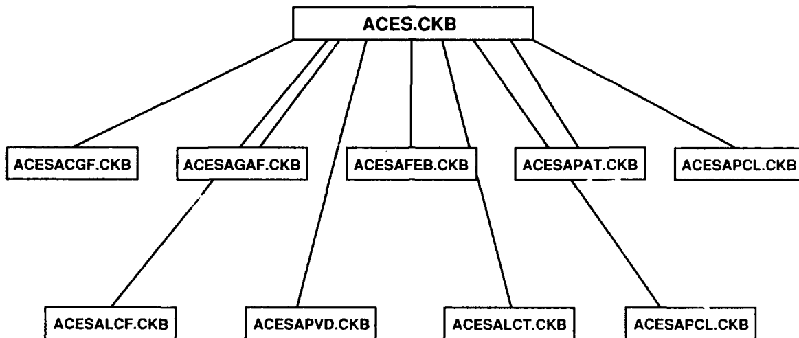
Figure 4-12. ACES Knowledge Base Partition
