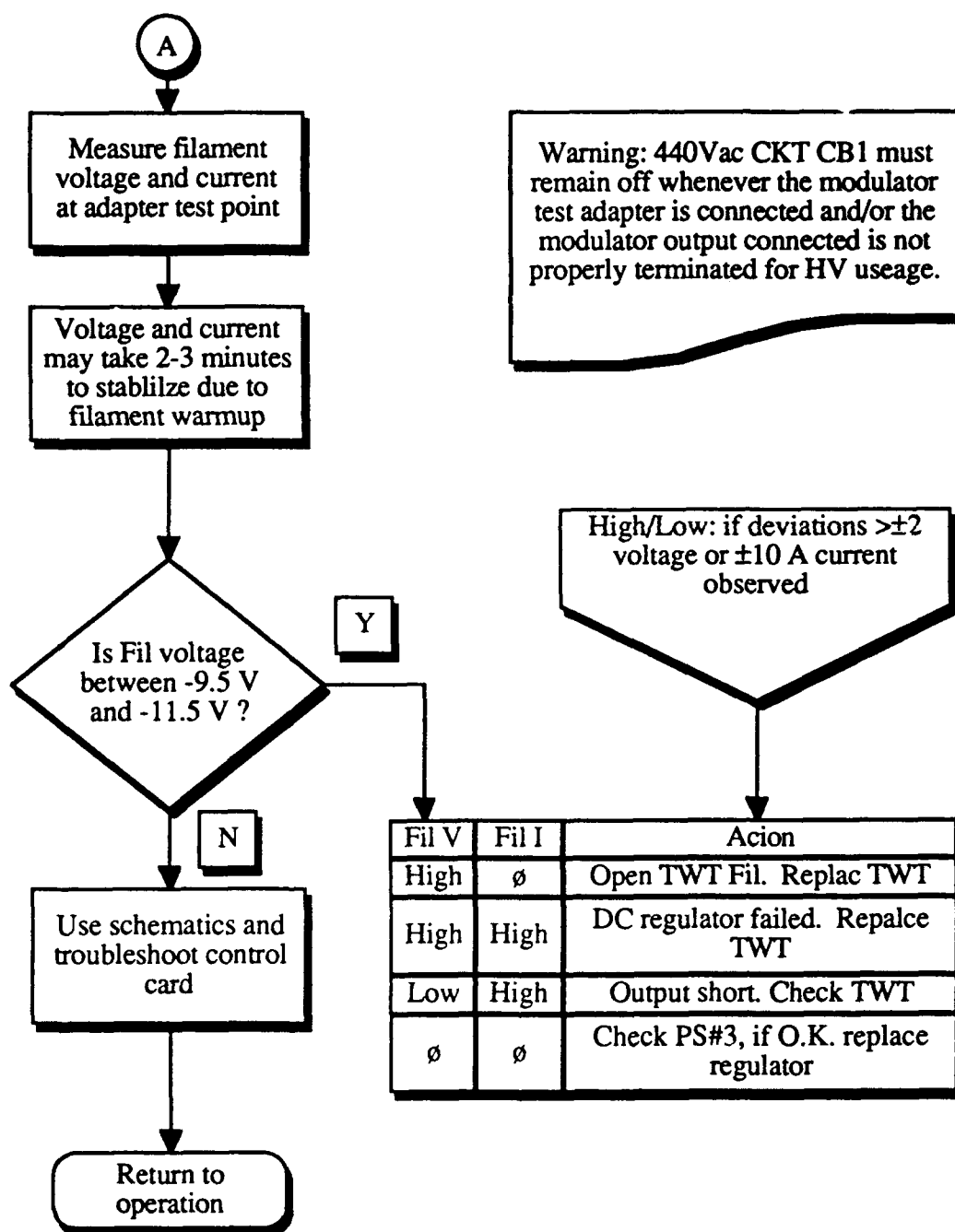
Figure B.8 Filament Voltage Regulator Fault Troubleshooting Flowchart (continued)
