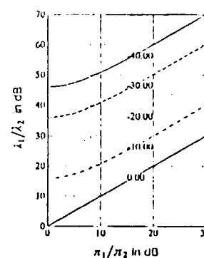
Figure 13. \lambda_1/\lambda_2 in dB vs \pi_1/\pi_2 in dB = 0, 5, 10, 15, 20, 25, 30 at \eta in dB = -40, -30, -20, -10, 0 for \xi = 0 .
