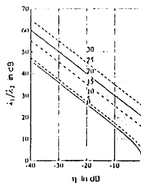
Figure 12. \lambda_1/\lambda_2 in dB vs \eta in dB = -40, -30, -20, -10, 0 at \pi_1/\pi_2 in dB = 0, 5, 10, 15, 20, 25, 30 for \xi = 0 .
