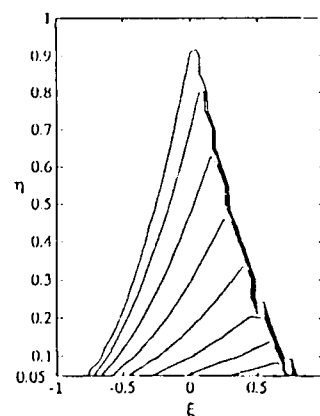
Figure 11. Parabolic contour plot of \lambda_1/\lambda_2 in dB as function of \xi and \eta for \pi_1/\pi_2 = 0 dB.
