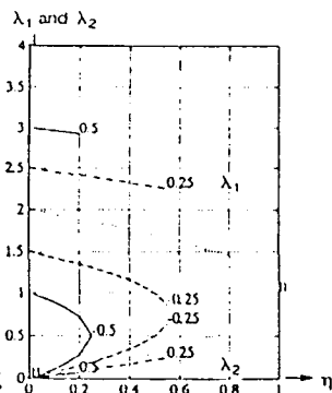
Figure 5. Parabolic slices: \lambda_1 and \lambda_2 vs \eta at \xi = -0.50, -0.25, 0, +0.25, +0.50 for \pi_1/\pi_2 = 0 dB.
