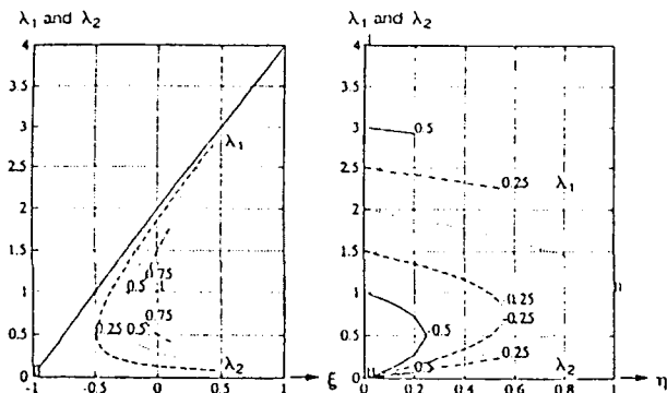
Figure 4. Hyperbolic slices: \lambda_1 and \lambda_2 vs \eta at \xi = 0.0, 0.25, 0.50, 0.75, 1.00 for \pi_1/\pi_2 = 0 dB.
