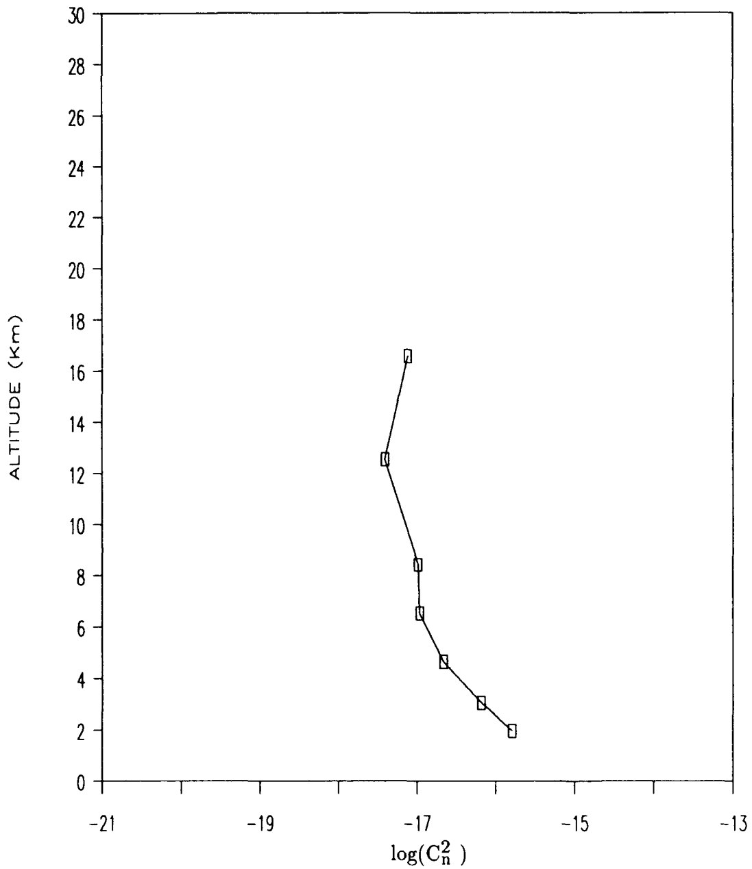
Figure 1. A typical profile obtained using a stellar scintillometer. The units of C_n^2 are m^{-\frac{2}{3}} .
