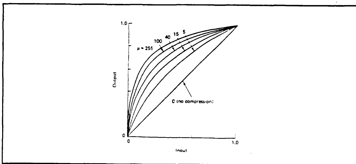
Figure A-2. Companding
