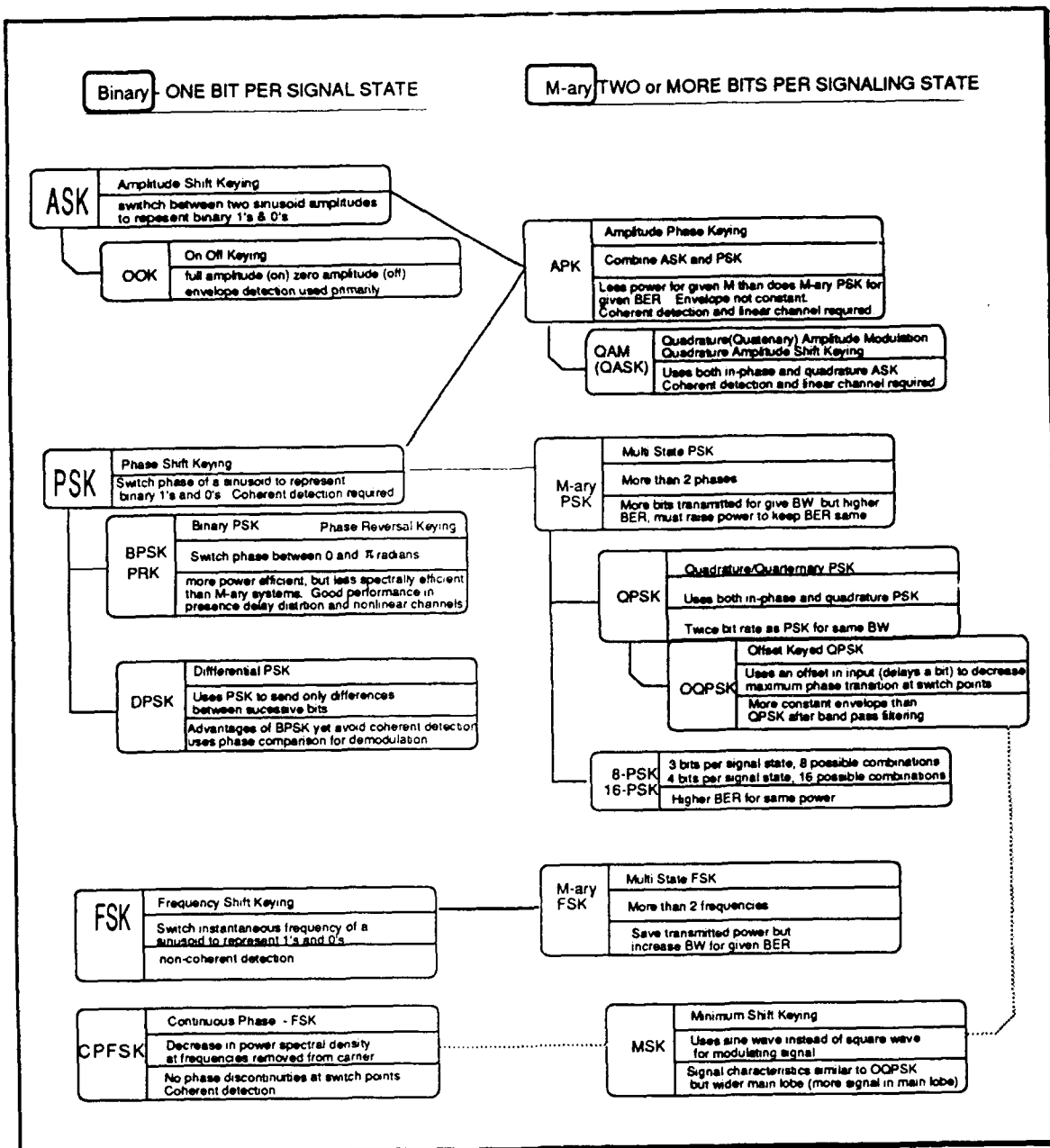
Figure C-1. Modulation Relationship
