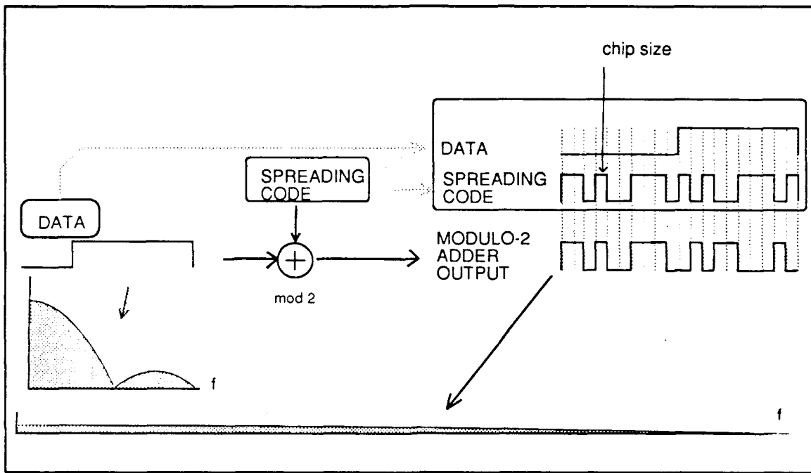
Figure B-1. Direct Sequence Spread Spectrum
