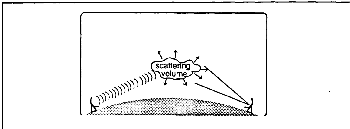
Figure 7-13. Troposcatter
