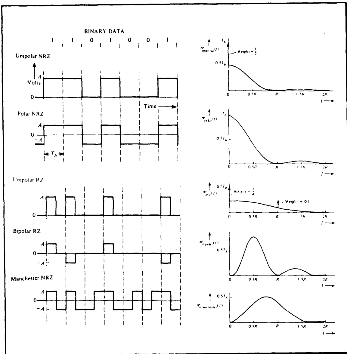
Figure A-3. Line Encoding Formats
