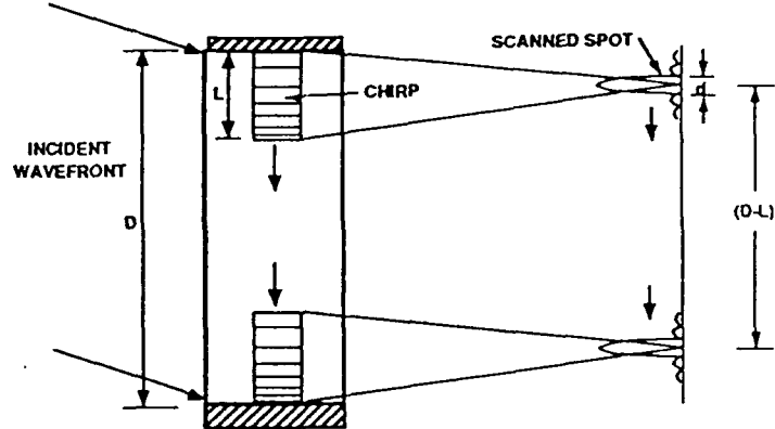
Figure 2 Acoustic Chirp Scanning
