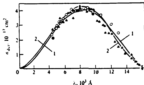
Figure 2-3: Photodetachment cross section of the hydrogen ion (after Smirnov [16] ).
