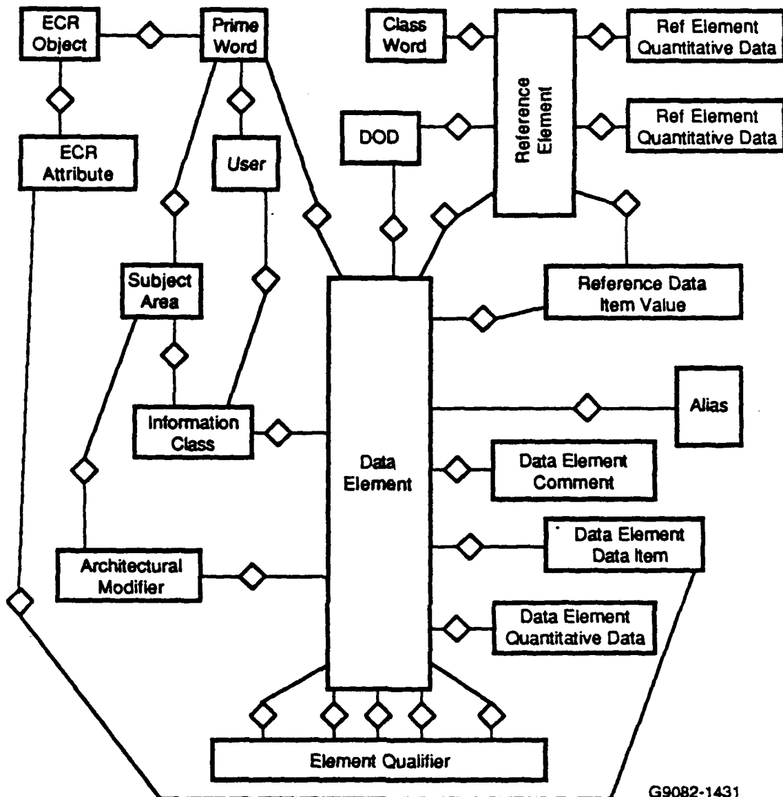
Figure 3-3. Add ER Representation in IRDS
