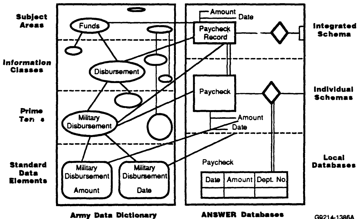
Figure 2-1. Phase I Information Architecture
