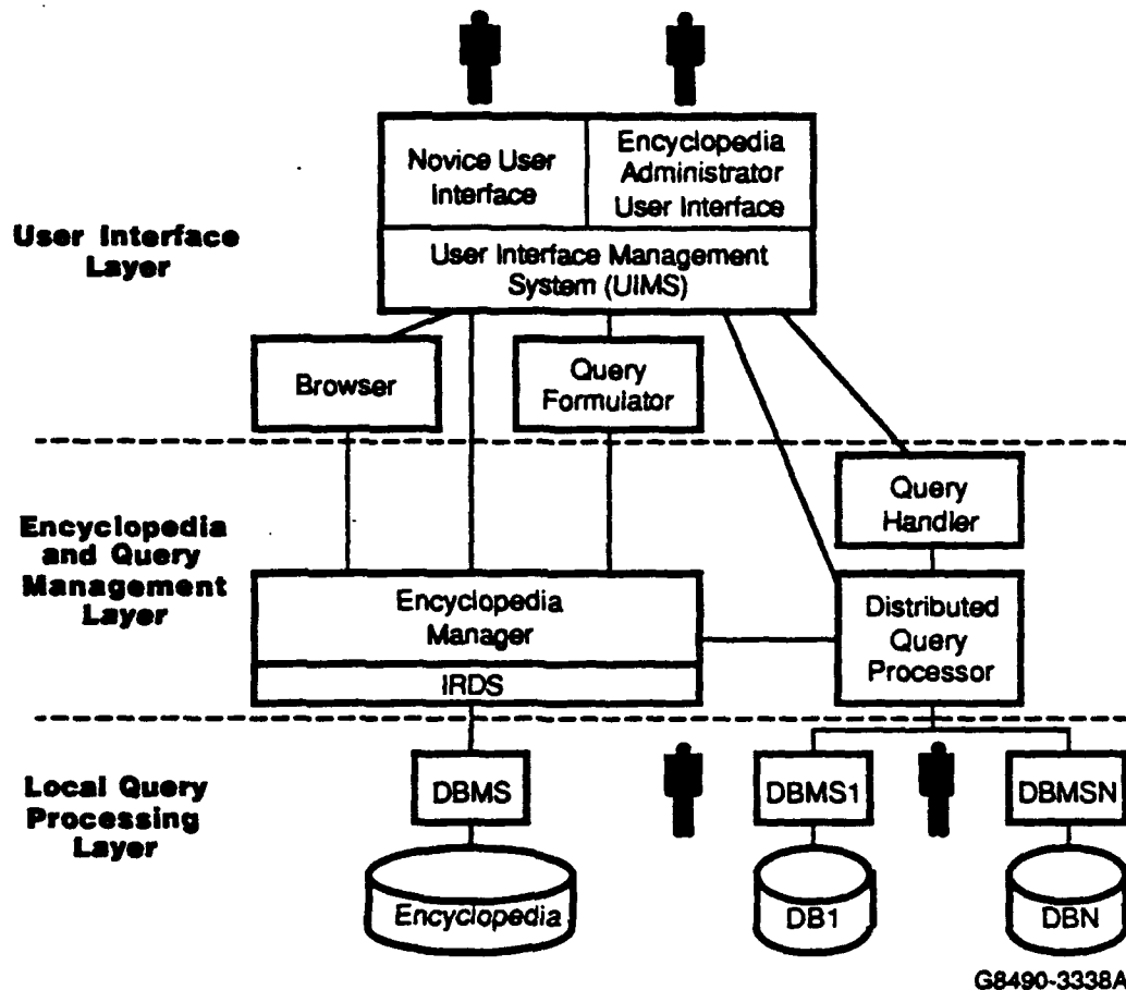
Figure 2-3. Original ANSWER Software Architecture
