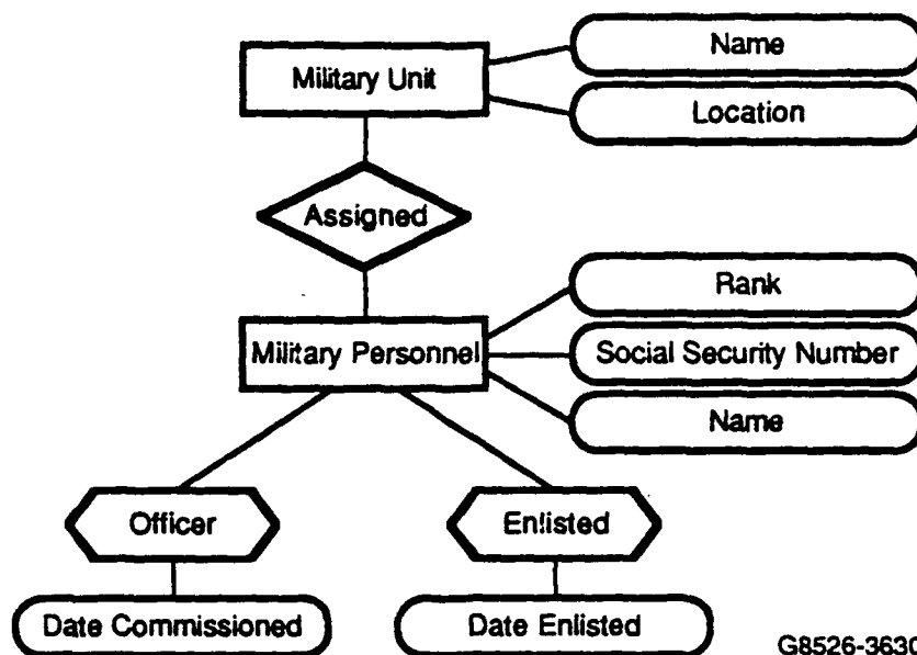
Figure 2-2. Example Entity Type: MILITARY PERSONNEL
