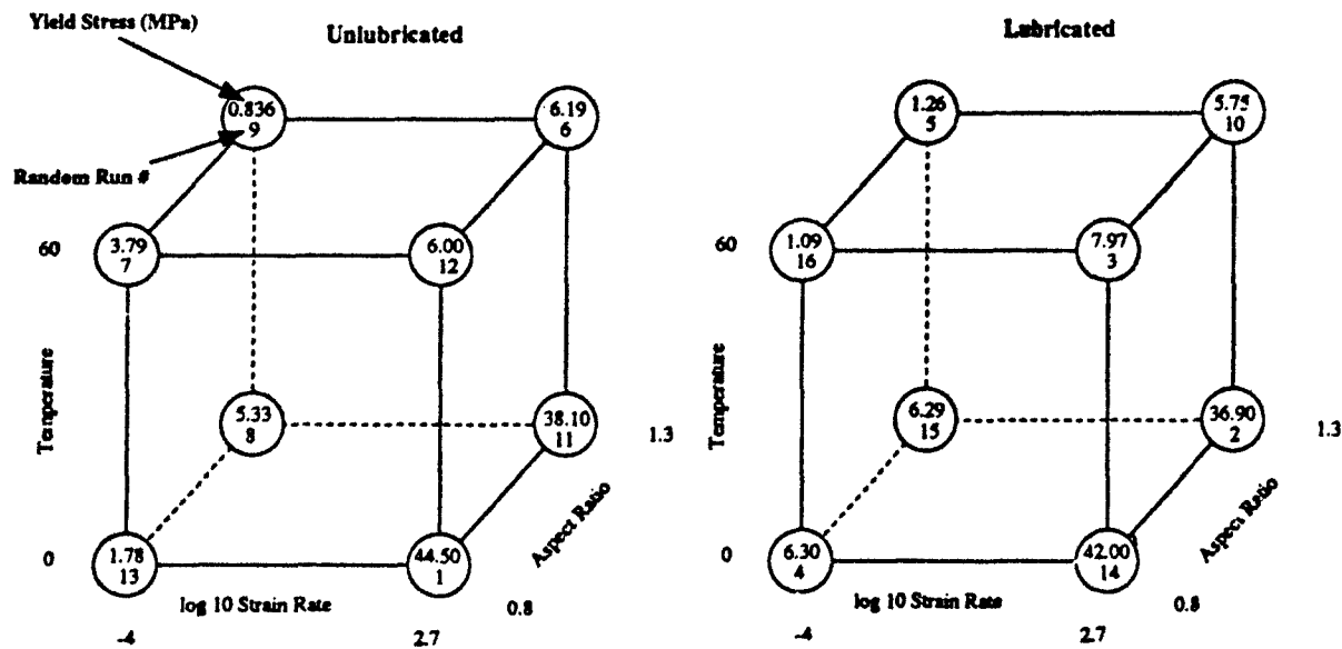
Figure 6. Cube Plots of Stress at Yield Response With and Without Specimen End Lubrication.
