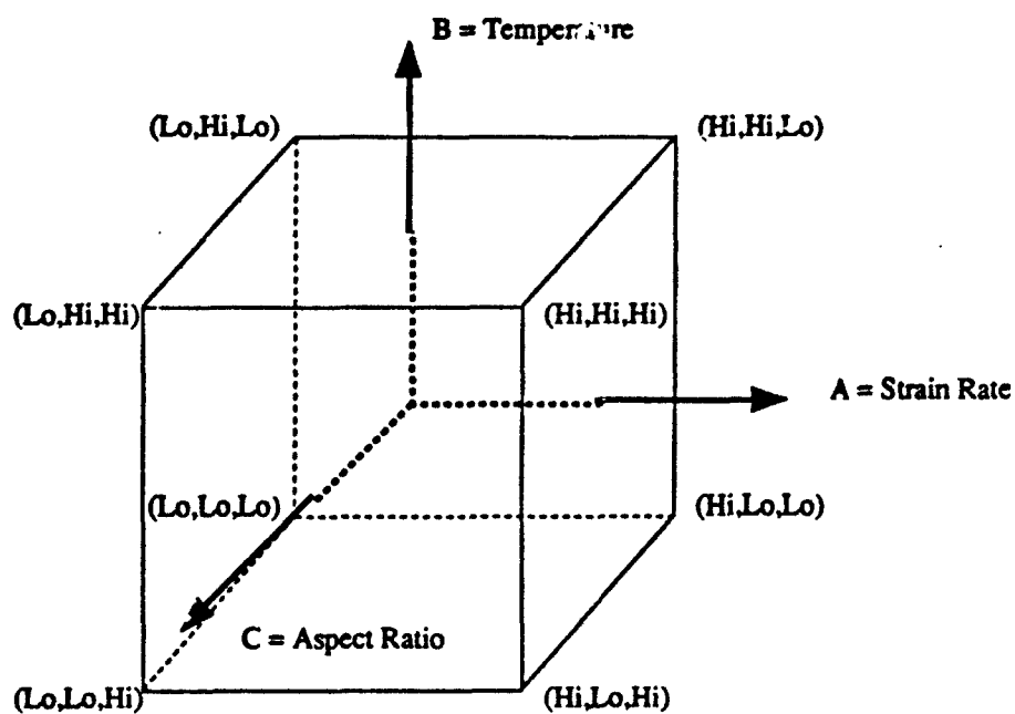
Figure 3. Cube Plot with 2^3 Design Points.
