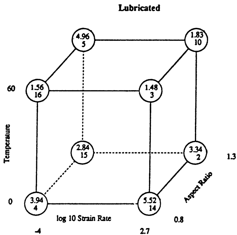
Figure A4. Cube Plots for Strain at Yield.
