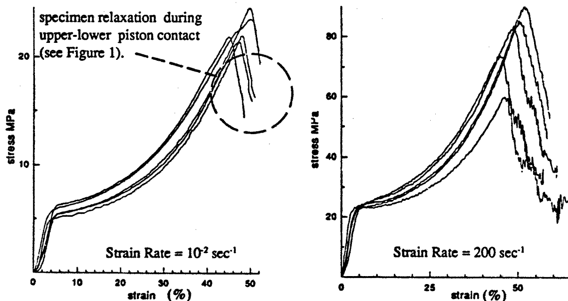
Figure 2. Experimental Reproducibility of the Mechanical Response of JA2 in Uniaxial Compression at Strain Rates of 10^{-2} and 200 \text{ sec}^{-1} .
