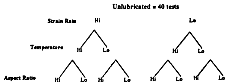
Figure 4. "Classical" Material Test Program for Strain Rate, Temperature, Aspect Ratio, and Specimen End Lubrication.
