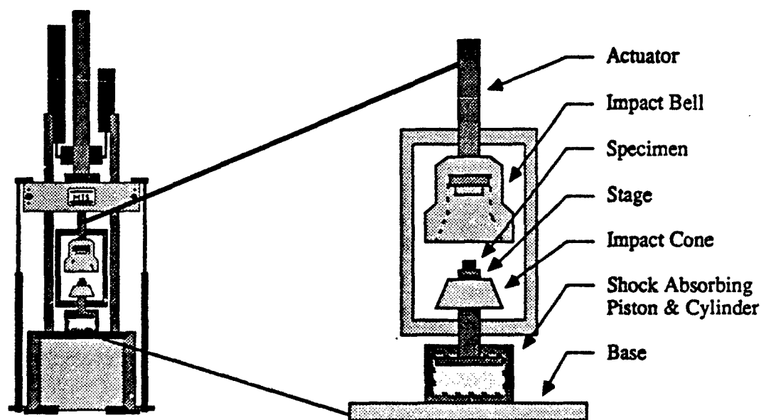
Figure 1. Servohydraulic Test Apparatus with Upper Bell and Impact Cone Piston Assembly.
