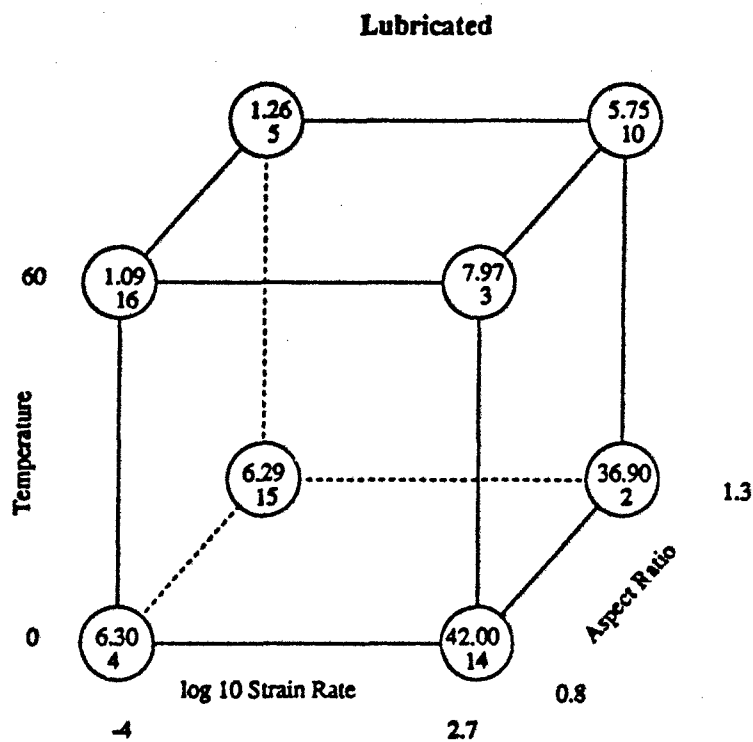
Figure A1. Cube Plots for Stress at Yield
