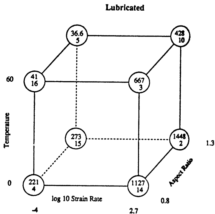
Figure A10. Cube Plots for Modulus.
