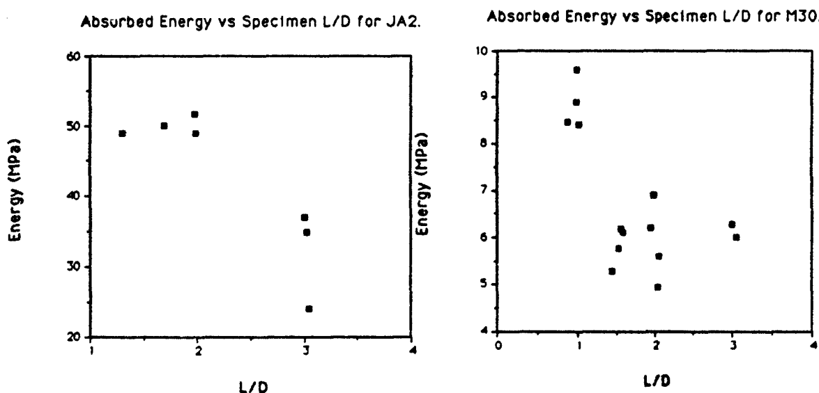
Figure 7. Absorbed Strain Energy Density at Maximum Stress and -30 degrees Celsius for JA2 and M30 Deformed at 100 sec -1 in Uniaxial Compression versus Specimen Aspect Ratio.
