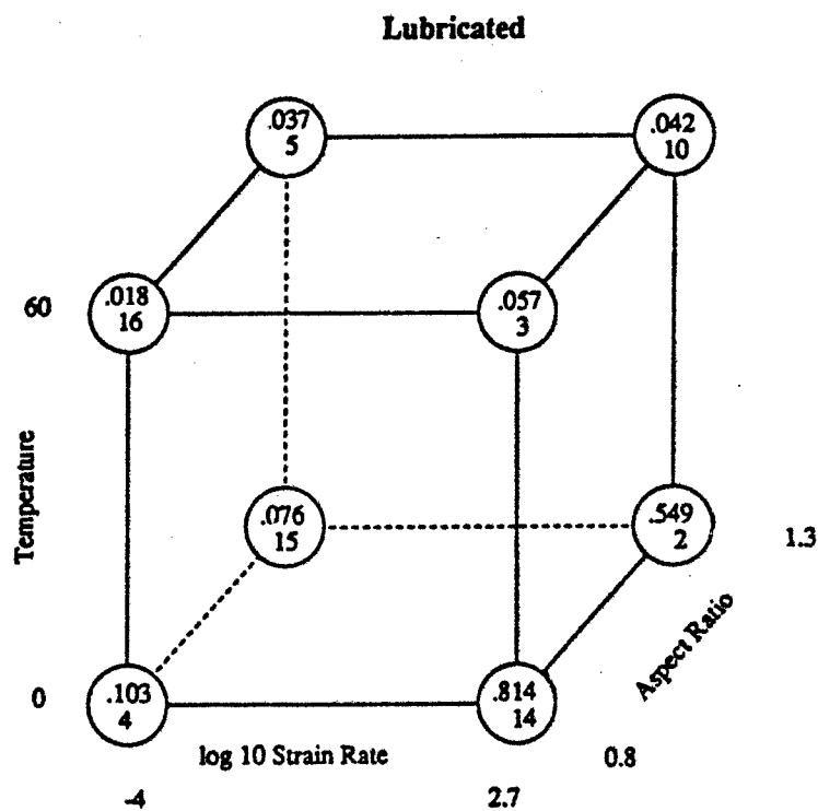
Figure A7. Cube Plots for Energy.
