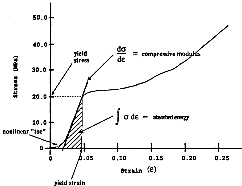
Figure 5. Measured Mechanical Responses.
