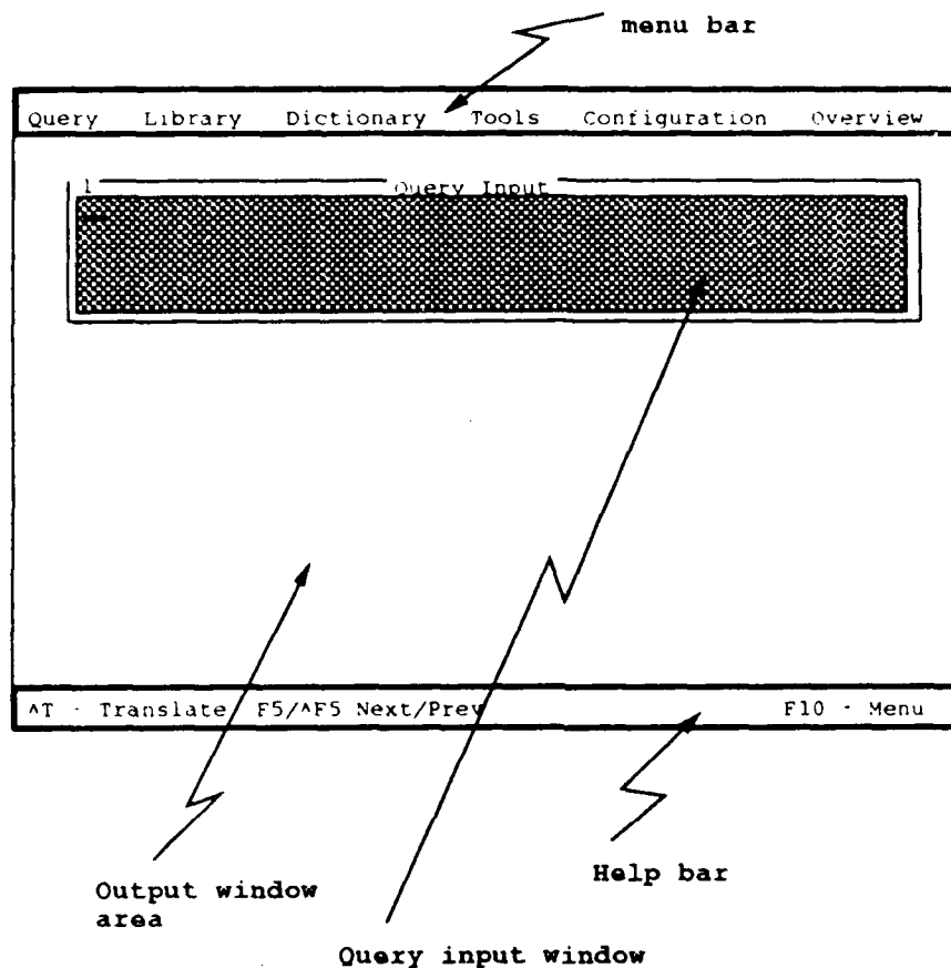
Figure 6. The Expert-MCA interface.
