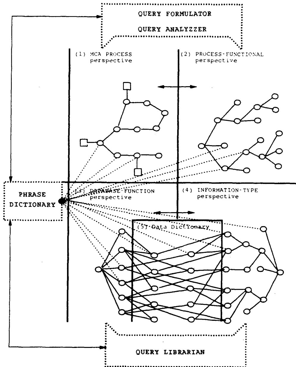
Figure 7. The organization of Expert-MCA knowledge.
