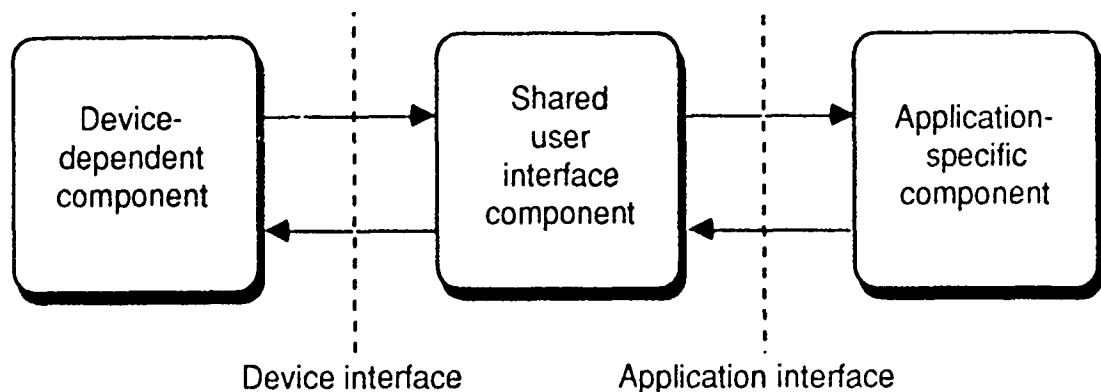
Figure 2-1: A Basic Structural Model for User Interface Software
