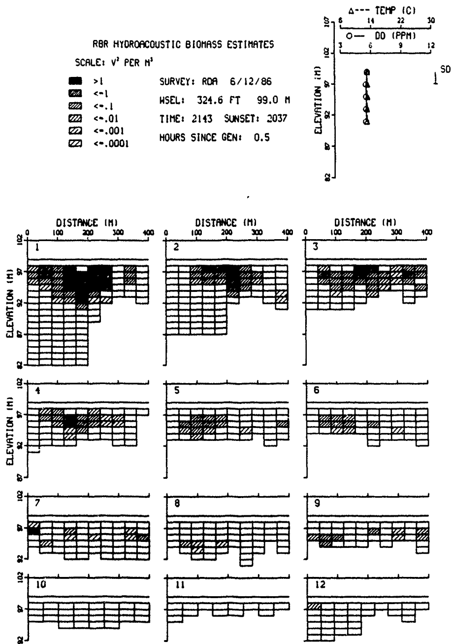
Figure 35. Distribution of relative fish biomass on 12 June 1986 at night immediately after generation. (Refer to Figure 28 for explanation of data)
