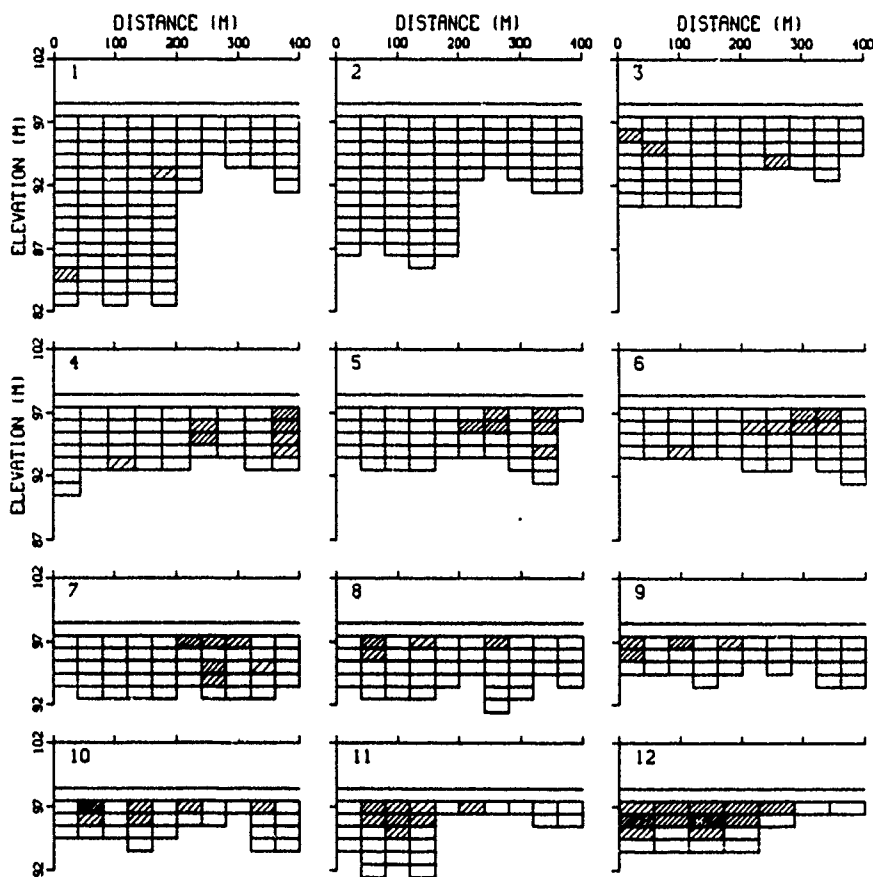
Figure 36. Distribution of relative fish biomass on 16 July 1986 at dusk immediately after generation. (Refer to Figure 28 for explanation of data)
