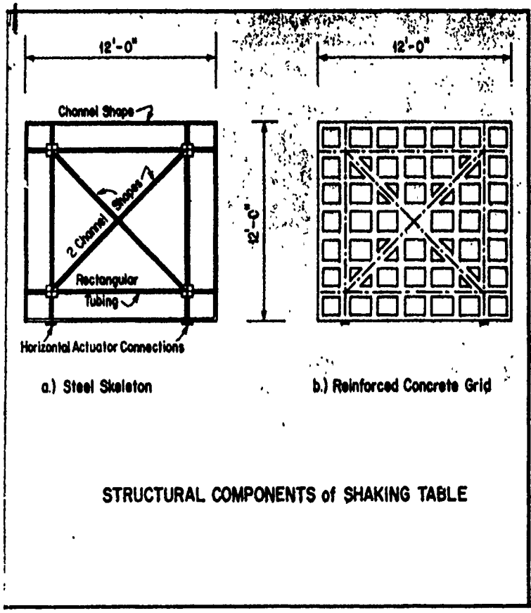
Figure E4. Structural components of shake table.
