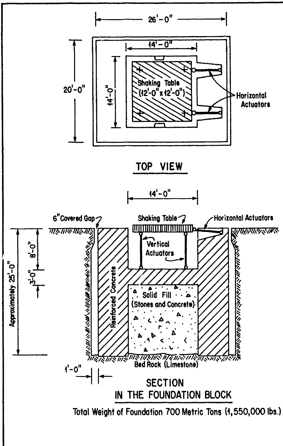
Figure E3. Section in the foundation block.
