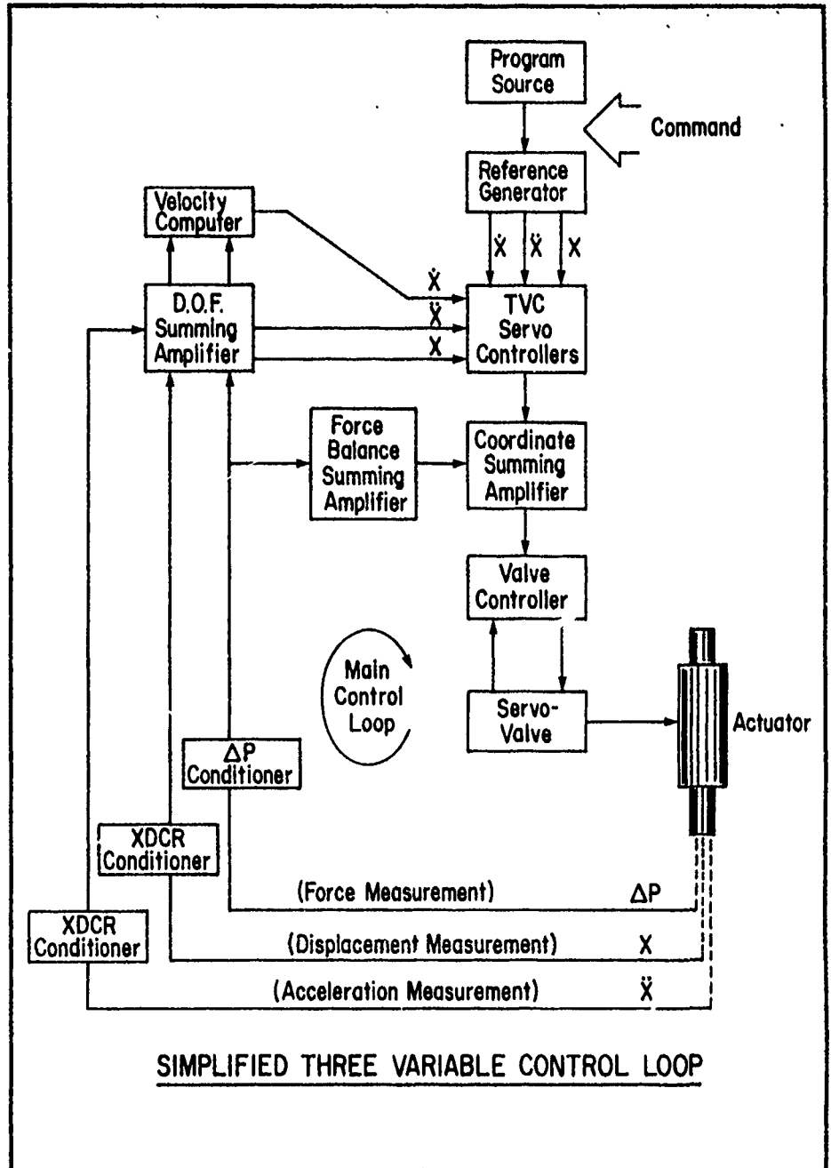
Figure E7. Simplified three-variable control loop.
