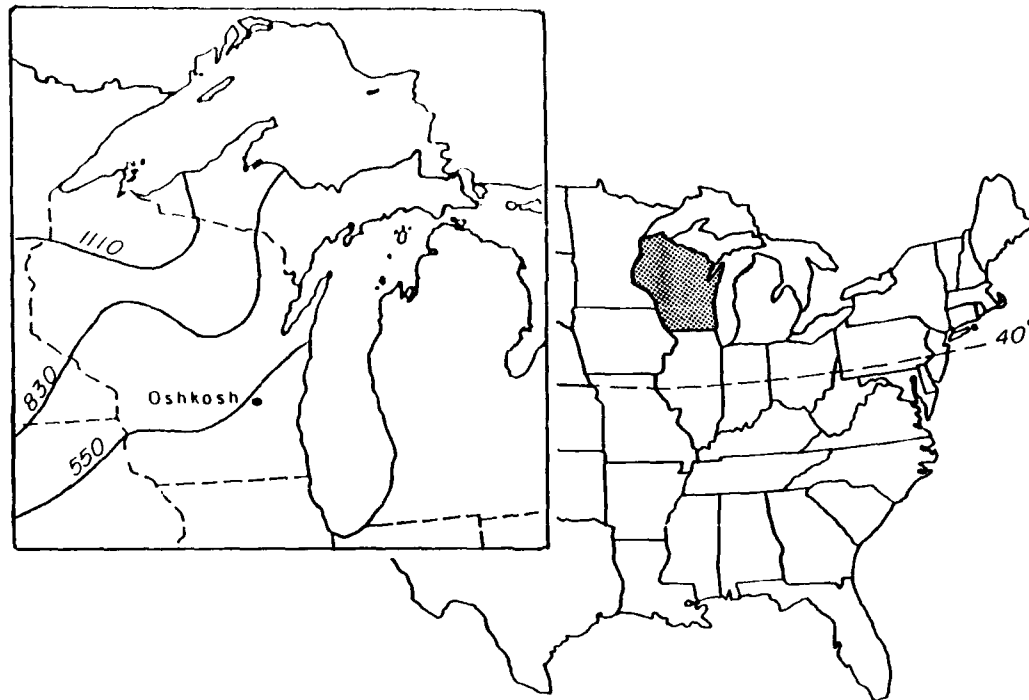
Figure 1. Location of Wittman Field (isolines show mean air freezing index [ ^{\circ}\text{C-days} ]).
