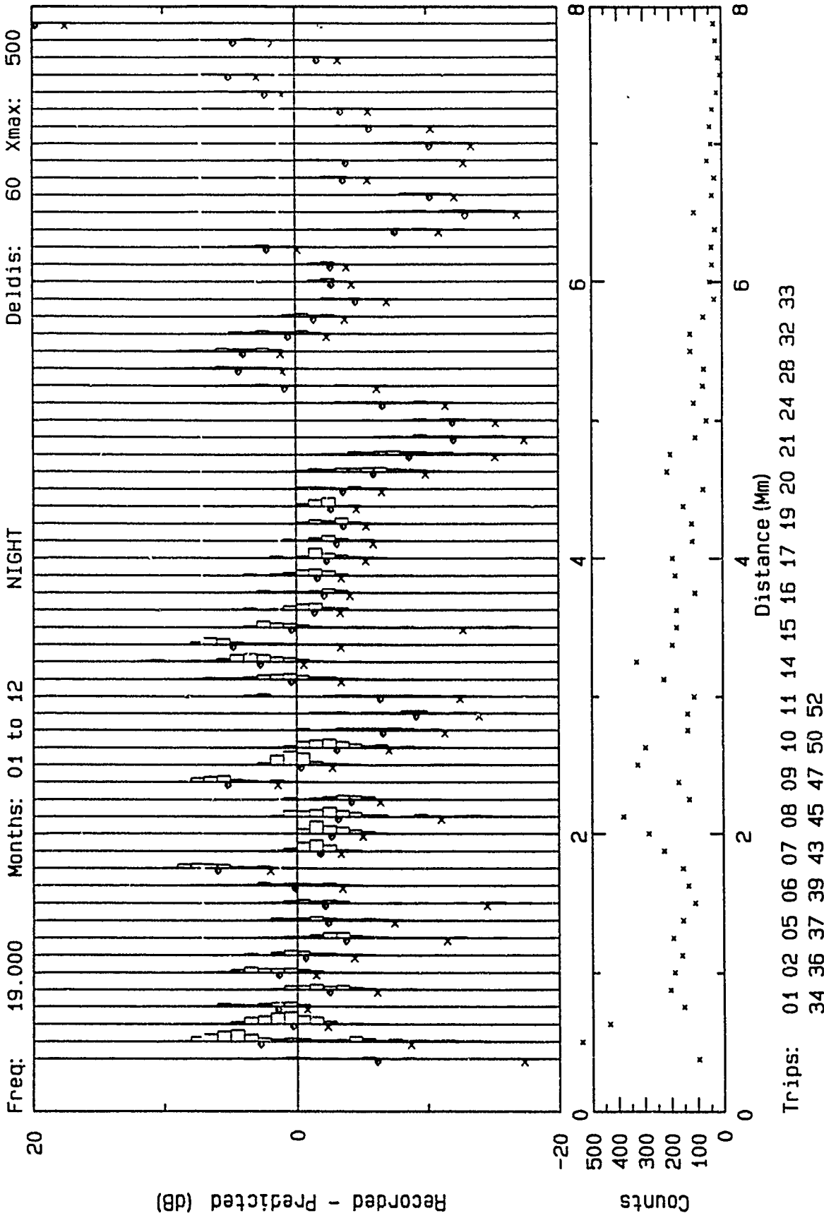
Figure 48. Recorded - predicted data, Anthorne at 80 kW, 19.0 kHz, with LWPC prediction for \beta = 0.49 , h' = 87 , PCAP = 70-74.
