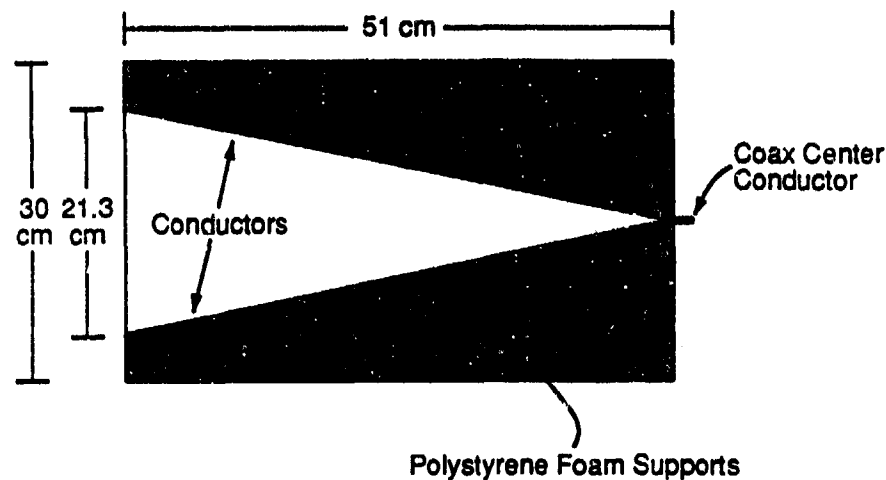
Figure 8. Schematic of TEM Horn Antenna
