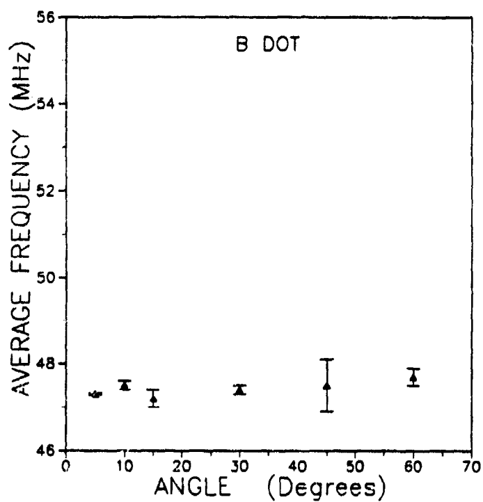
Figure 45. Average Frequency of Spectrum for Full Current B Dot
