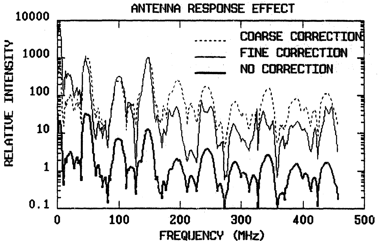
Figure 15. Comparison of Correction Values
