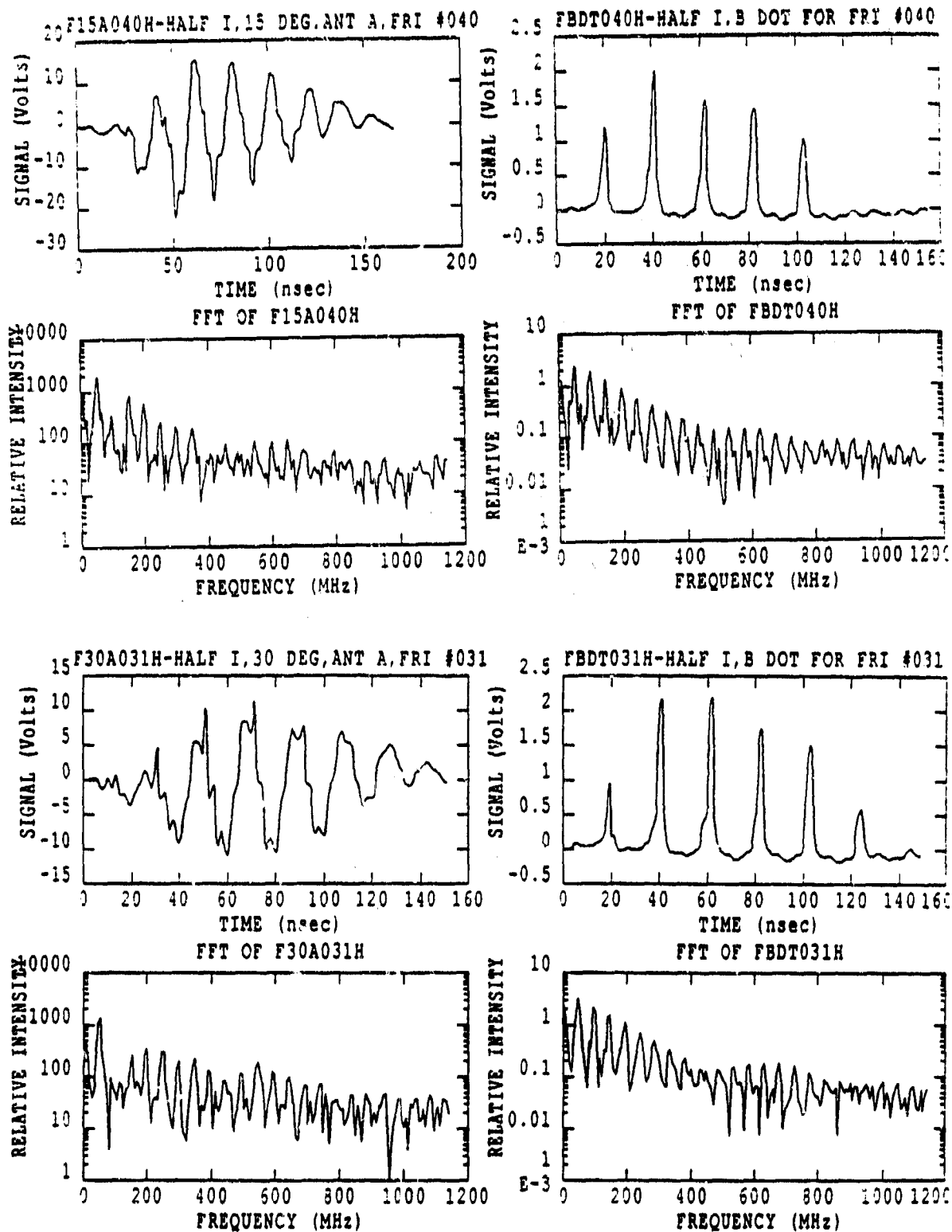
Figure 30. Signal and Spectrum for Half Energy, Half Current, Angles of 15 and 30 Degrees
