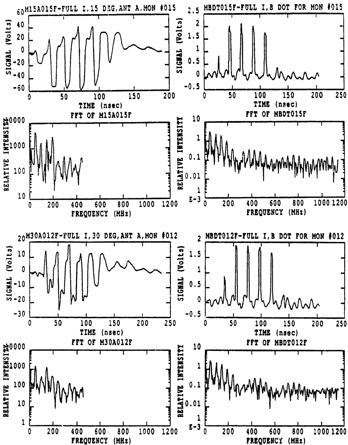
Figure 21. Signal and Spectrum for Full Current, Full Energy, Angles of 15 and 30 Degrees
