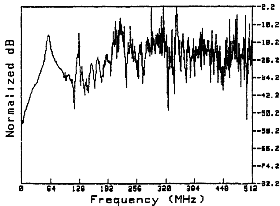
Figure 14. Antenna Response
