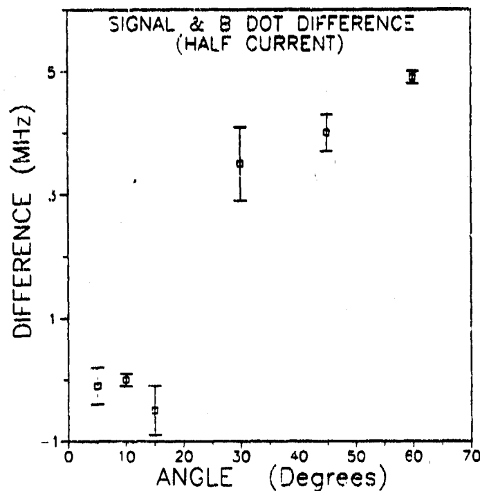
Figure 48. Signal and B Dot Difference for Half Current
