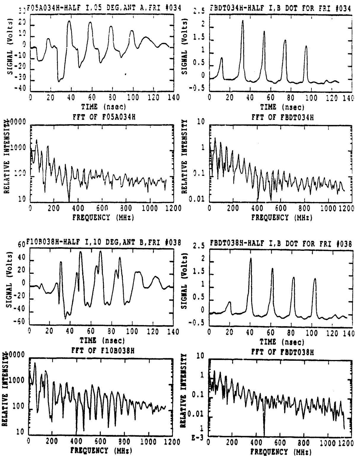
Figure 29. Signal and Spectrum for Half Energy, Half Current, Angles of 5 and 10 Degrees
