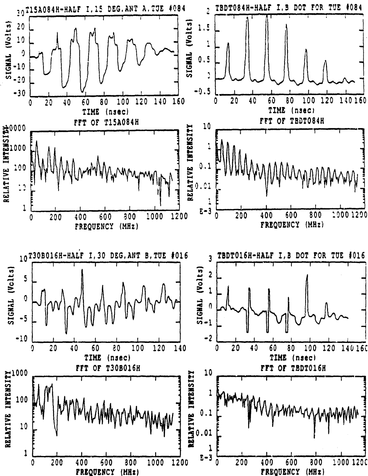
Figure 24. Signal and Spectrum for Half Current, Full Energy. Angles of 15 and 30 Degrees
