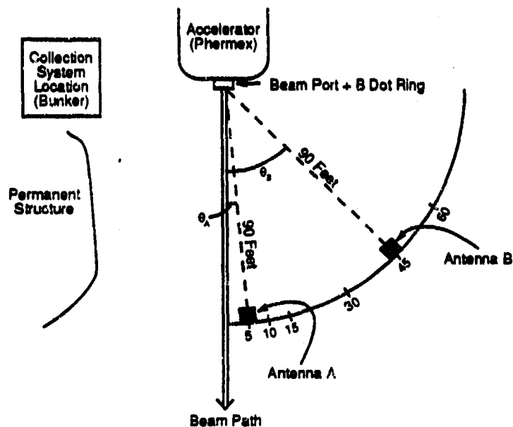
Figure 10. Antenna Placement
