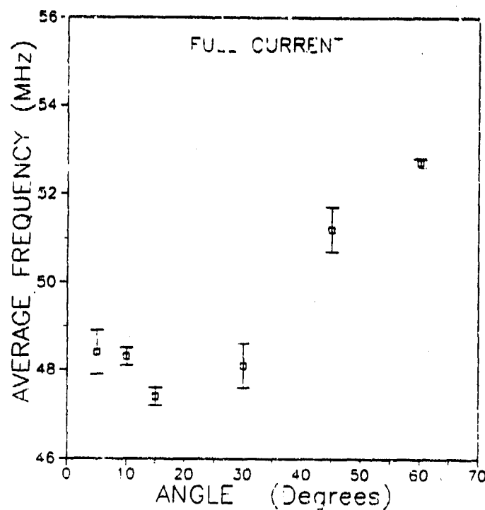
Figure 43. Average Frequency of Spectrum for Full Current
