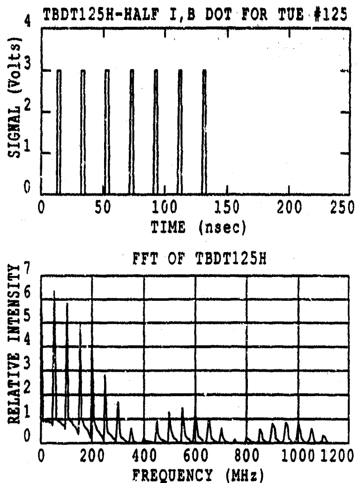
Figure 49. Modulation Example from a Perfectly Pulsing Accelerator
