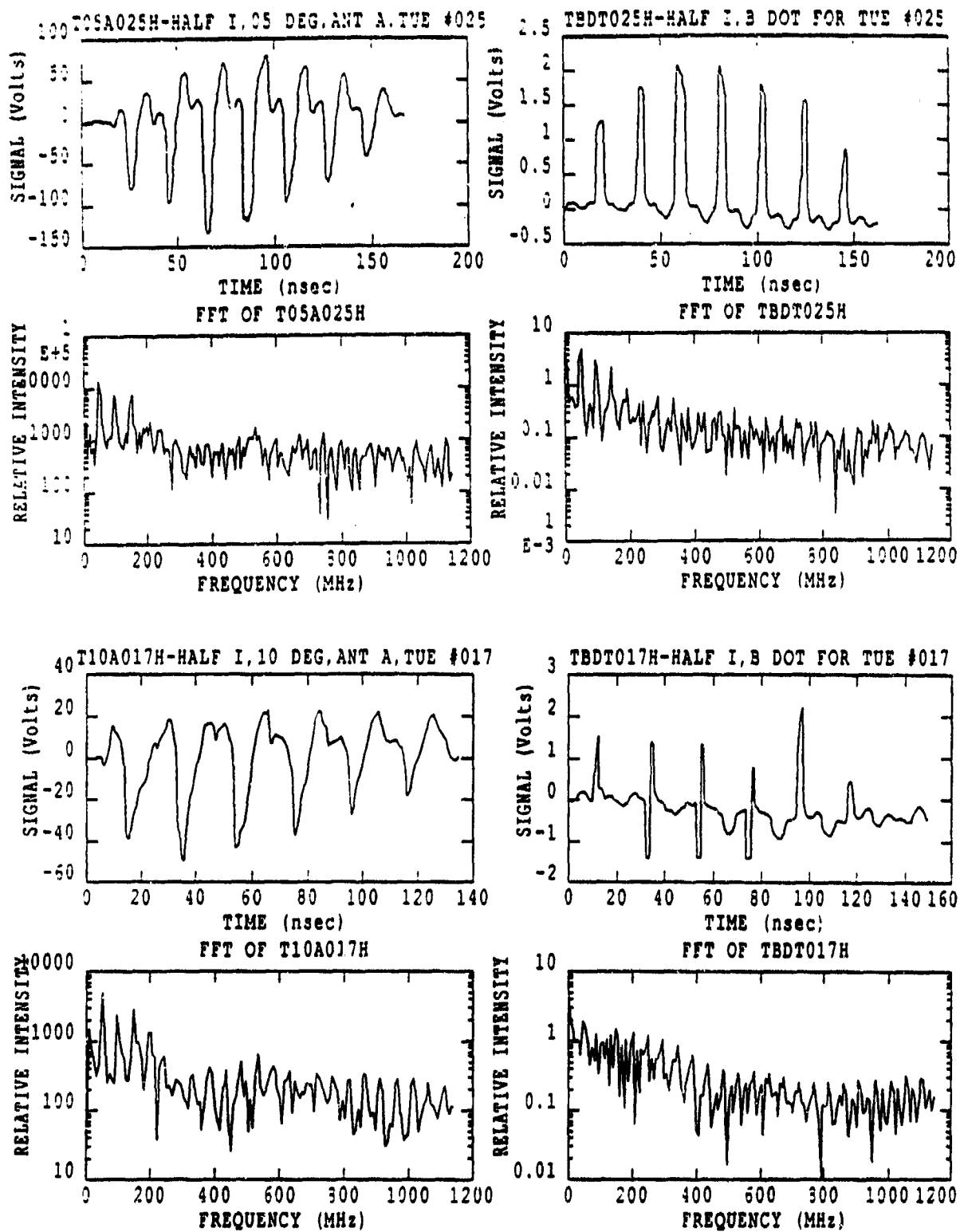
Figure 23. Signal and Spectrum for Half Current, Full Energy, Angles of 5 and 10 Degrees
