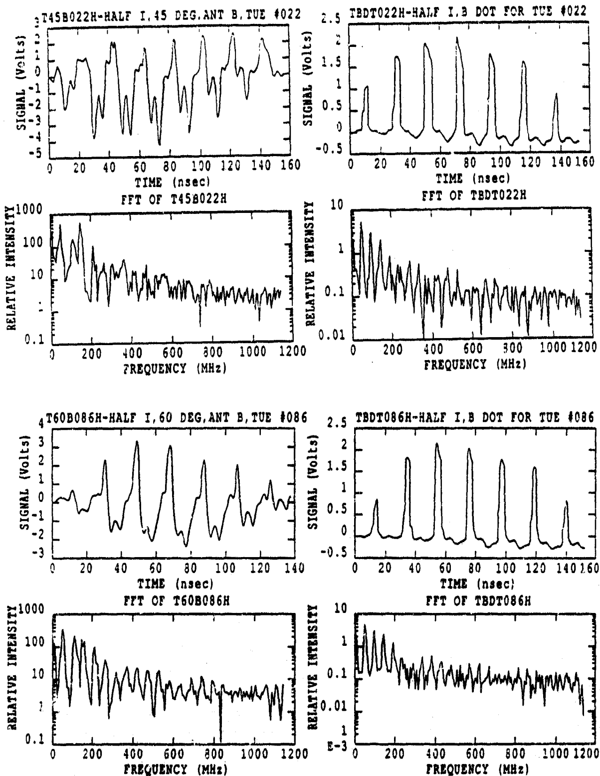
Figure 25. Signal and Spectrum for Half Current, Full Energy, Angles of 45 and 60 Degrees
