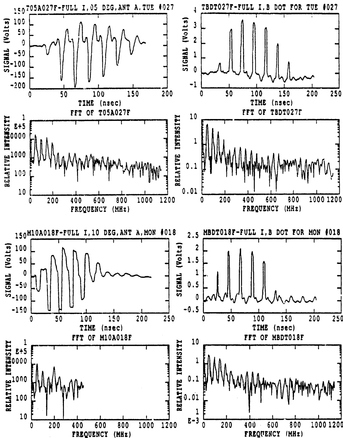
Figure 20. Signal and Spectrum for Full Current, Full Energy. Angles of 5 and 10 Degrees
