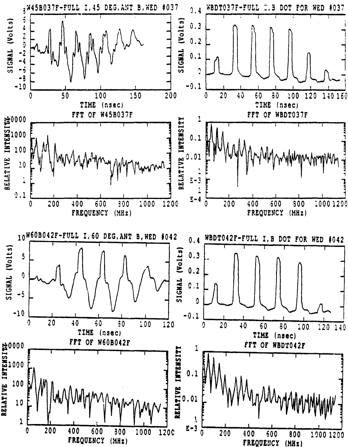
Figure 28. Signal and Spectrum for Diffuse Beam, Full Current, Full Energy, Angles of 45 and 60 Degrees
