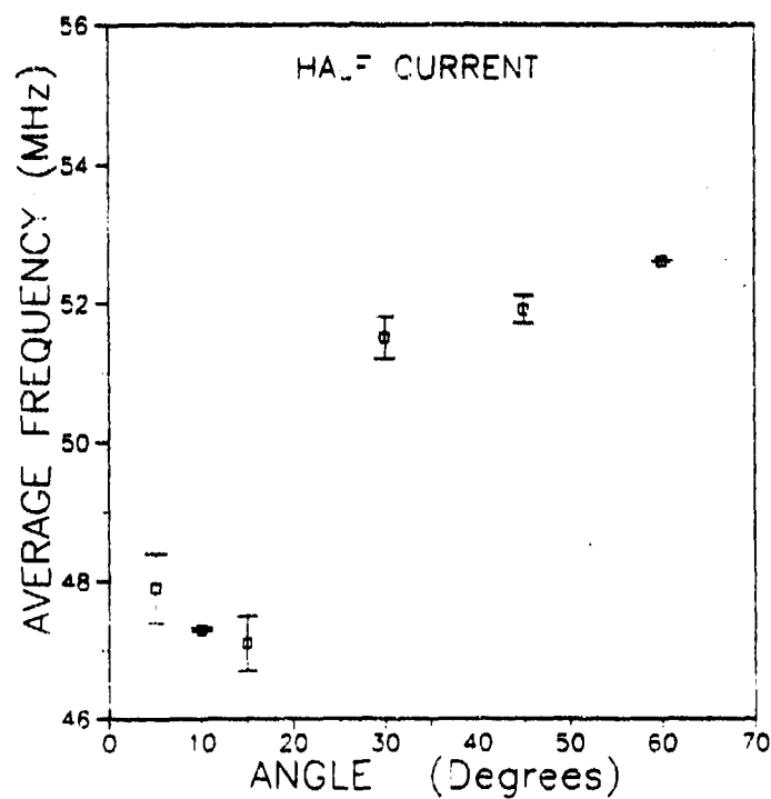
Figure 44. Average Frequency of Spectrum for Half Current
