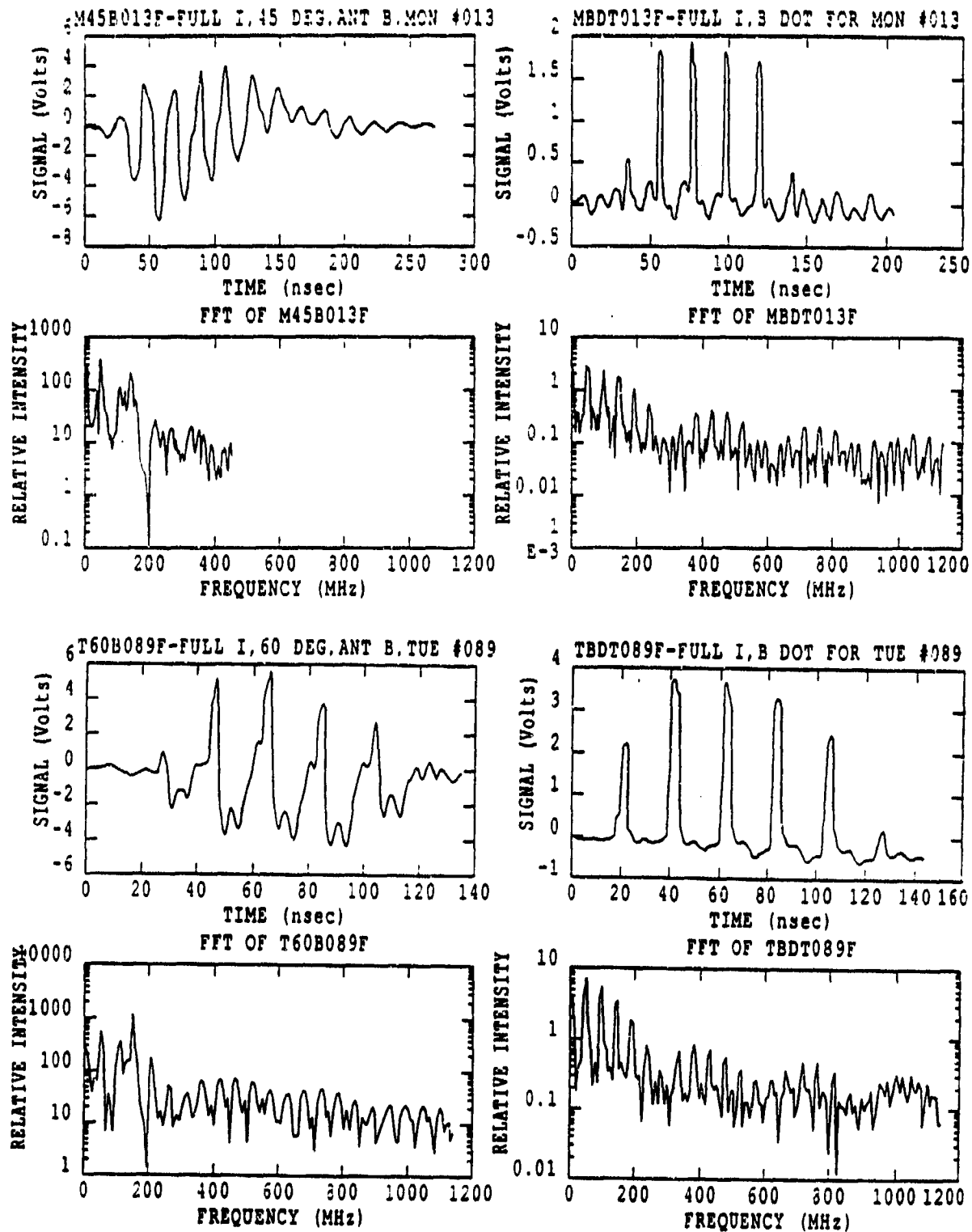
Figure 22. Signal and Spectrum for Full Current, Full Energy, Angles of 45 and 60 Degrees
