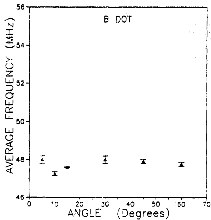
Figure 46. Average Frequency of Spectrum for Half Current B Dot
