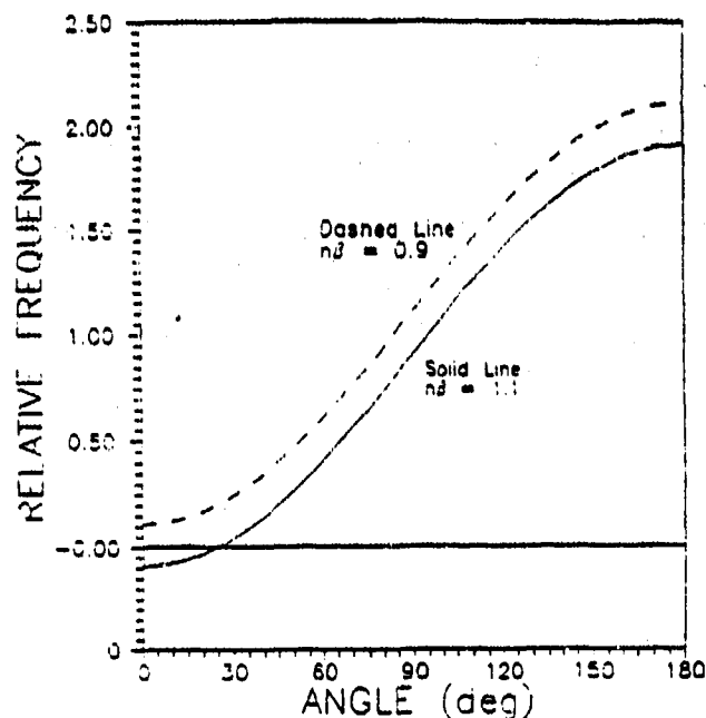
Figure 2. Frequency Shifting with Angle
