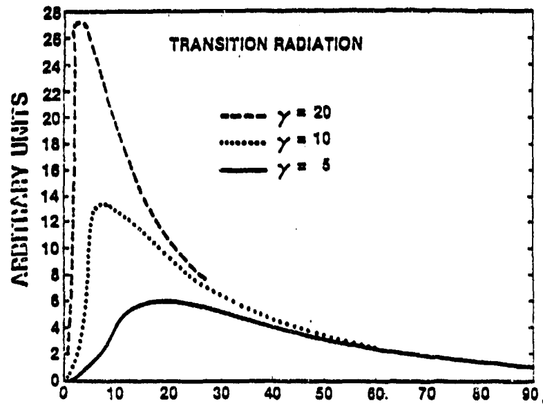
Figure 3. Transition Energy Emitted per Unit Angle
