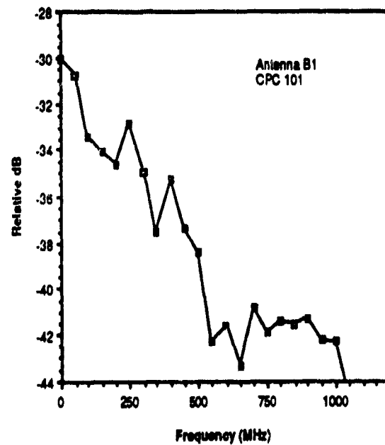
Figure 16. Antenna A & B1 Transfer Functions
