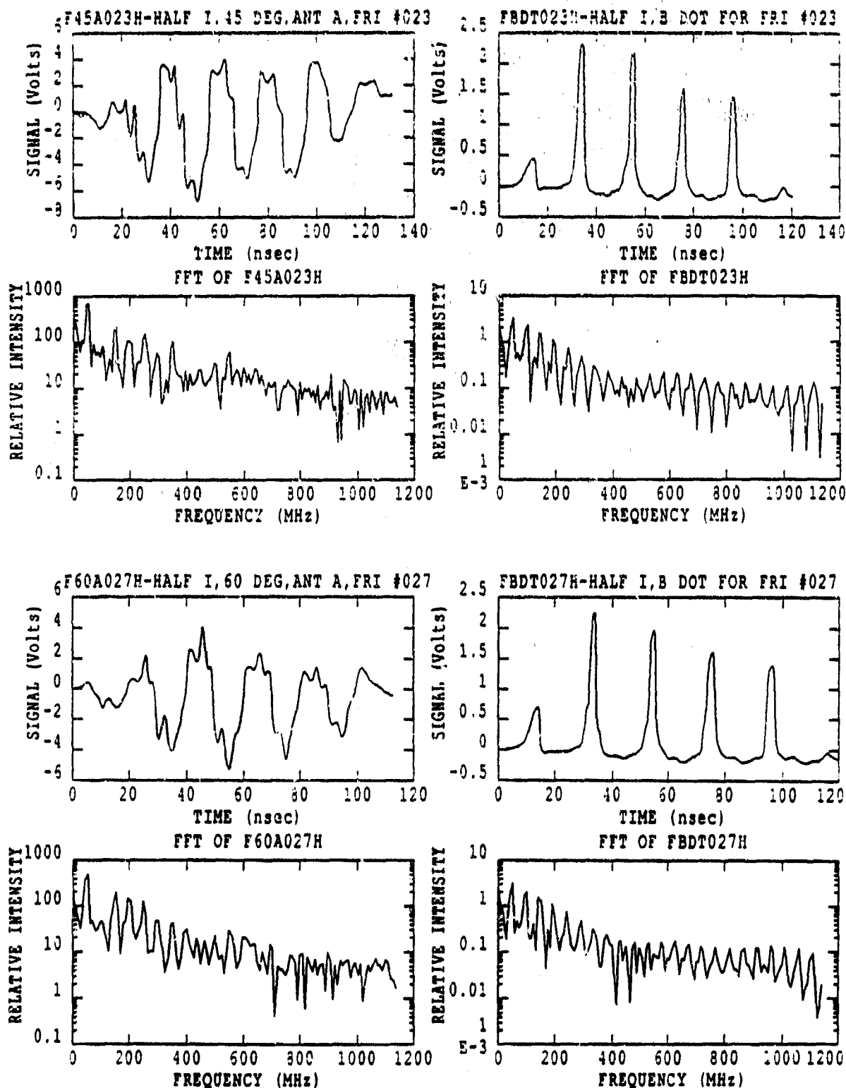
Figure 31. Signal and Spectrum for Half Energy, Half Current, Angles of 45 and 60 Degrees
