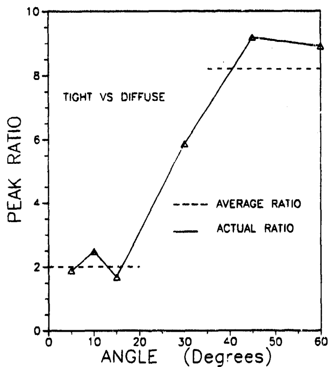
Figure 36. Ratio of Tight to Diffuse Beam Signals
