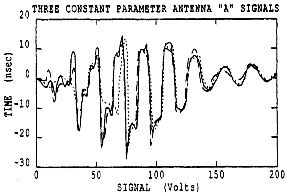
Figure 17. Reproducible Signals from Antenna A
