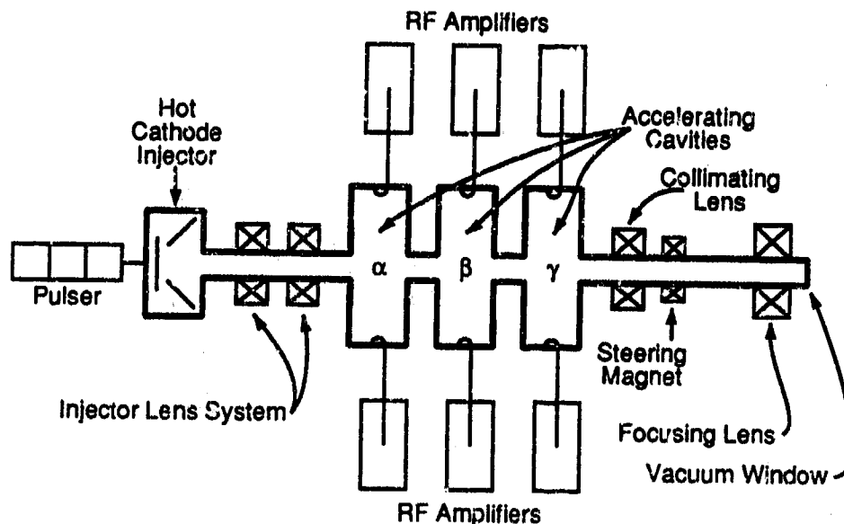
Figure 7. Schematic of Phermex Accelerator
