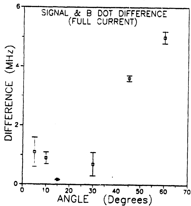
Figure 47. Signal and B Dot Difference for Full Current
