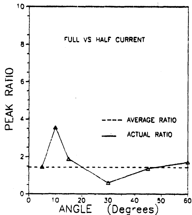
Figure 35. Ratio of Full to Half Current Signals
