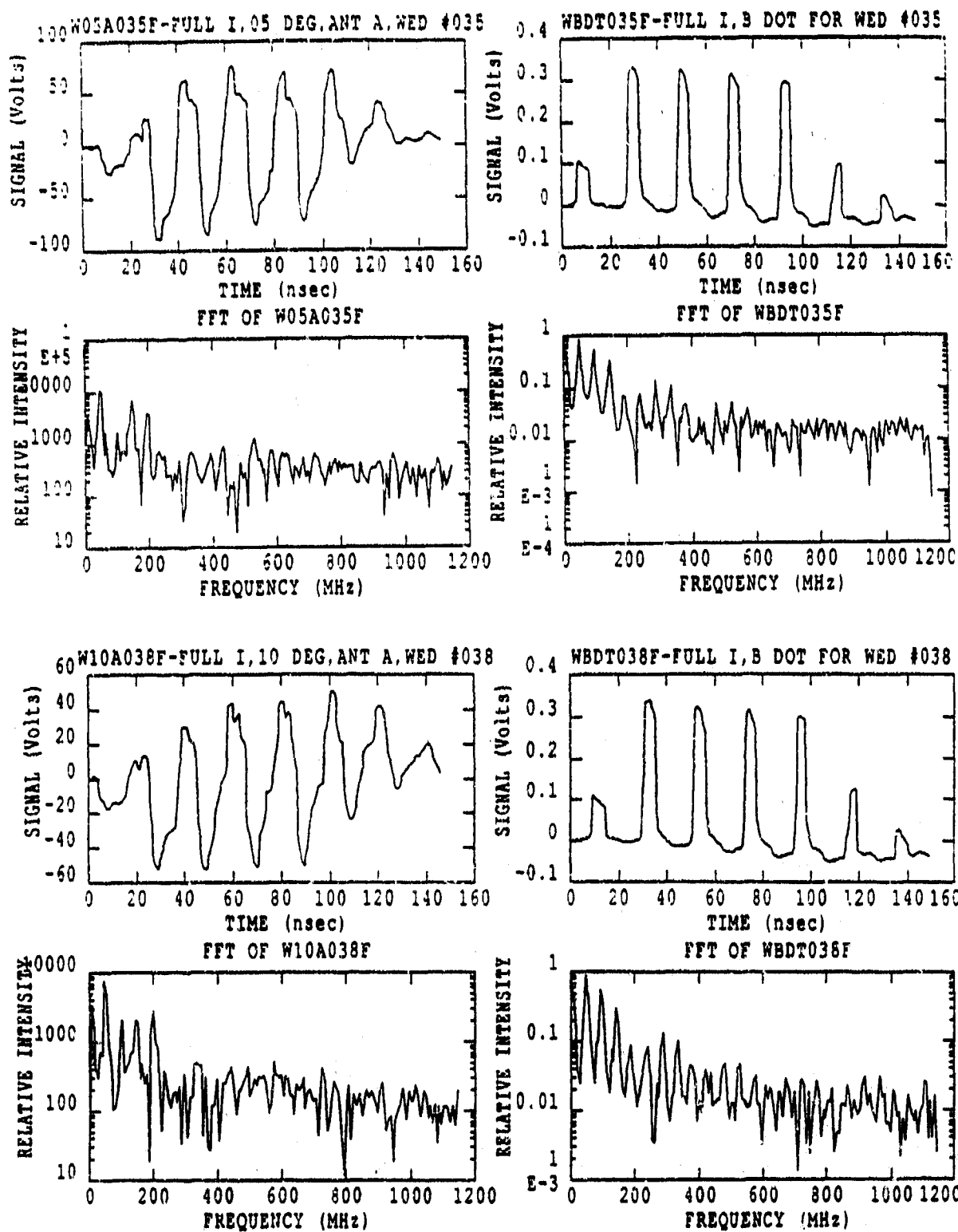
Figure 26. Signal and Spectrum for Diffuse Beam, Full Current, Full Energy, Angles of 5 and 10 Degrees
