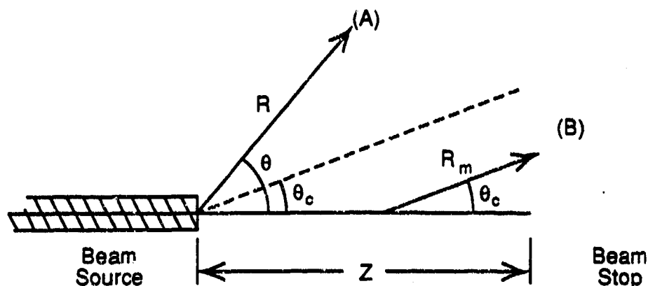
Figure 4. Radiation Areas with a Finite Beam
