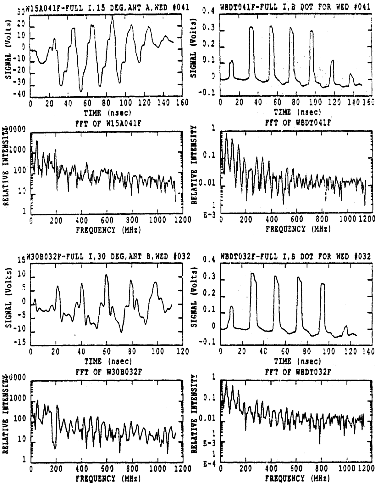
Figure 27. Signal and Spectrum for Diffuse Beam, Full Current, Full Energy, Angles of 15 and 30 Degrees
