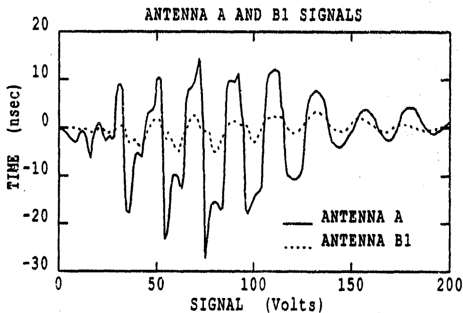
Figure 19. Comparison of Antenna A and B1 Signals
