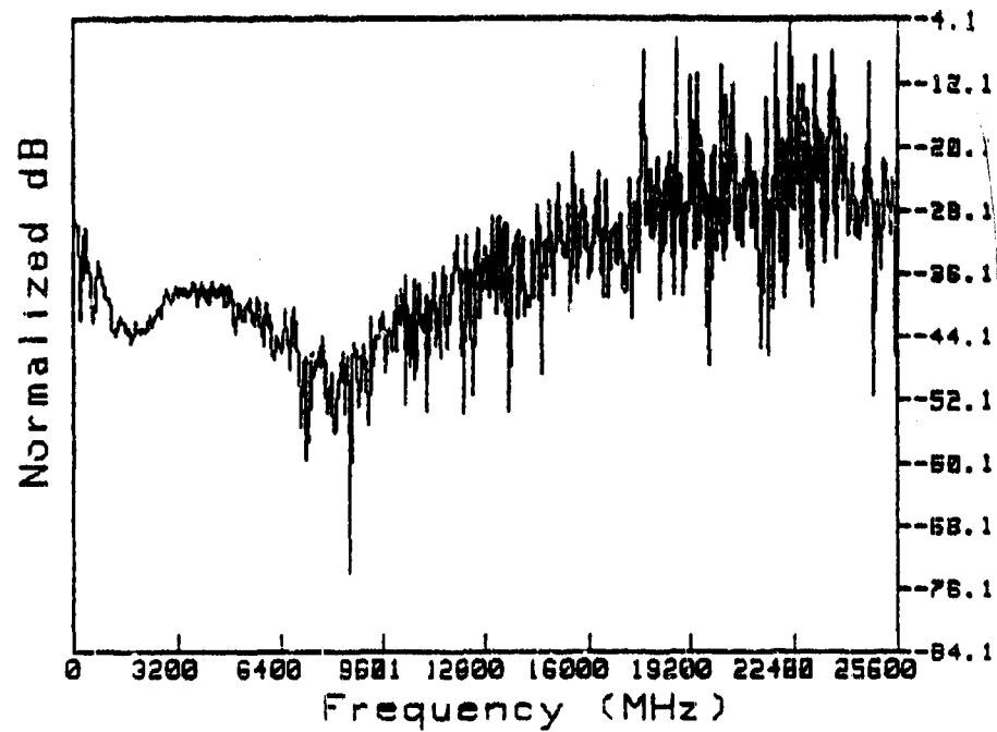
Figure 13. Antenna Response
