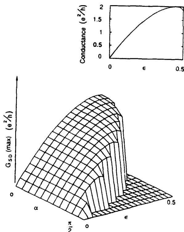
FIG. 4. The maximum source-to-drain conductance G_{SD}(\max) (or the "on" conductance of the transistor as a function of \epsilon , the transmission probability from the source to either the gate or the drain, and \alpha , the phase of the internal reflection within the gate or the drain arm. The inset shows G_{SD}(\max) as a function of \epsilon for \alpha = \pi . The plateau region in this plot corresponds to those values of \alpha and \epsilon that are forbidden by the condition in Eq. (5). This plot is symmetric about the \alpha = \pi/2 plane.
