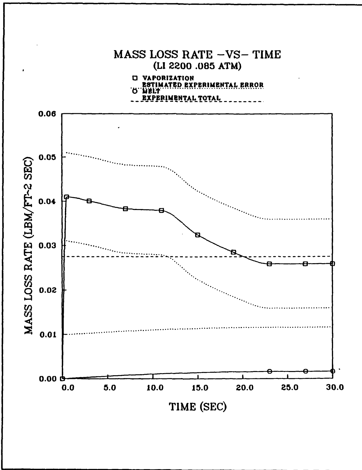
Figure 30 LI 2200 Mass Loss Rate .085 Atmospheres
