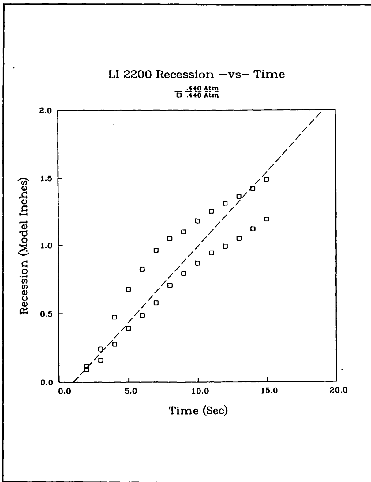
Figure 26 LI 2200 Recession .440 Atmospheres
