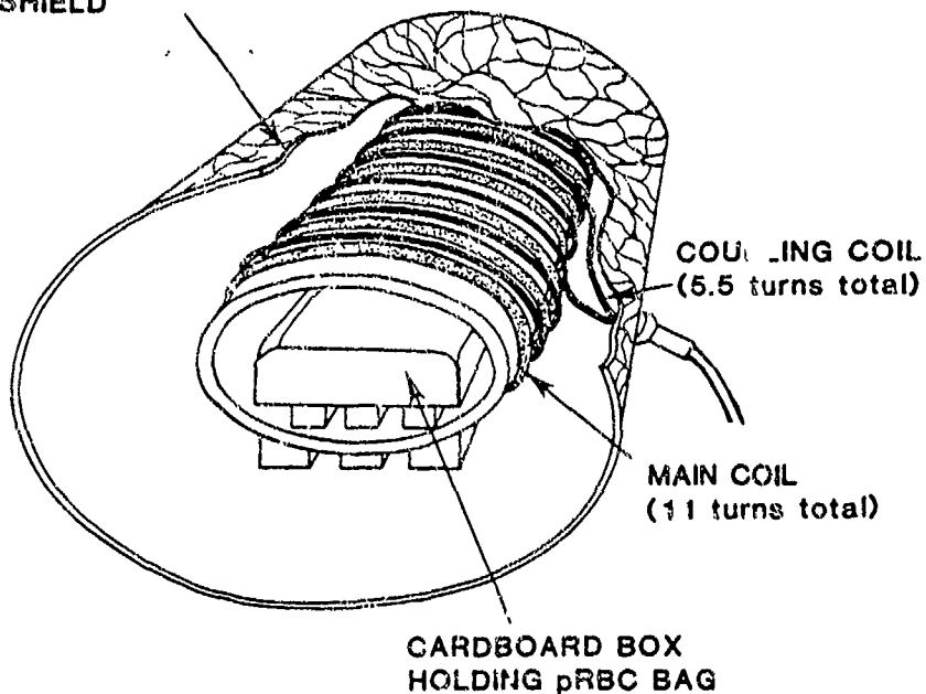
Figure 1. Diagram of the RF coil system.
