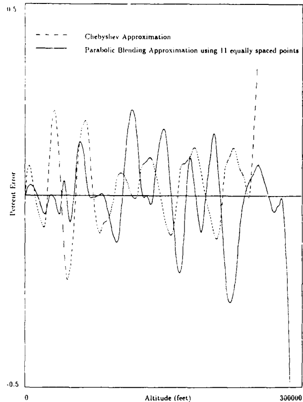
Fig. 2 Pressure error vs altitude (parabolic blending approximation using 11 equally spaced points).
