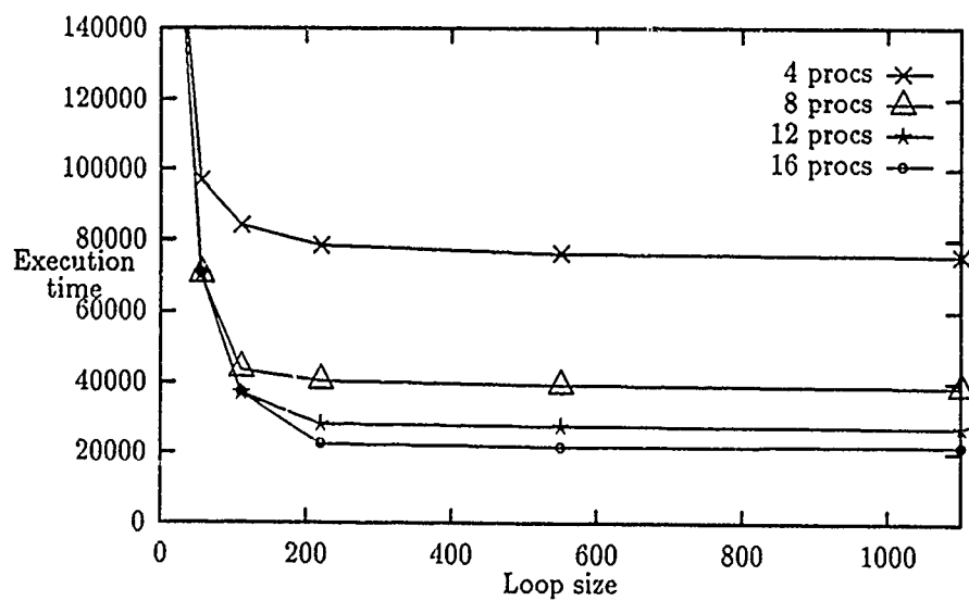
Figure 14: Execution time vs. granularity for synchronization bus
