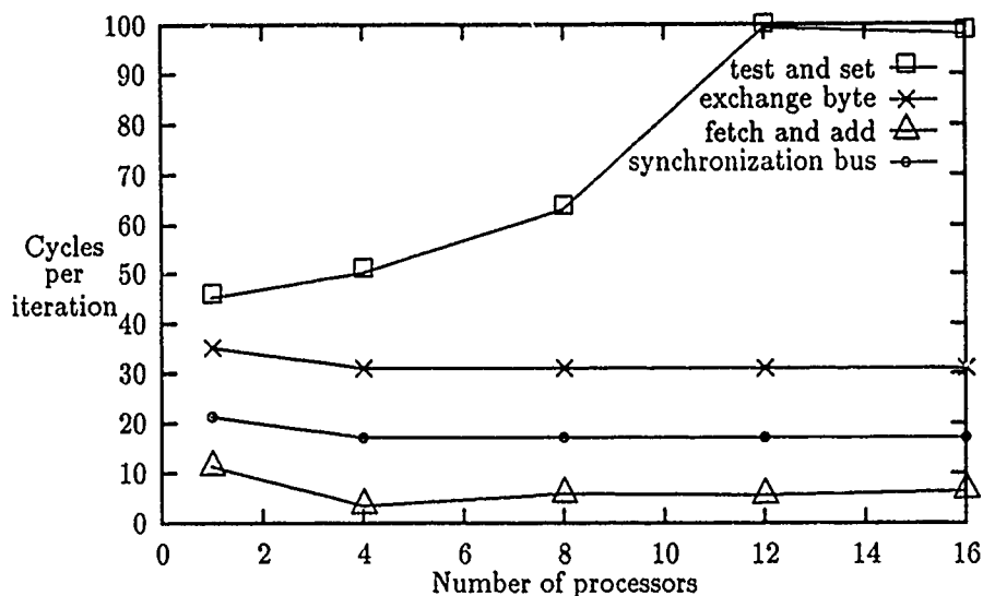
Figure 20: Loop scheduling overhead vs. number of processors
