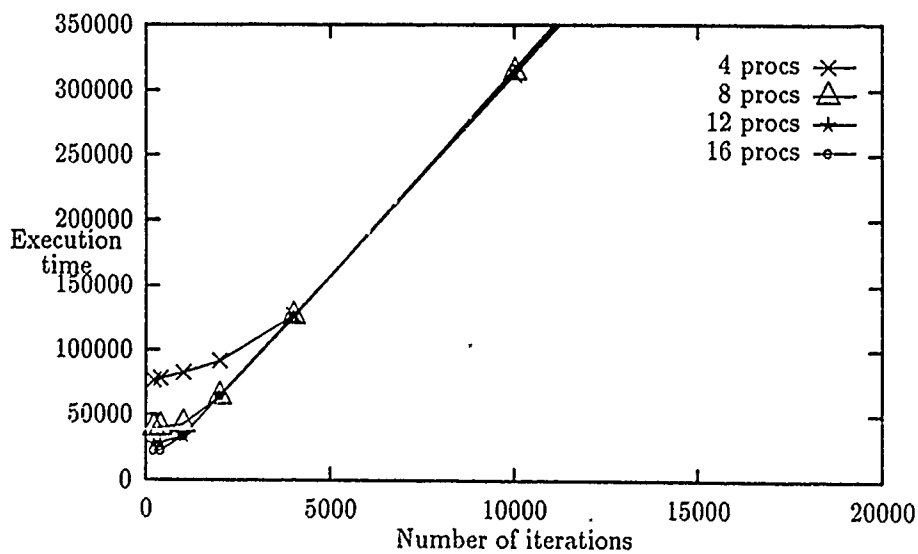
Figure 17: Execution time vs. number of iterations for exchange-byte primitive
