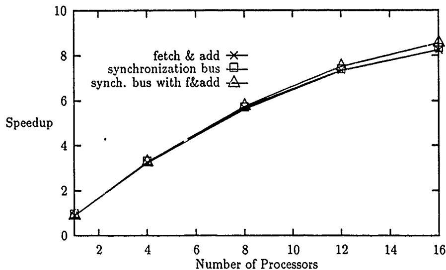
Figure 24: Performance of BDNA program with the use of synchronization bus and fetch&add primitive
