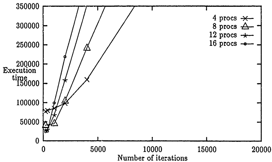
Figure 16: Execution time vs. number of iterations for test&set primitive
