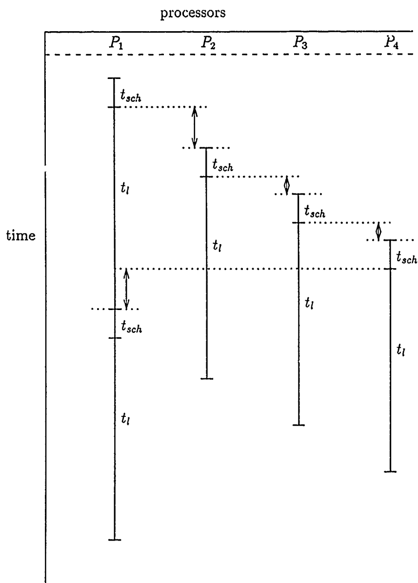
Figure 10: Scheduling of iterations for Case 1
