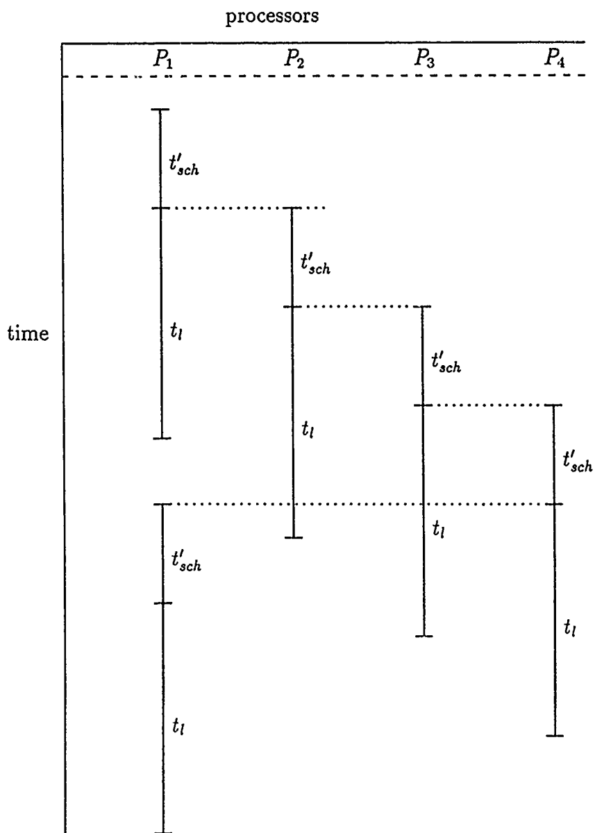
Figure 11: Scheduling of iterations for Case 2
