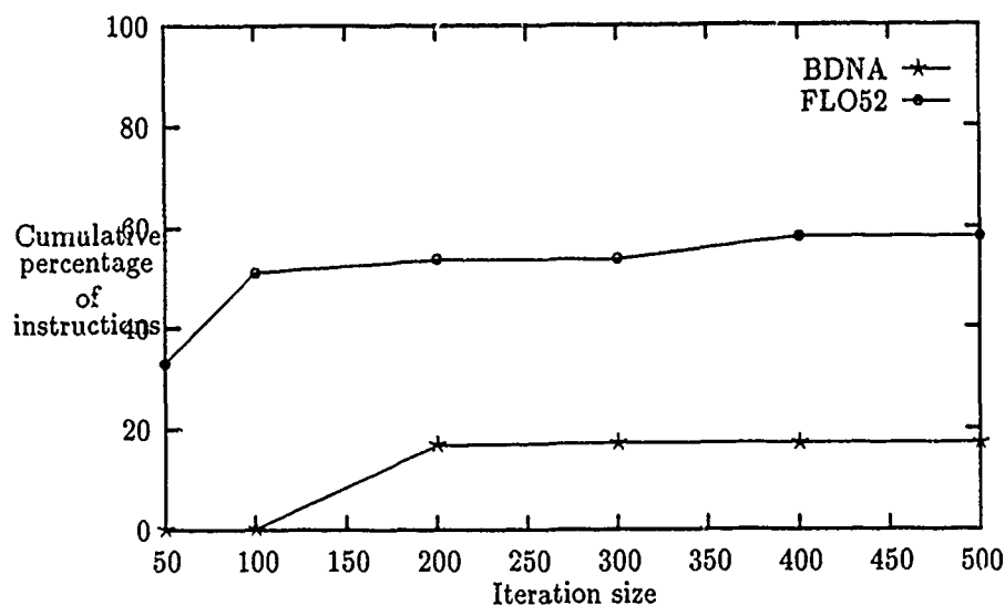
Figure 21: Cumulative distribution of dynamic instructions for loop iteration size
