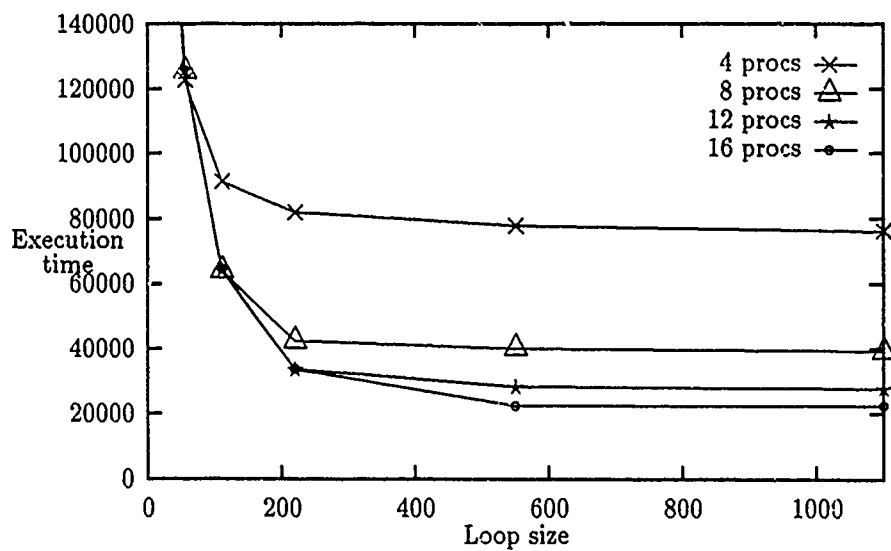
Figure 13: Execution time vs. granularity for exchange-byte primitive
