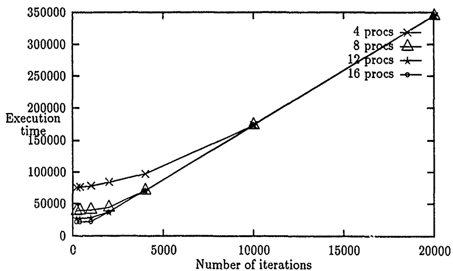
Figure 18: Execution time vs. number of iterations for synchronization bus
