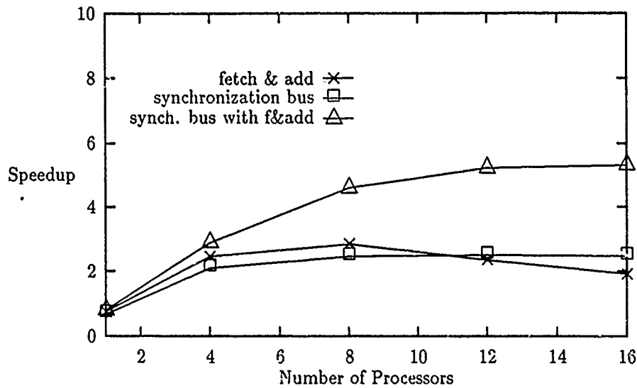
Figure 25: Performance of FLO52 program with the use of synchronization bus and fetch&add primitive
