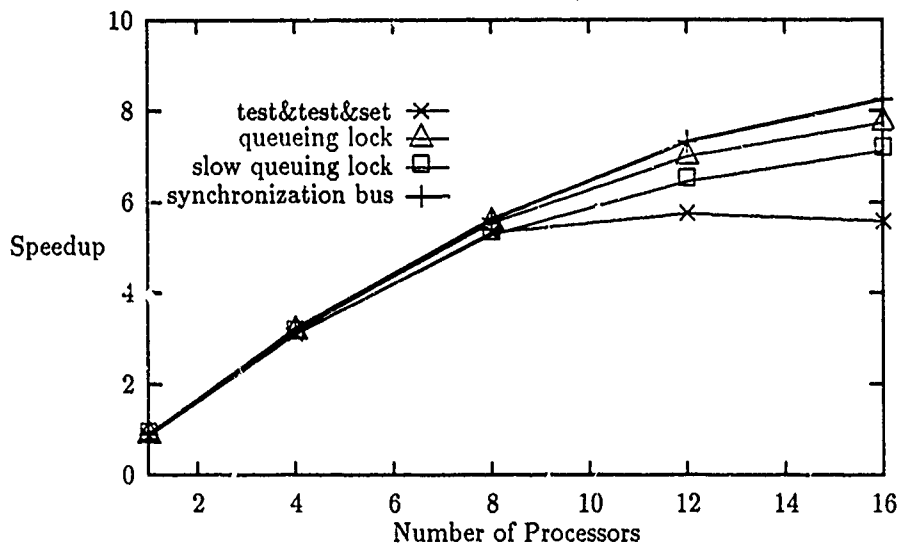
Figure 22: Lock latency and contention effects on BDNA program
