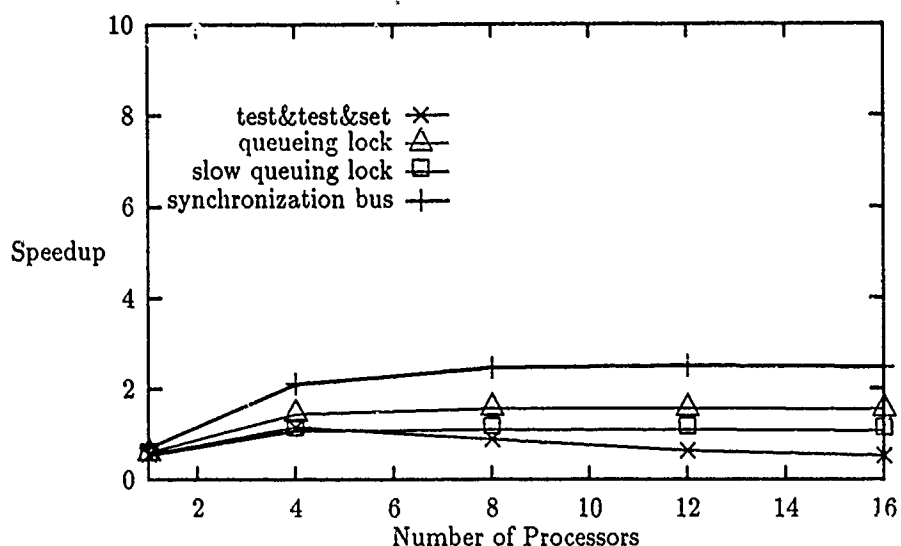
Figure 23: Lock latency and contention effects on FLO52 program
