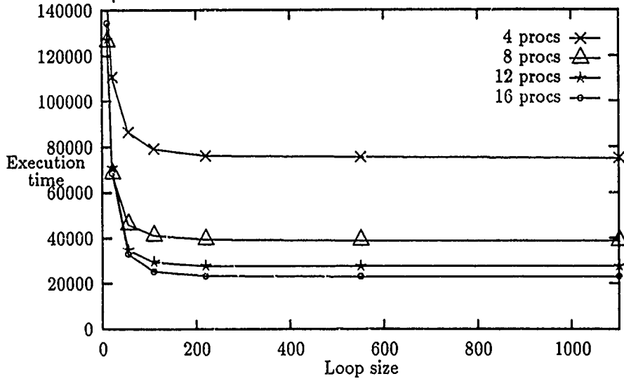
Figure 15: Execution time vs. granularity for fetch&add primitive
