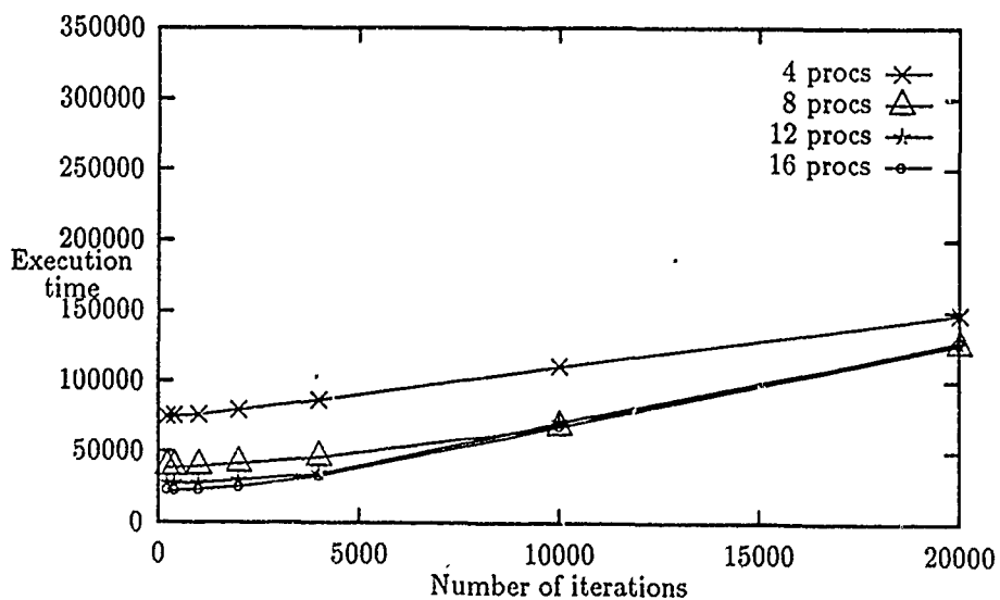
Figure 19: Execution time vs. number of iterations for fetch&add primitive
