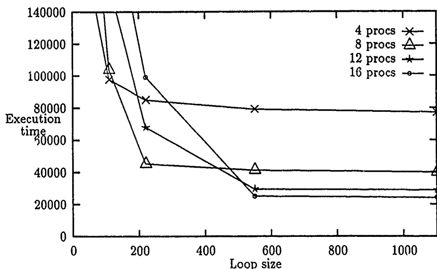
Figure 12: Execution time vs. granularity for test&set primitive
