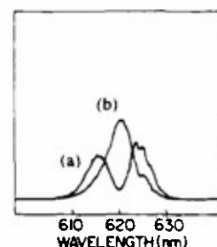
Fig. 9. Coincident spectra of the counterpropagating beams. (a) Clockwise beam, (b) counterclockwise beam. The conditions were the same as Figs. 1(b) and 7; the clockwise spectrum here corresponds to the midperiod of Fig. 7(b).
