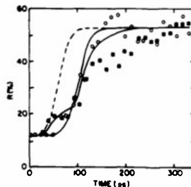
Fig. 5. Reflectivity jump at 532 nm due to melting of silicon, measured at 60^\circ and for two pump energies just above threshold E_T (○) and \sim 4 \times E_T (■). The full lines are obtained from a computer simulation which includes heating of the liquid, while the dashed line assumes that the temperature never exceeds T_m for the higher pump energy.
