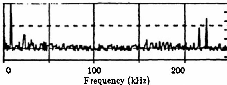
Figure 4 a) Single-sweep intensity autocorrelation trace showing what appears to be sub-100 fsec modulation (27 fsec delay per division or 0.1 msec per division) b) Frequency content of the output train showing beating between two solitons with \sim 5 \mu\text{sec} periods for a situation similar to Fig. 4 a). The \sim 10 \text{ kHz} beat frequency produces the deep modulation seen in Fig. 4 a) because one arm of the autocorrelator is driven at a low audio frequency.
