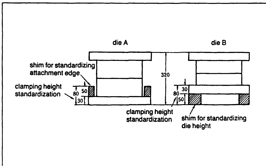
Figure 2. Function Standardization of Die Height and Clamping Edge
