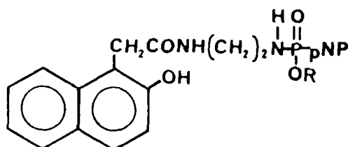
XVII ( \text{R} = \text{C}_2\text{H}_5 ); XVIII ( \text{R} = \text{C}_3\text{H}_7 )
