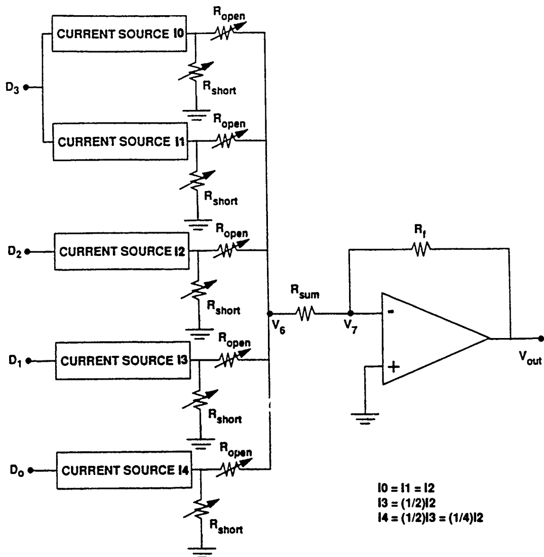
Figure 2-8A. 4-bit D/A converter. The current sources are switched on by application of 5V to the control inputs D_n . The variable resistors represent the application of shorts and opens to the current source outputs.
