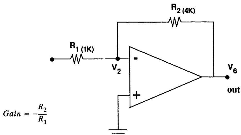
Figure 2-3B. Inverting amplifier configuration. The op-amp is represented by the behavioral model of Figure 2-3A.
