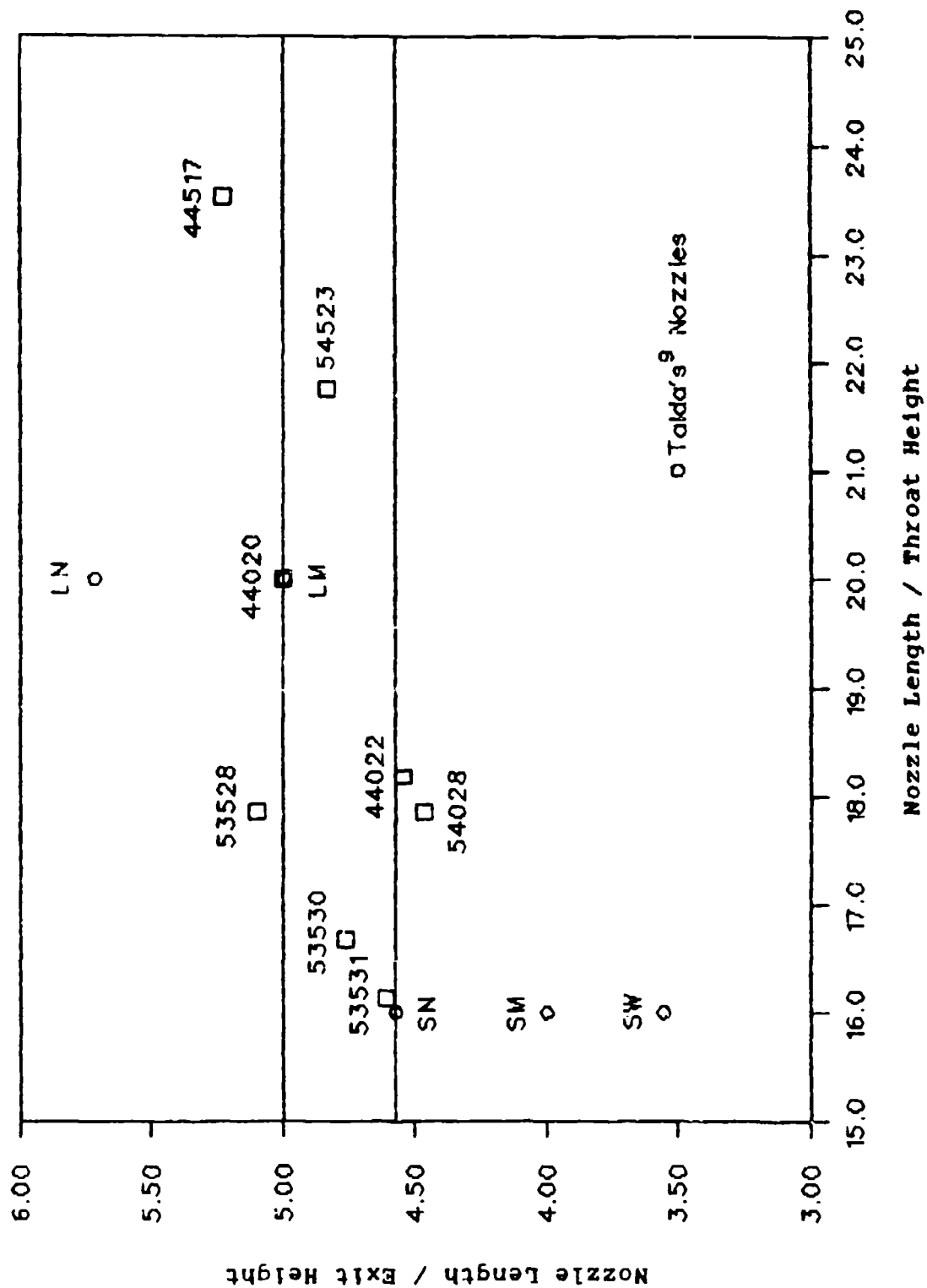
Figure 31. Design Guidelines for 2-D CJTVC Nozzles (Talda 9 )
