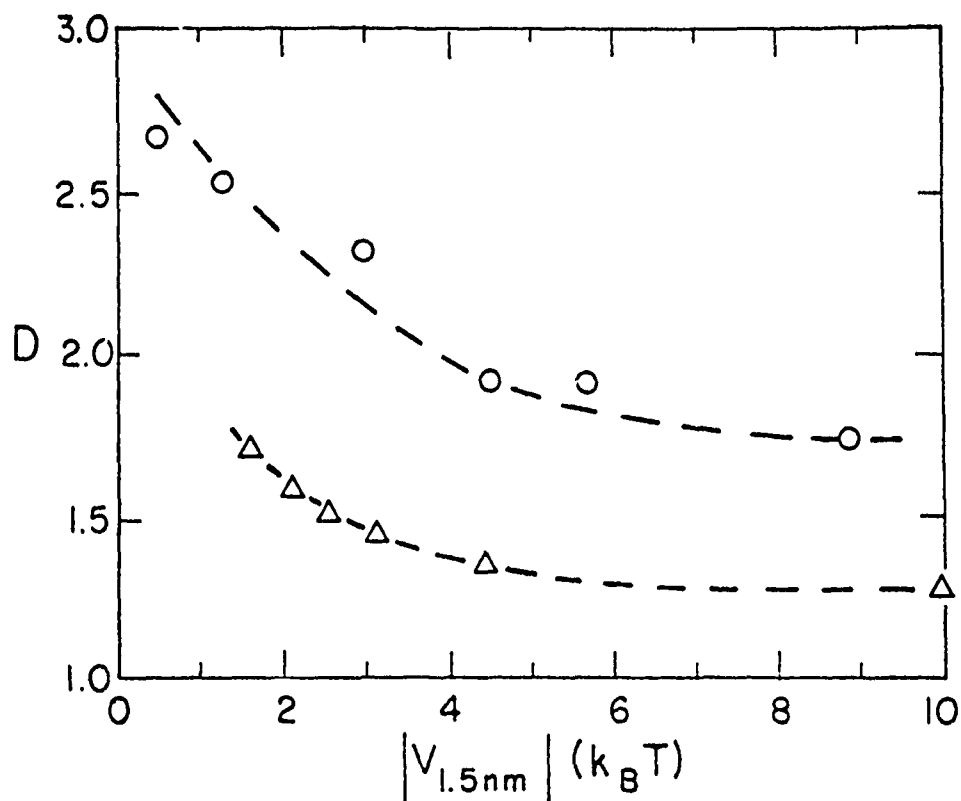
Figure 3. Fractal dimension D versus |V_{1.5\text{ nm}}| for the gold aggregates (O) where |V_{1.5\text{ nm}}| is the magnitude of the attraction energy between gold particles at the average closest distance 1.5 nm. Also plotted is the D versus \bar{E} ( \Delta ) where \bar{E} is nearest-neighbor attraction energy from the computer simulations of Shih, et al. 1 in two dimensions. Although the computer simulations of Ref. 1 were done in two dimensions, the resemblance of the two curves to each other is remarkable, suggesting that the reversible aggregation process in colloids can be represented by the model of Shih et al.
