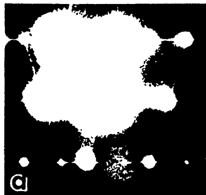
Figure 2. (a) SAD pattern and its analysis (b). Note the streaks due to \{01\bar{1}1\} twins.
