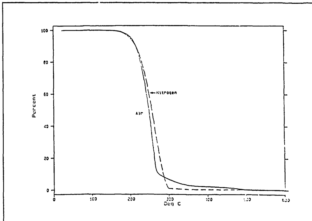
Figure 3. TGA weight loss data for paraffin wax in different furnace atmospheres.
