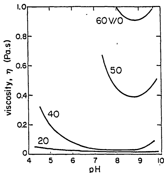
Figure 5: Viscosity (at 9.3 \text{ s}^{-1} ) of aqueous \alpha\text{-Al}_2\text{O}_3 ( 0.4 \mu\text{m} ) suspension stabilized with a Na+ salt of PMAA polyelectrolyte as a function of pH from 20 to 60 v/o solids concentration.
