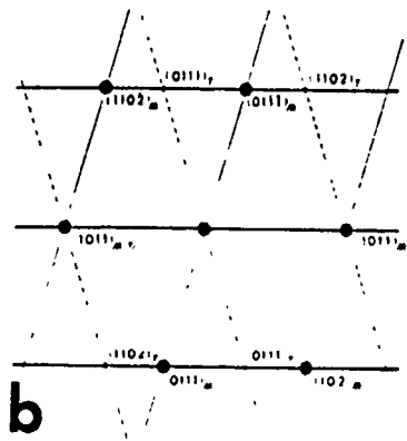
Figure 2. (a) SAD pattern and its analysis (b). Note the streaks due to \{01\bar{1}1\} twins.
