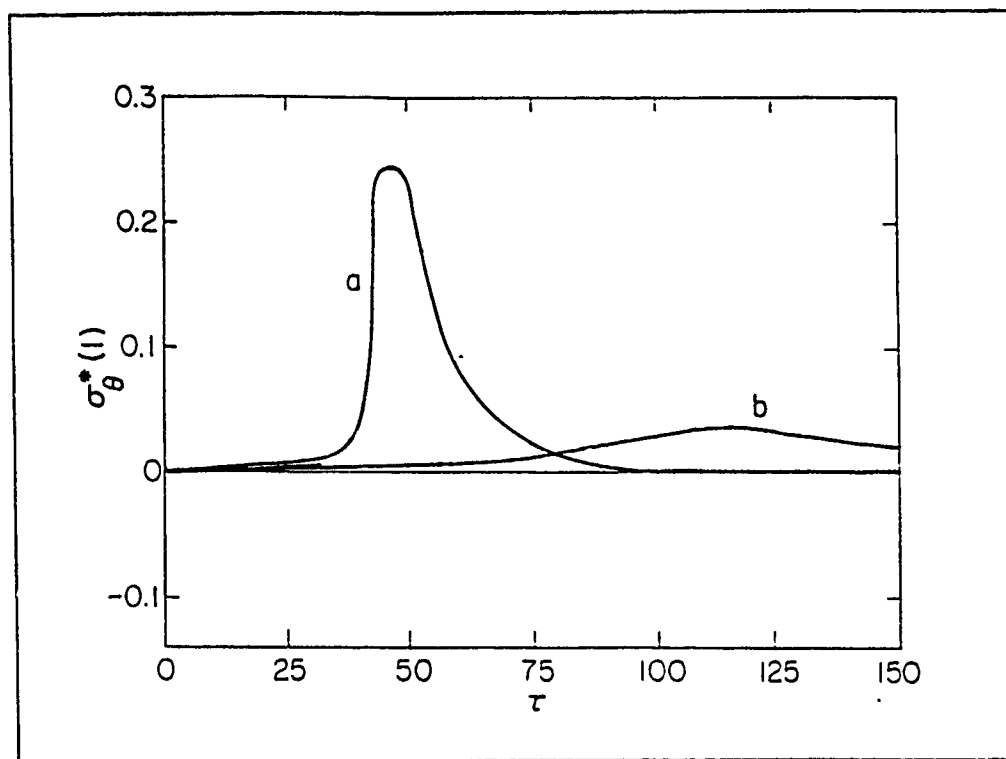
Figure 6. Internal stress profiles corresponding to saturation profiles in Figure 5. (a) T_f = 230^\circ\text{C} ; (b) T_f = 155^\circ\text{C}
