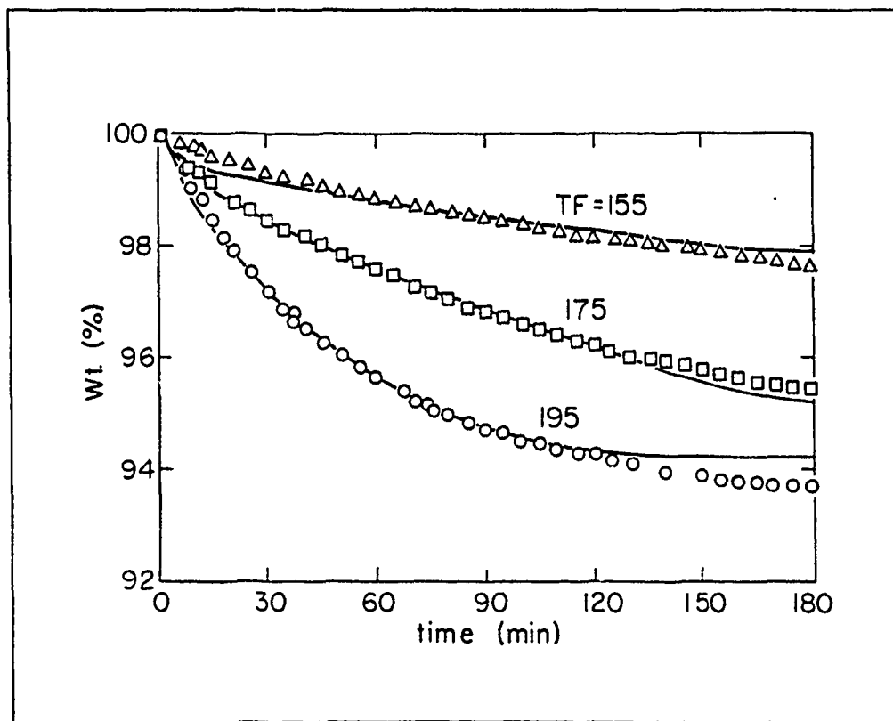
Figure 2. Comparison of model predictions with experimental TGA data. From ref. [14].
