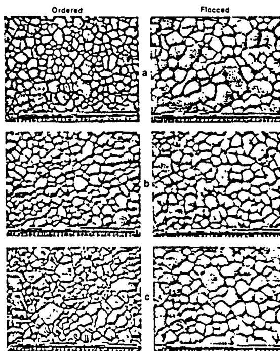
Figure 11. Micrographs of surface grain shapes for the 170 g ordered and flocced compacts sintered at 1150°C for (a) 10 minutes, (b) 2 hours, and (c) 10 hours (note scale changes).
