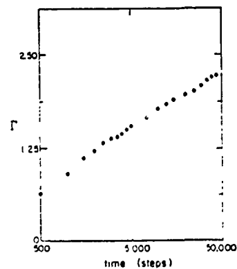
Fig. 3. The adsorption amount \Gamma vs. time for N_1 = 45 .
