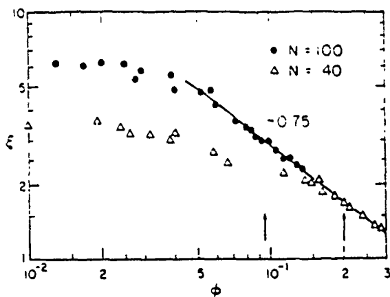
Fig. 6. \xi vs. \phi for N = 40 ( \Delta ) and for N = 100 ( \bullet ) where \xi is the correlation length and \phi is the bulk segment density.
