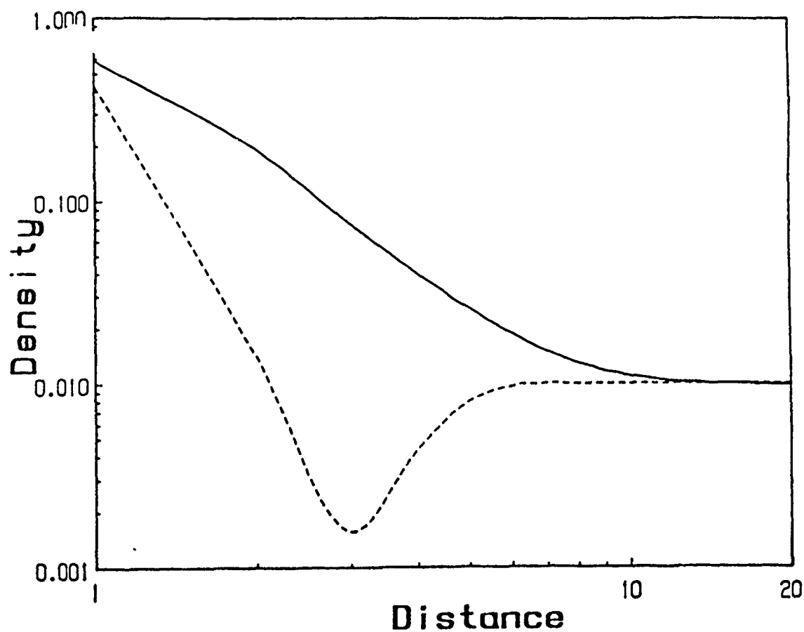
Fig. 2 Analytical results for adsorption due to the CVM.
