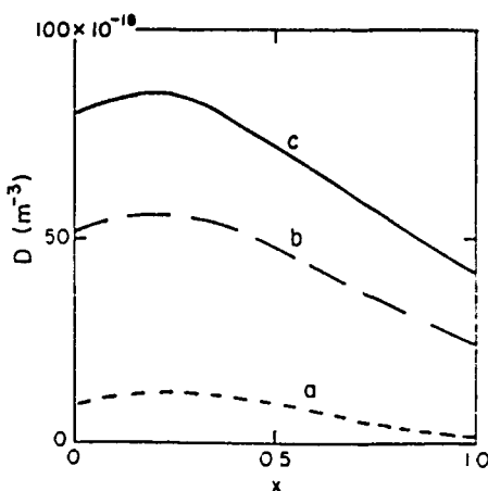
FIG. 5. D - x phase diagrams of binary colloidal particles where a_1 = 545 , Z_1 = 300 and a_2 = 445 , Z_2 = 245 . Curve (a) is the freezing density without adding salt, (b) is that with 10 \mu\text{M} salt, and (c) is with 20 \mu\text{M} salt.
