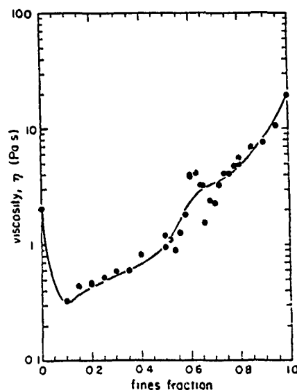
Figure 6: Zero-shear viscosity of an aqueous \alpha\text{-Al}_2\text{O}_3 ( 0.8 \mu\text{m} ) suspension as a function of fraction of fines ( 0.18 \mu\text{m} ) at a fixed solids loading of 50%.
