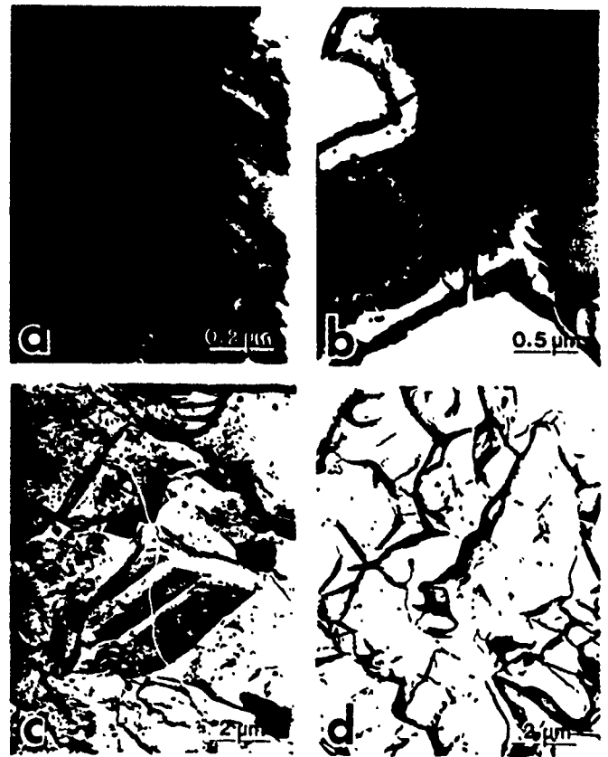
Figure 3. BF images from statically ((a) and (c)) and dynamically ((b) and (d)) loaded samples; thin foil ((a) and (b)) and replicas ((c) and (d)).
