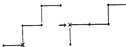
Fig. 1b. A monomer can wiggle within a chain (segment flipping).
