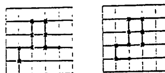
Fig. 1c. Reptation
