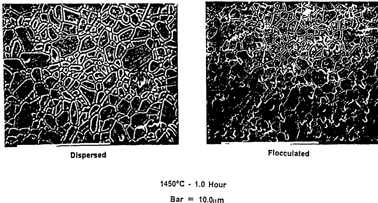
Figure 9. Effect of processing path upon microstructure of \text{Al}_2\text{O}_3 after densification by sintering for 1 hr. at 1450°C. Bar = 10.0 µm.
