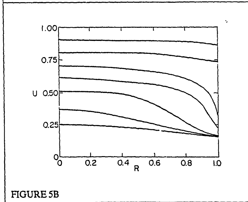
Figure 5. Liquid saturation profiles at (a) T_f = 155^\circ\text{C} and (b) 230^\circ\text{C} . By definition: R = r/r_p = dimensionless radial coordinate; U = dimensionless saturation parameter ( U = 1 when pores are full, and U=0 when empty); and \tau = \alpha_s t/r_p^2 = dimensionless time. The quantities r_p and \alpha_s are sample radius and thermal diffusivity, respectively.
