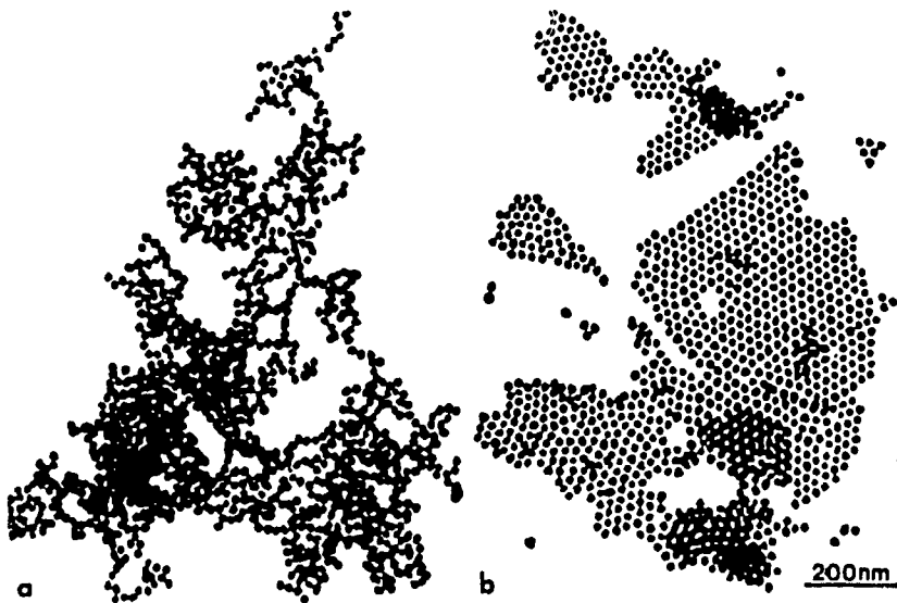
Figure 8: (a) Fractal clusters of 15 nm gold particles that result in the formation of low density compacts; (b) The dense packing of the same gold particles after they are first coated with lubricating surfactants (53).
