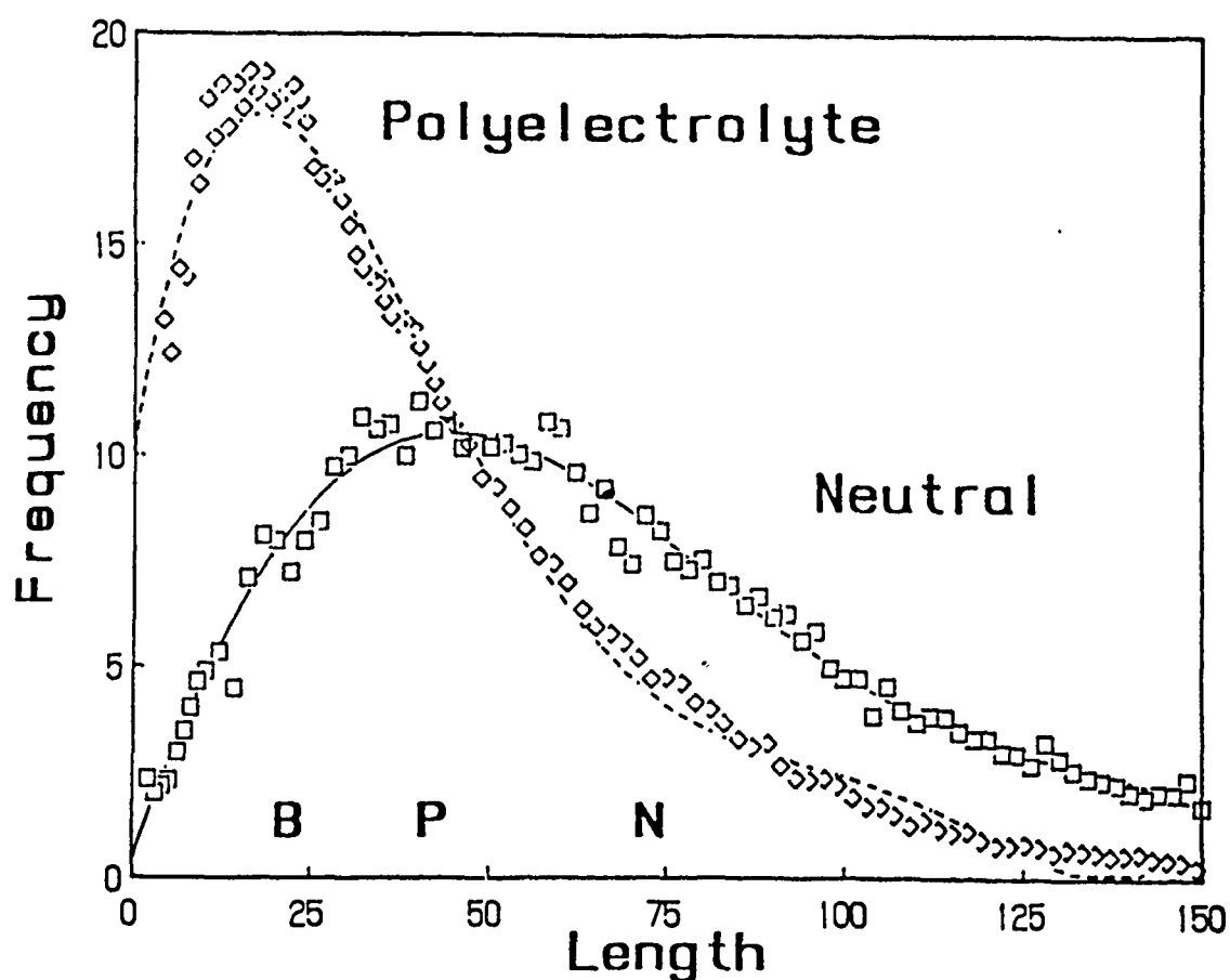
Fig. 3 Length dependence of adsorption obtained by the CVM simulation. The points B, P and N indicate the average lengths of the bulk, polyelectrolytes and neutral polymers.
