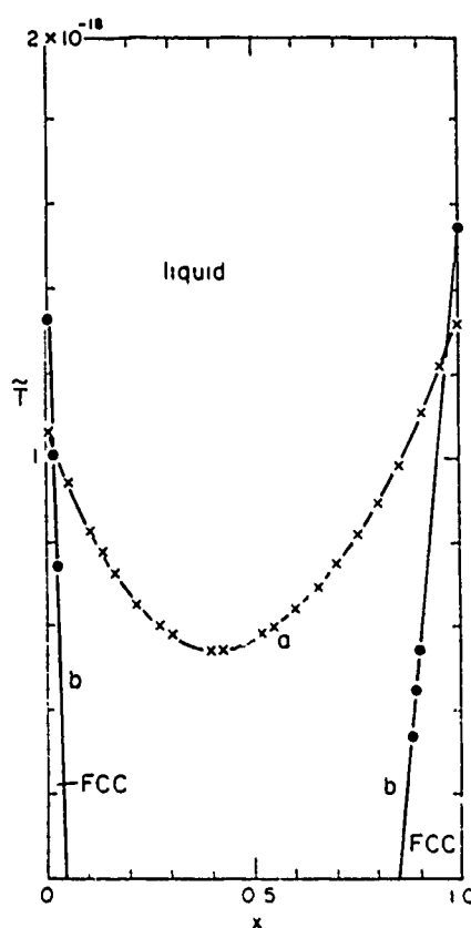
FIG. 2. \tilde{T} - x phase diagrams of the binary colloidal particles in Fig. 1. \tilde{T} is the effective temperature as defined in the text, and x is as in Fig. 1.
