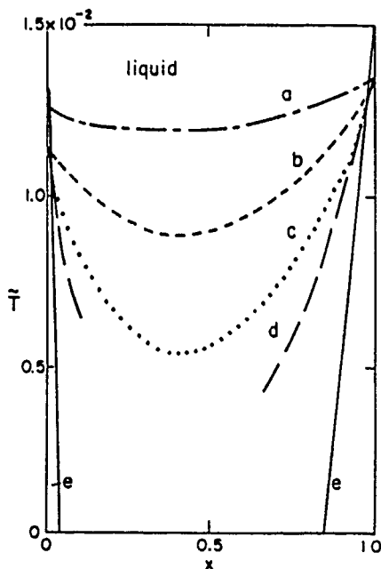
FIG. 4. \bar{T} - x phase diagrams of binary colloidal particles. Curves (a)–(d) correspond to the freezing temperatures of Figs. 3(a)–3(d) while (e) corresponds to Fig. 1(b).
