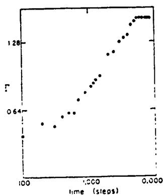
Fig. 2. The adsorption amount \Gamma vs. time for N_1 = 10 .
