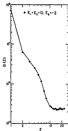
Fig. 4. The adsorption density profile of homopolymers of N = 45 .
