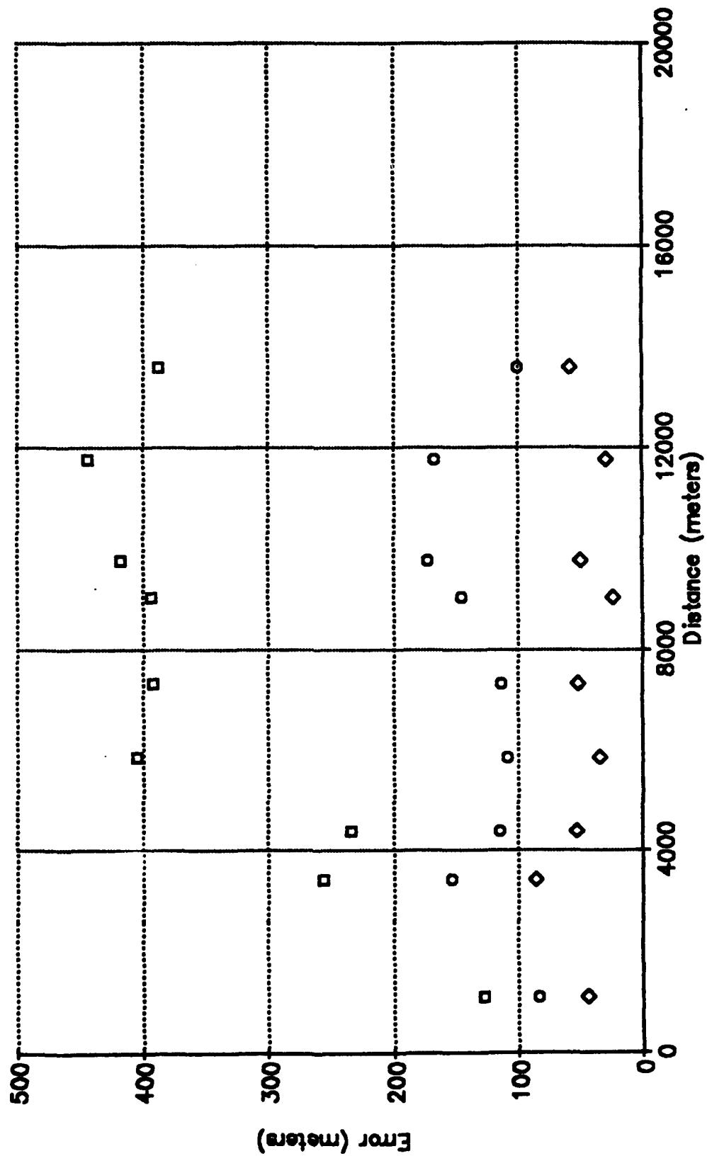
Figure 27. April SNDR Error Plot
