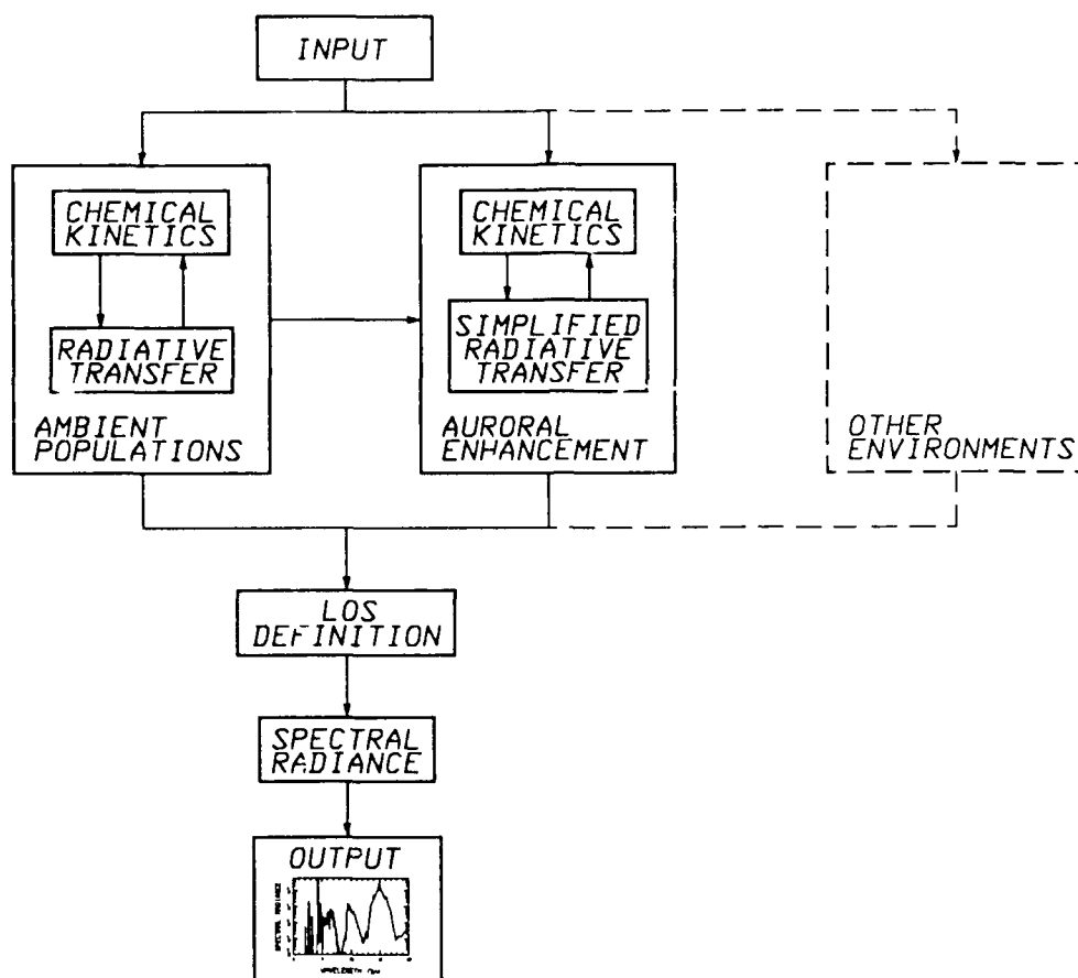
Figure 6. Computational Sequence for SHARC.
