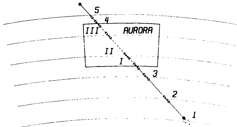
Figure 8. Layering Schematic with Local Auroral Region.
