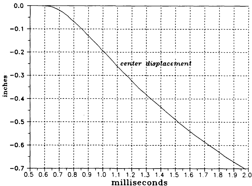
Fig. 4-15: Numerical modeling of a larger scale test (m) - Pressure over the roof and motion records of the roof center.
