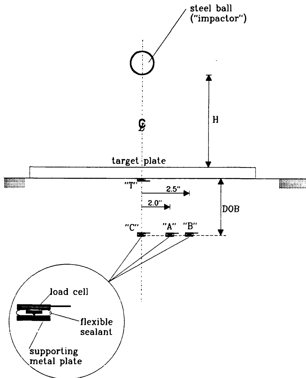
Fig. 2-6: Setup for measurement of the free field vertical stress distribution.
