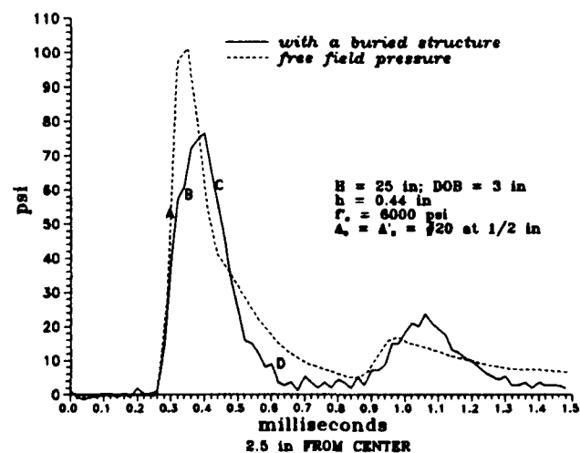
Fig. D-1: Pressure records over a simply supported roof in test 2 v.s. free field (4 th hit).
