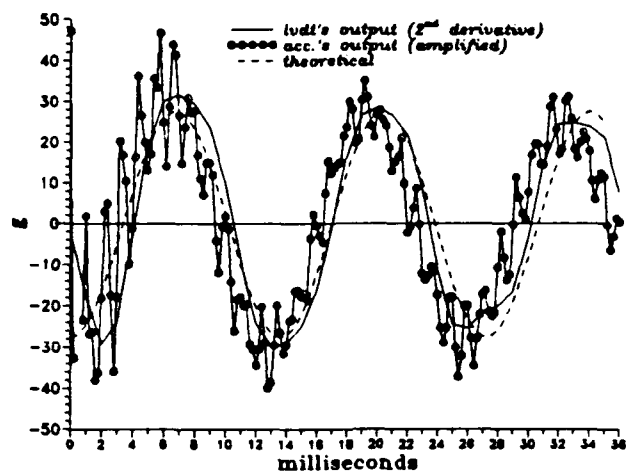
Fig. B-3(c): Acceleration of a cantilever end at L = 8 in.
