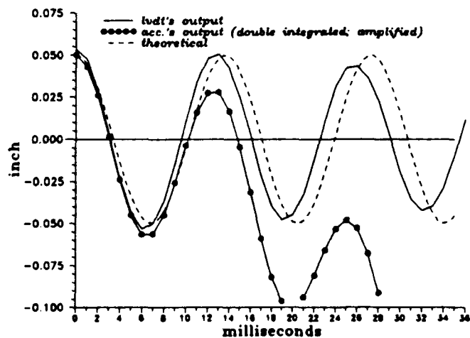
Fig. B-3(a): Displacement of a cantilever end at L = 8 in.
