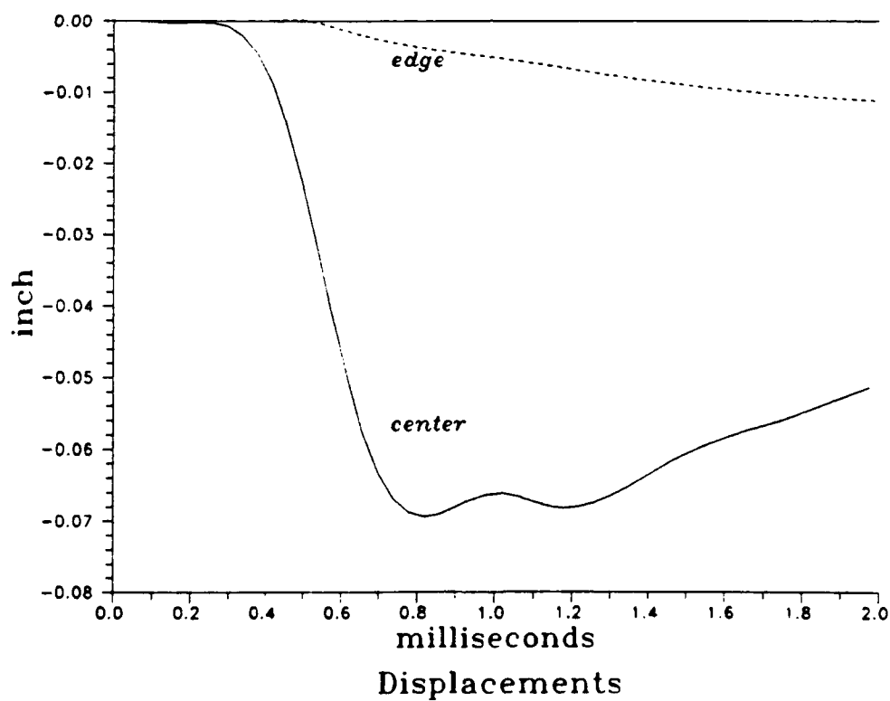
Fig. 2-17: Response of the plexiglas roof. (DOB = 3 in; H = 25 in)
