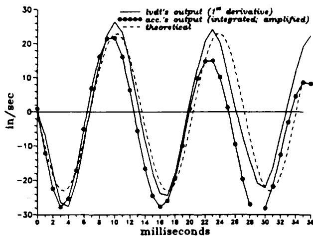
Fig. B-3(b): Velocity of a cantilever end at L = 8 in.
