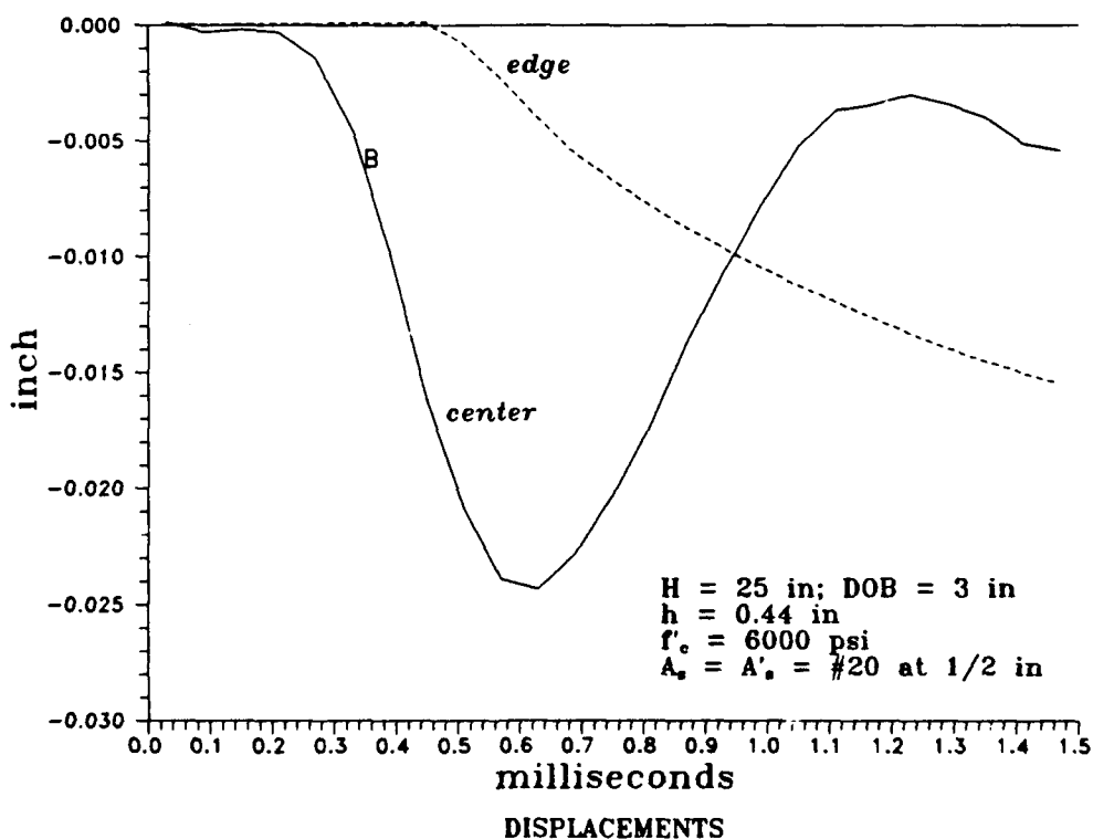
Fig. D-2: Response of the simply supported roof in test 2.
