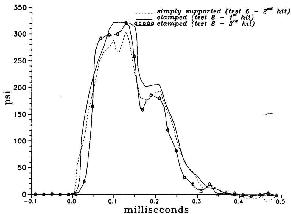
Fig. 2-27: Pressure under the target plate center - H = 25 in, DOB = 2.5 in.
