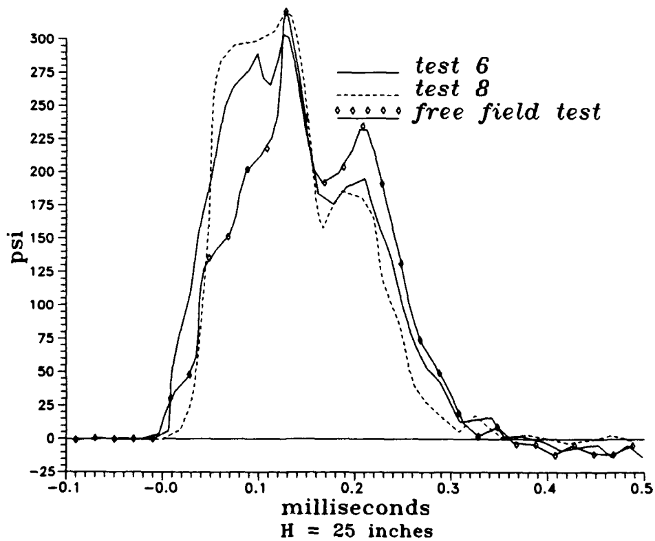
Fig. D-10: Pressure induced under the target plate center in the tests with DOB = 2.5 inches.
