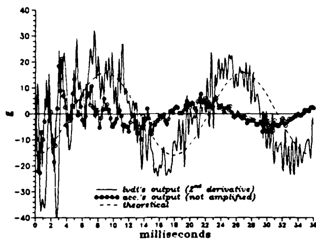
Fig. B-4(c): Acceleration of a cantilever end at L = 9 \frac{7}{16} in.
