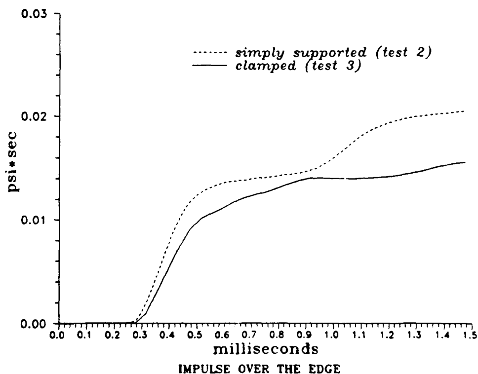
Fig. 2-26: Simply supported v.s. clamped roof - impulse records. (DOB = 3 in; H = 25 in)
