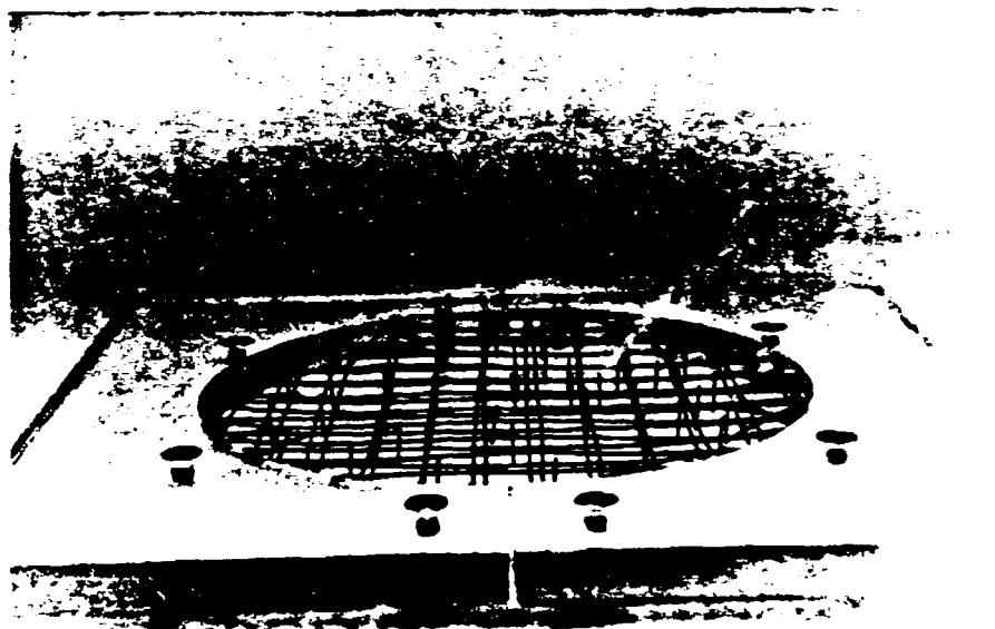
Fig. 2-10-a: Form and reinforcement ready for casting of micro-concrete slabs.
