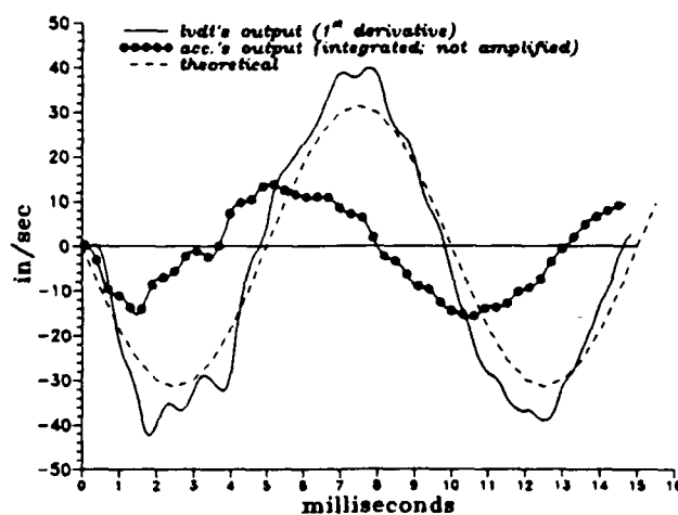
Fig. B-2(b): Velocity of a cantilever end at L = 6 \frac{5}{8} in.
