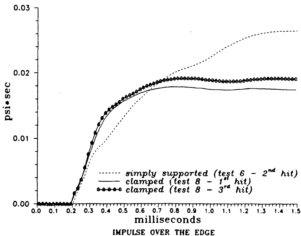
Fig. 2-29: Simply supported v.s. clamped roof - impulse records. (DOB = 2.5 in; H = 25 in)
