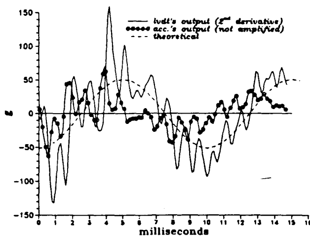
Fig. B-2(c): Acceleration of a cantilever end at L = 6 \frac{5}{8} in.
