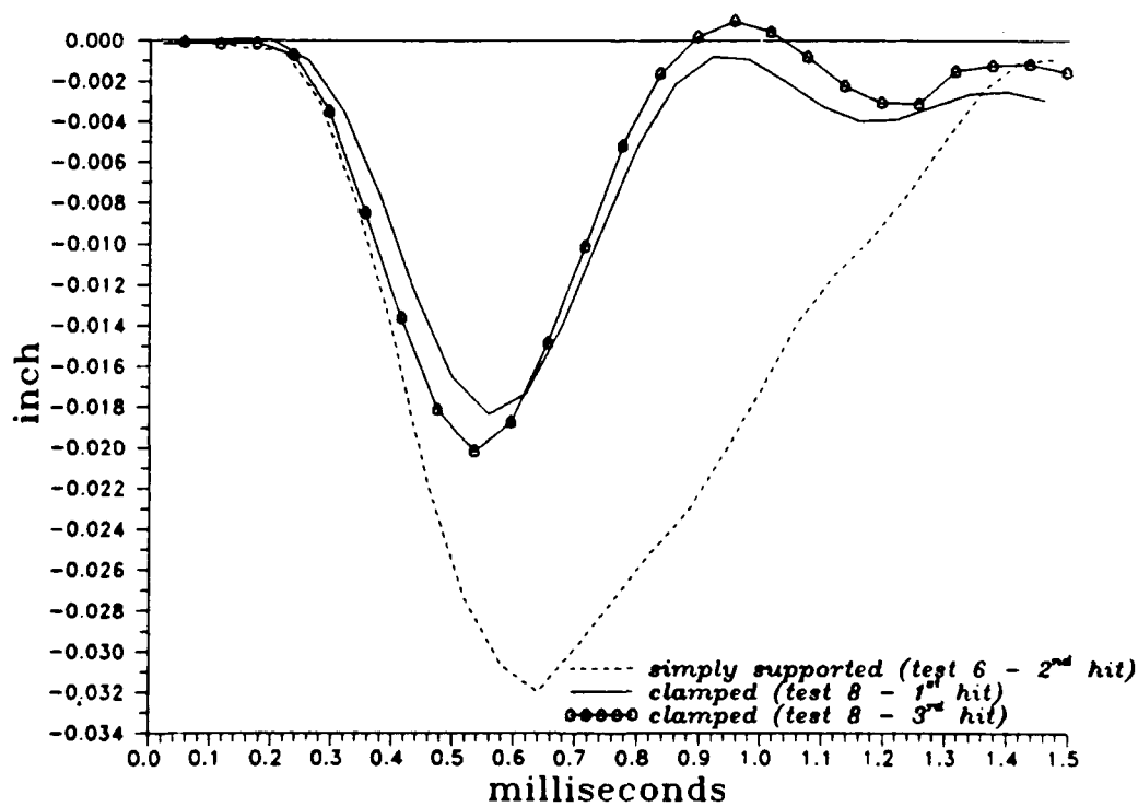
Fig. 2-28: Simply supported v.s. clamped roof - displacement of the roof center ( DOB = 2.5 in; H = 25 in).
