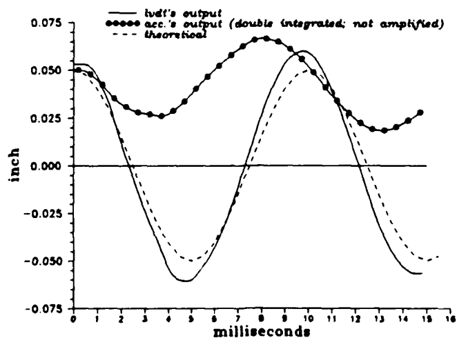
Fig. B-2(a): Displacement of a cantilever end at L = 6 \frac{5}{8} in.
