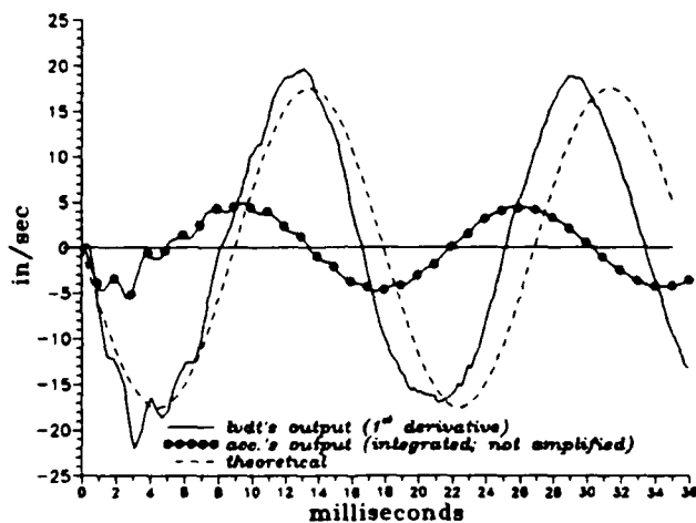
Fig. B-4(b): Velocity of a cantilever end at L = 9 \frac{7}{16} in
