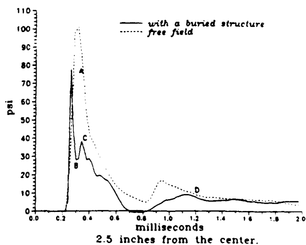
Fig. 2-18: Pressure at buried roof level v.s. free field. (Plexiglas roof; DOB = 3 in. H = 25 in)
