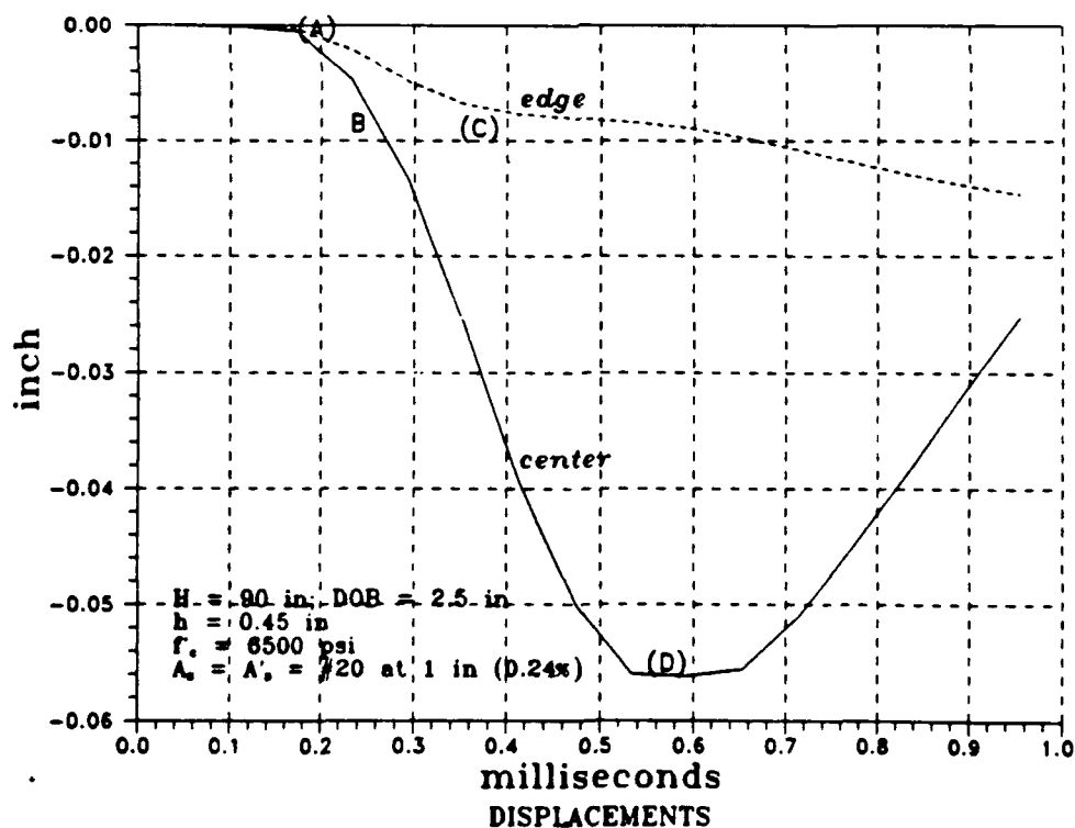
Fig. 2-21: Response of the clamped roof in test 8 (5 th hit).
