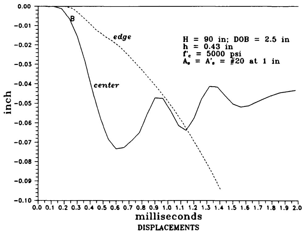
Fig. D-5: Response a simply supported roof in test 6 (4 th hit).
