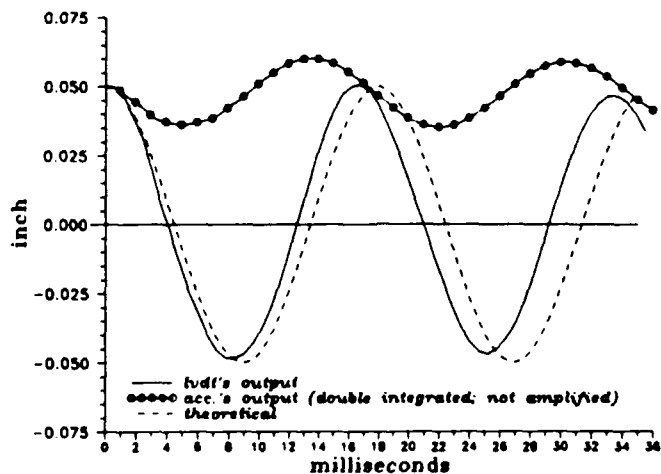
Fig. B-4(a): Displacement of a cantilever end at L = 9 \frac{7}{16} in.
