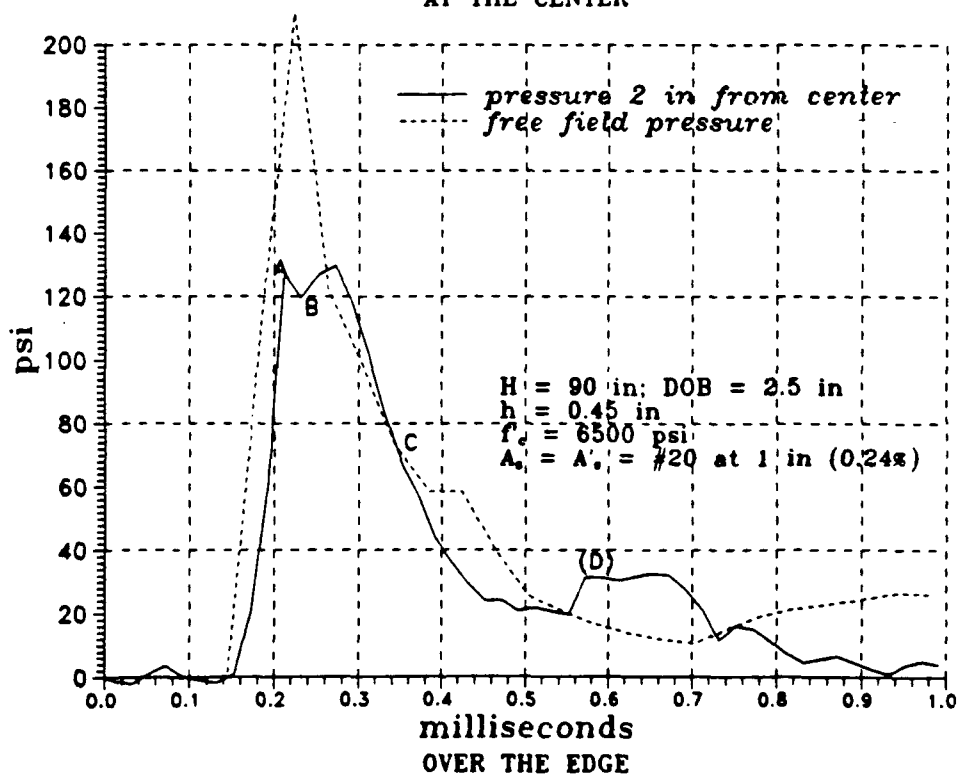
Fig. 2-20: Pressure over the clamped roof of test 8 (5 th hit) v.s. free field.
