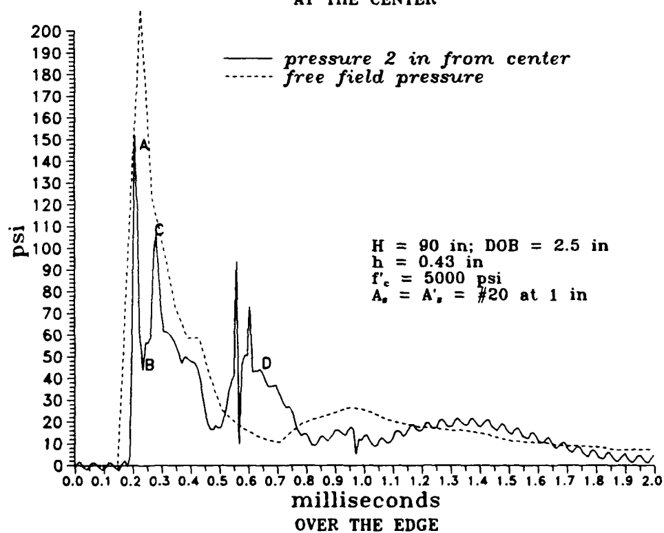
Fig. D-4: Pressure over the simply supported roof in test 6 (4 th hit) v.s. free field.
