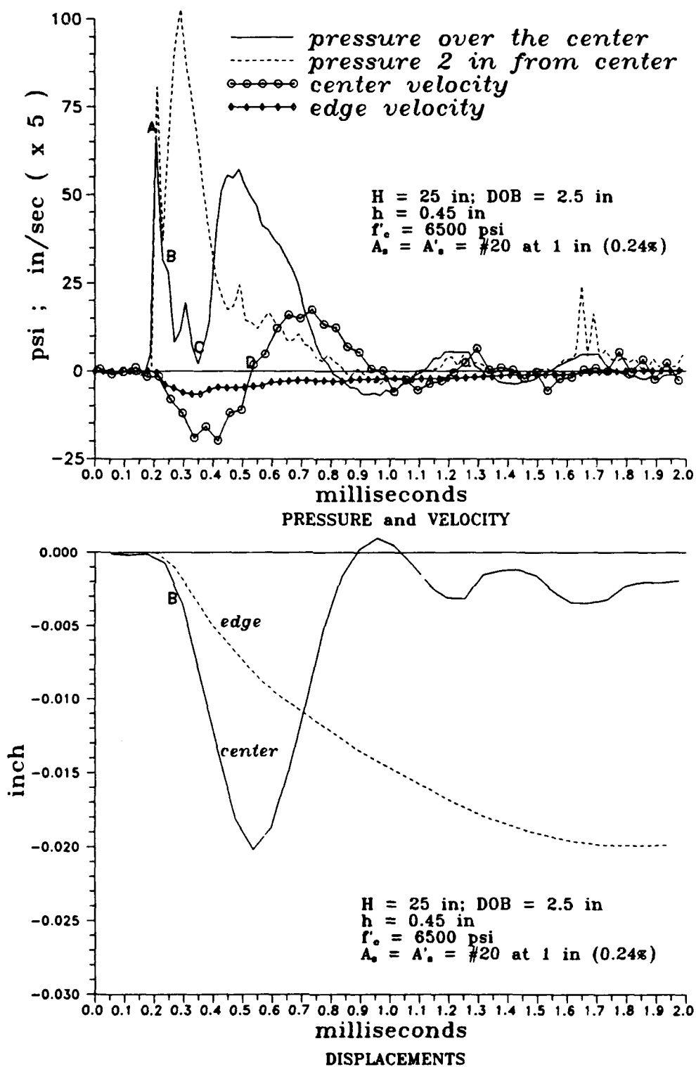
Fig. D-8: Response of a clamped roof in test 8 (3 rd hit).
