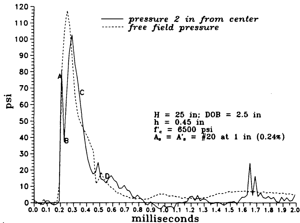
Fig. D-7: Pressure over the clamped roof in test 8 v.s. free field (3 rd hit).
