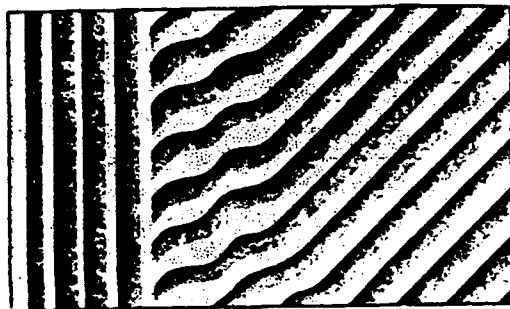
Fig. 4. Resolution of discharge with a rotating mirror. Left - stationary striae, right - pulsing.
