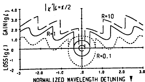
Fig. 10. Parametric gain \kappa'l and linear gain gl versus normalized wavelength detuning at the oscillation condition.
