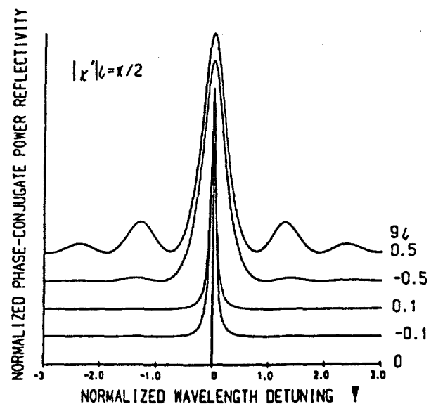
Fig. 6. Normalized phase-conjugate power reflectivity versus normalized wavelength detuning \Psi for parametric gain |\kappa' l| = \pi/2 and several values of linear gain g_l . All curves are normalized to unity power reflectivity to emphasize the frequency bandpass of the interaction.
