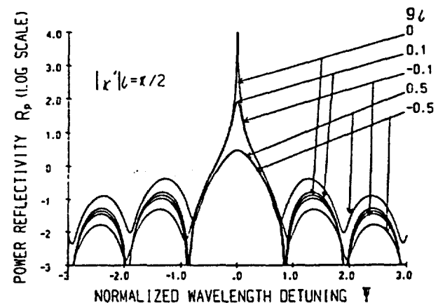
Fig. 5. Power-reflection coefficient R_p versus a normalized wavelength-detuning parameter \Psi for |\kappa' l| = \pi/2 and several values of the linear gain g_l . For the example given in the text, unity along the abscissa corresponds to \Delta\lambda/2 = 0.0772 \text{ \AA} , or \Delta\nu = 9.26 \text{ GHz} .
