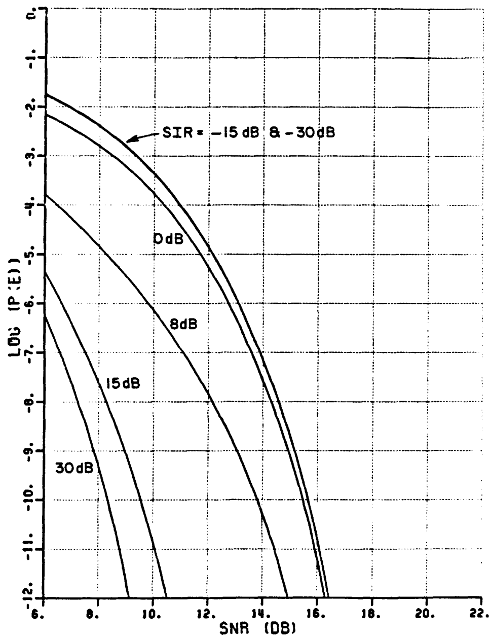
Figure 7.6. P(e) vs. SNR for 3-element narrowband array ( \theta_d=0^\circ , \theta_i=10^\circ , k=1/2 ).
