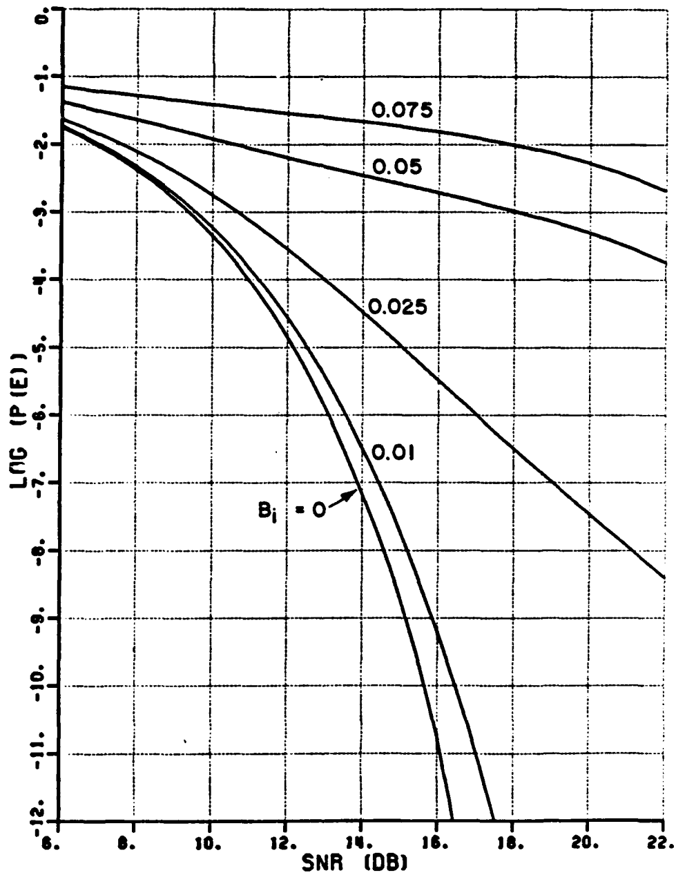
Figure 8.5. Three-element array performance with noise interference ( \theta_d=0^\circ , \theta_i=10^\circ , k = 1/2 , B_d = 0.1 ).
