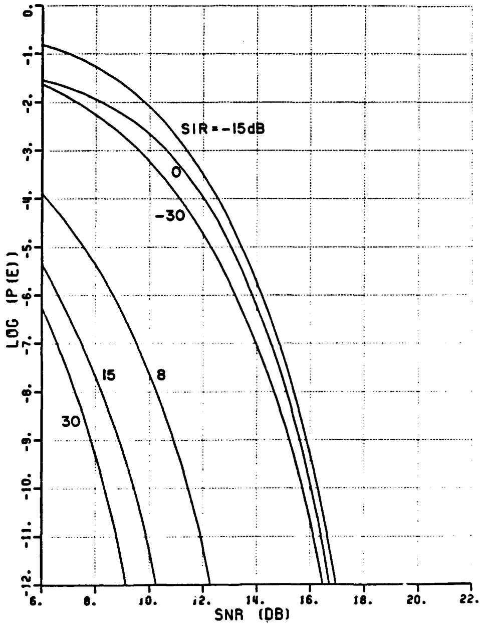
Figure 3.14. BPSK P(e) vs. SNR for 3-element array ( \theta_i=10^\circ , k=10 , \Delta\omega T=0 ).
