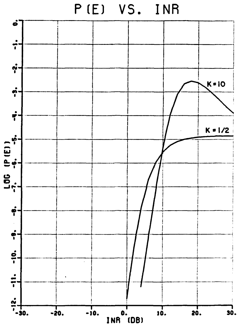
Figure 7.12. P(e) vs. INR for \text{SNR}=12 dB for two different k values ( \theta_d=0^\circ , \theta_i=10^\circ ).
