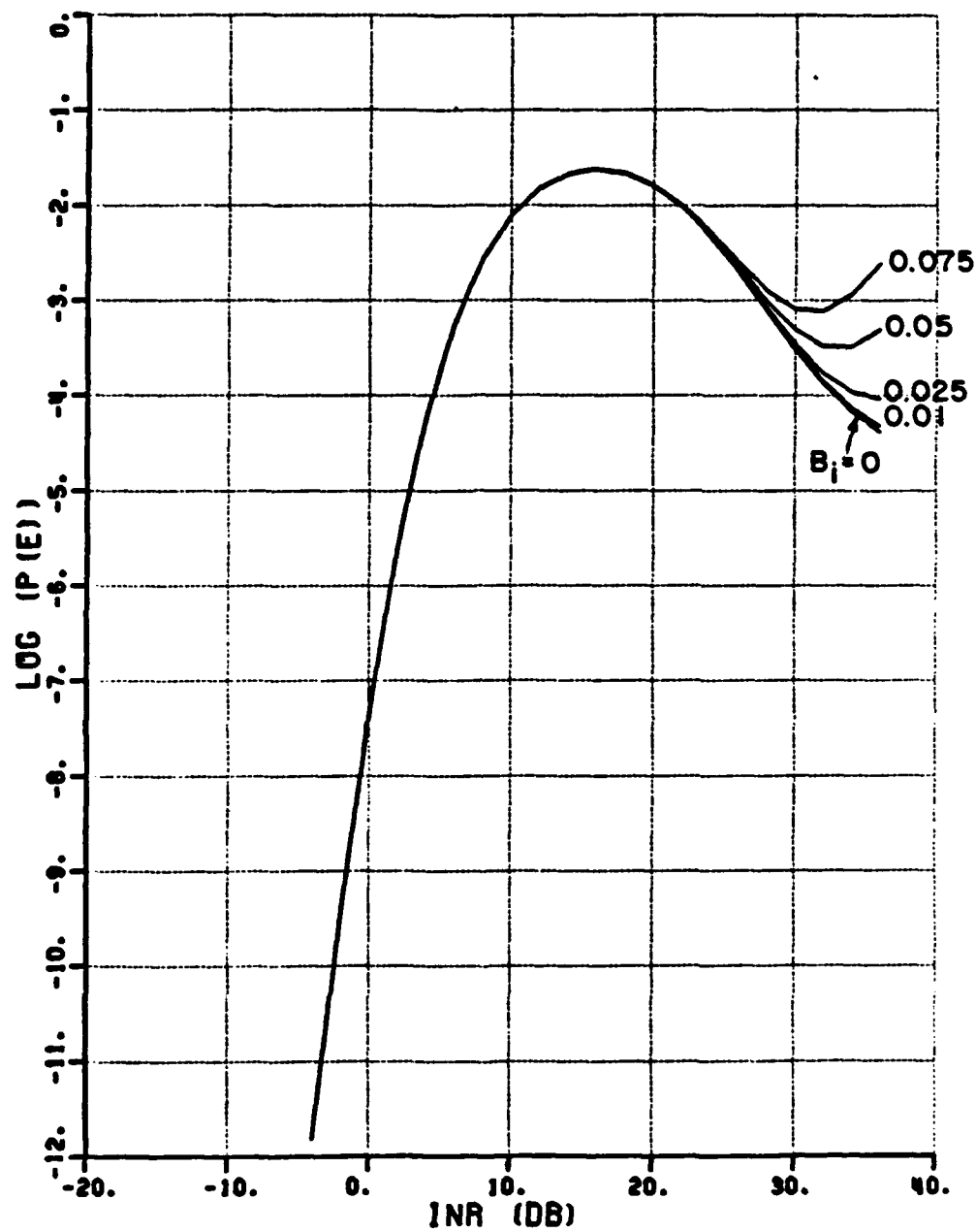
Figure 8.10. 3-element array performance - case (C).
