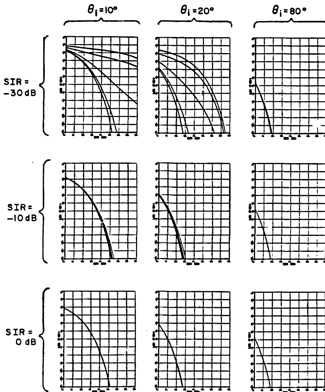
Figure 8.6. Performance of a 3-element array with noise interference for various SIR values ( \phi_d=0^\circ , k=1/2 , R_d=0.1 ). B_i values and scales are the same as those of Figure 8.5.
