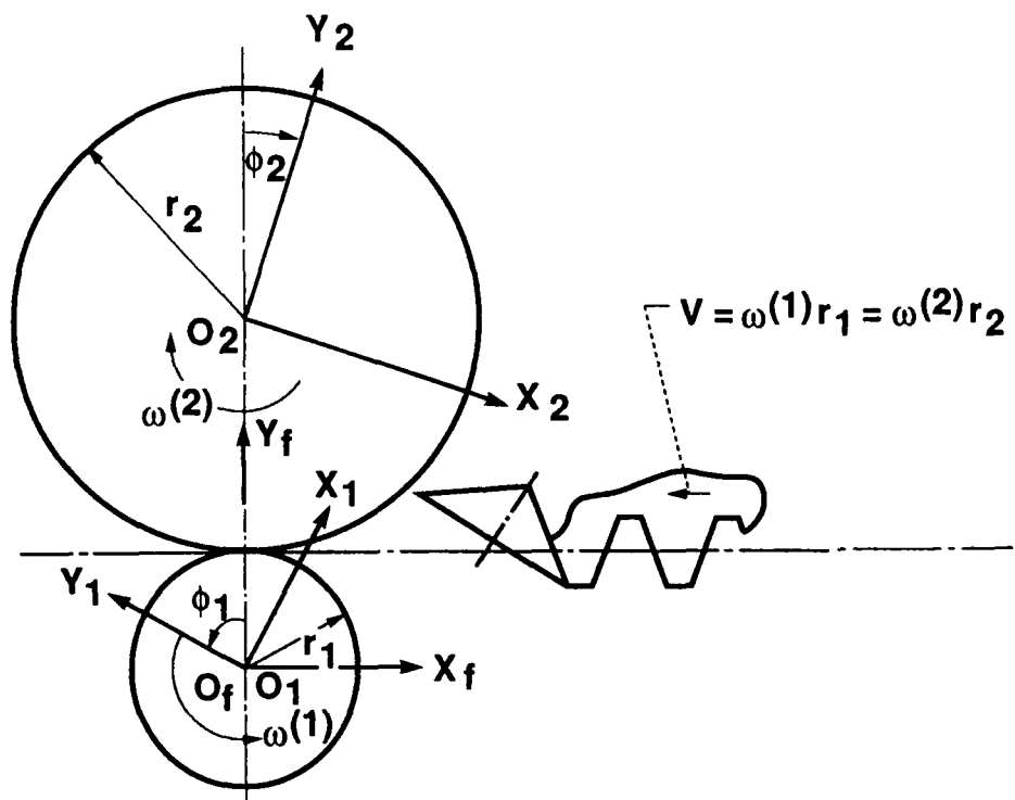
FIGURE 10. - GENERATION OF GEARS.
