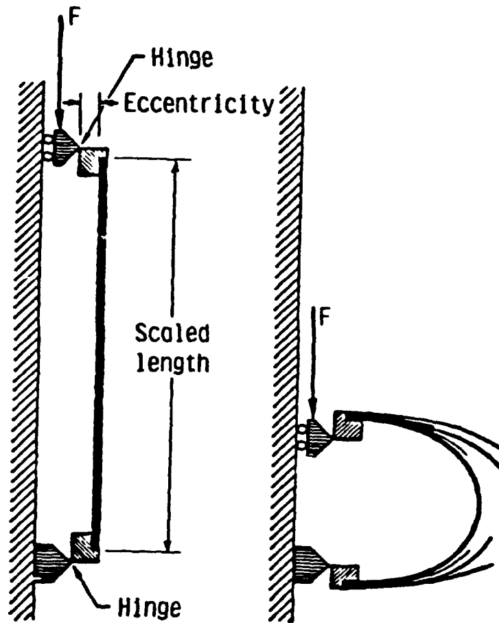
Figure 2. Schematic drawing of the test configuration.
