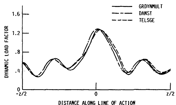
Figure 27.—Comparison of programs GRDYNMULT, DANST, and TELSGE. Dynamic load factor as function of contact position. Input torque = 203.4 N·m; input speed = 4000 rpm (Table VIII, run 7).
