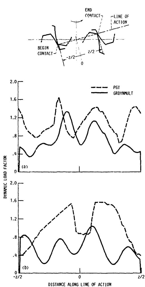
(a) PGT and GRDYNMULT sun/planet mesh. (b) PGT and GRDYNMULT ring/planet mesh. Figure 14.—Comparison of programs PGT and GRDYNMULT. Dynamic load factor as a function of contact position. Input torque = 33.9 N·m; input speed = 4000 rpm (Table V, run 1).
