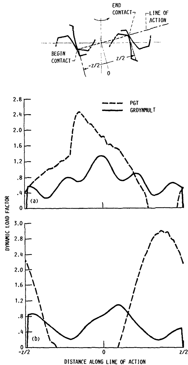
(a) PGT and GRDYNMULT sun/planet mesh. (b) PGT and GRDYNMULT ring/planet mesh. Figure 15.—Comparison of programs PGT and GRDYNMULT. Dynamic load factor as a function of contact position. Input torque = 33.9 N·m; input speed = 6000 rpm (Table V, run 3).
