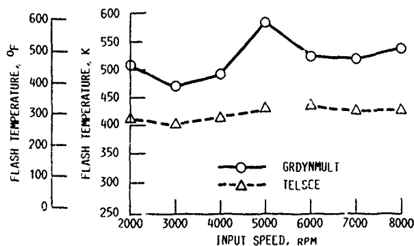
Figure 38.—Comparison of programs GRDYNMULT and TELSGE. Maximum flash temperature as function of input speed. Input torque = 203.4 N·m (Table VIII, runs, 5-11).
