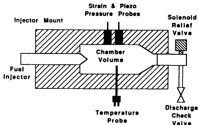
Fig. 2. Schematic of the Zuech rate of injection meter.
