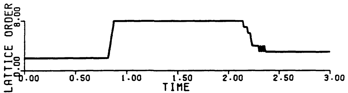
Figure 5.5. Controller Order Variable Payload Mass = 0.1 x Flexible Link Mass Gravity Not Included
