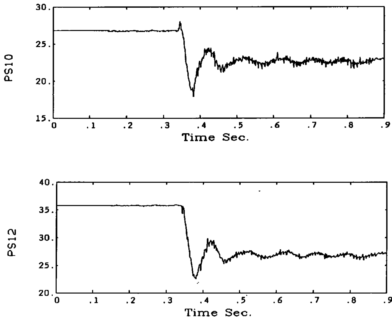
Figure 4.5.2 Resampled, Filtered and Averaged Static Pressure Measurements at Stages 8 and 10
