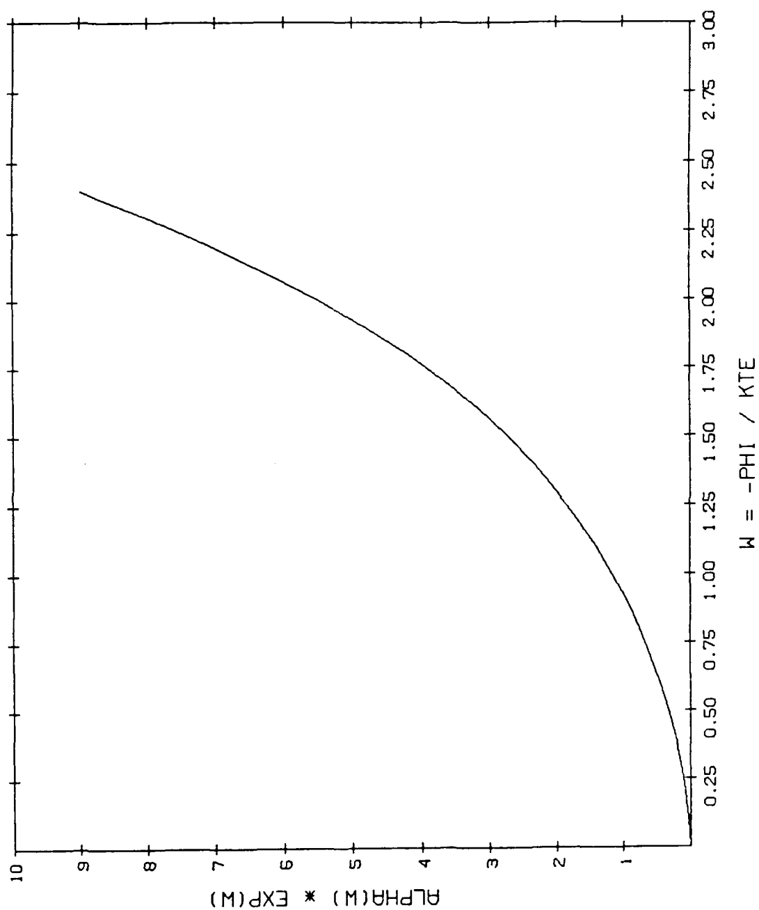
Figure 5. Trapped electron density \alpha(w) \cdot \exp(w)
