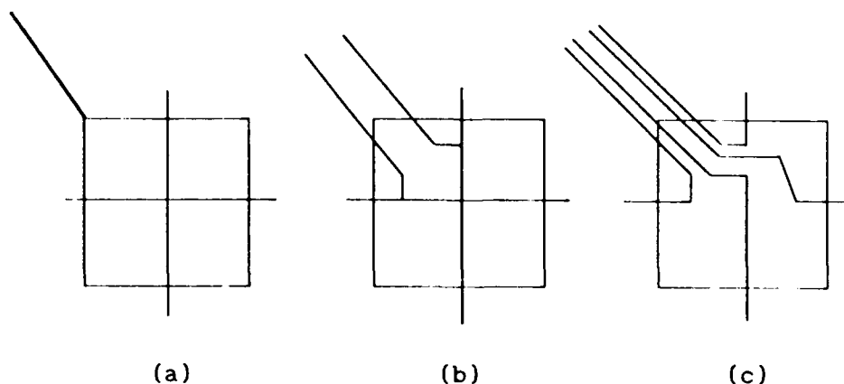
Figure 3.4 Typical switch settings for the reconfigurable mesh model. In (a) the PE is disconnected from row and column busses; in (b) the PE is able to communicate on row and column busses independently; and in (c) the row and column busses are opened and the PE communicates along each bus segment independently.
