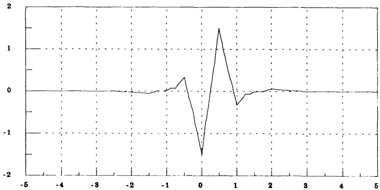
(b) \psi(x)
