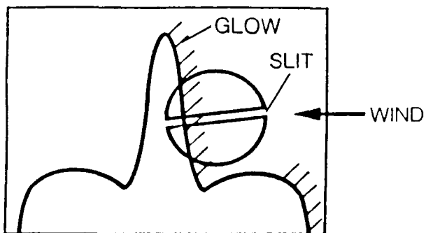
Figure 8.a. Glow spectra
