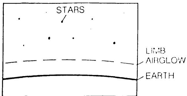
Figure 8.b. Window glow
