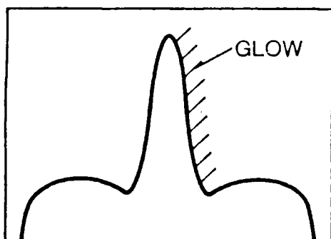
Figure 8.c. Glow image
