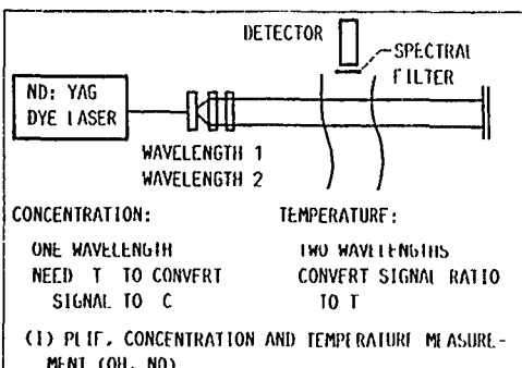
FIGURE 6. - INSTRUMENTATIONS AND ADVANCED DIAGNOSTIC TECHNIQUES.
