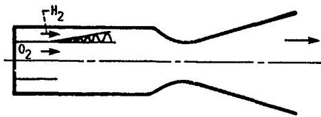
FIGURE 1. - HYDROGEN-OXYGEN MIXING LAYER OF THRUSTER CAN BE WELL SIMULATED WITH A PRSL FACILITY.
