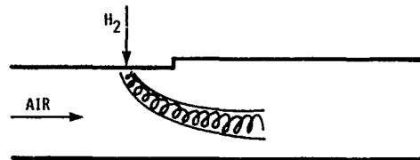
FIGURE 2. - HYDROGEN FUEL JET WITH AIR CROSSFLOW MIXING IS SIMULATED IN A 2-D PLANE SHEAR LAYER.
