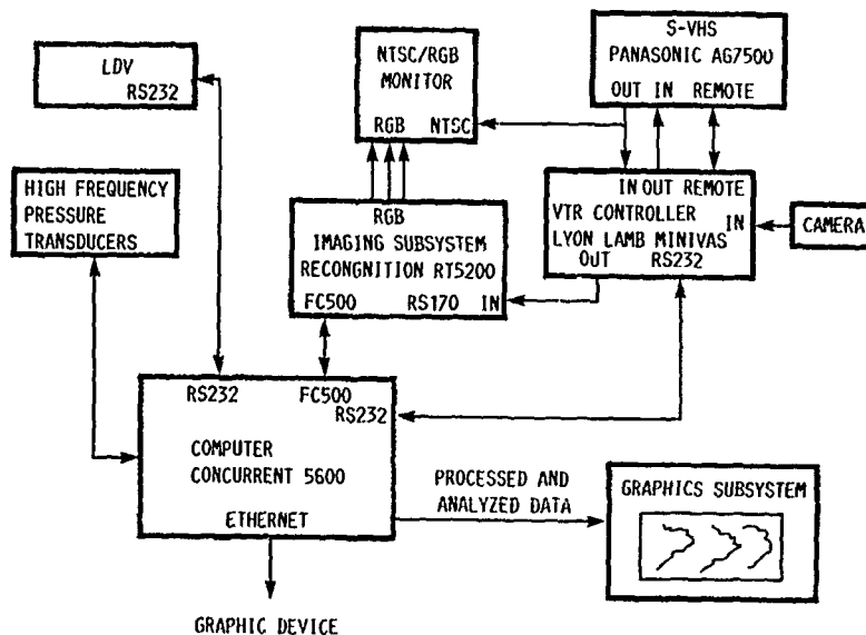
FIGURE 8. - PRSL IMAGING SYSTEM FLOW CHART.
