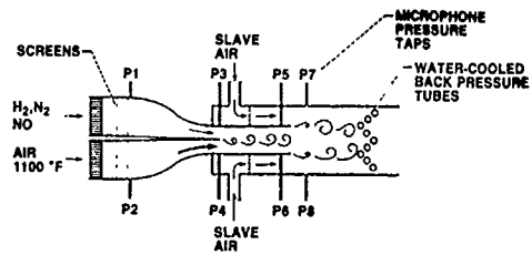
FIGURE 5. - MICROPHONE LOCATIONS (PRSL TEST SECTION).
