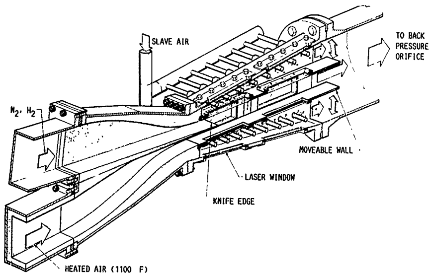
FIGURE 4. - PRSL TEST SECTION.
