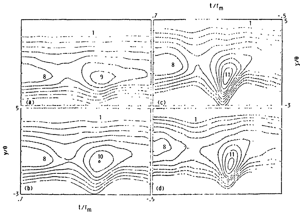
FIGURE 10. - -D_z CONTOURS AT: (a) \times 150 \theta_0 , (b) 300 \theta_0 , (c) 600 \theta_0 AND (d) 4800 \theta_0 FROM REF. 11.
