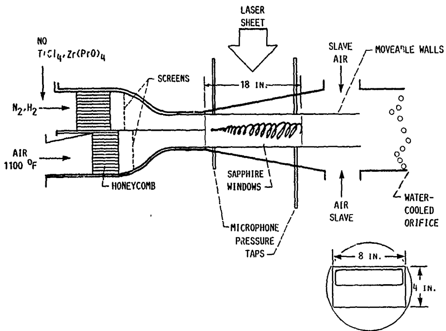
FIGURE 7. - LOCATION OF THE LASER SHEET IN THE FACILITY.
