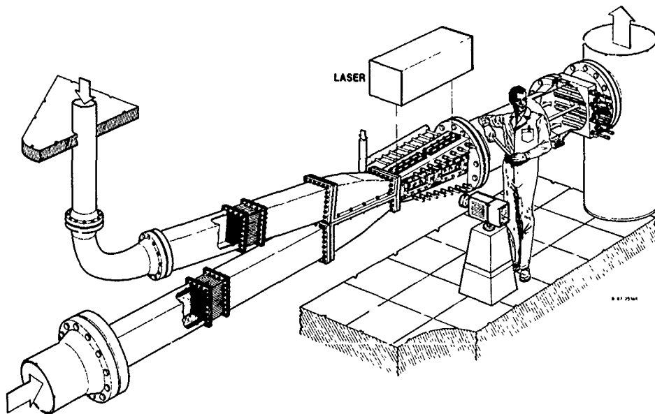
FIGURE 3. - A SCHEMATIC OF THE PRSL FACILITY.
