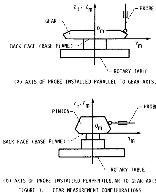
FIGURE 1. - GEAR MEASUREMENT CONFIGURATIONS.
