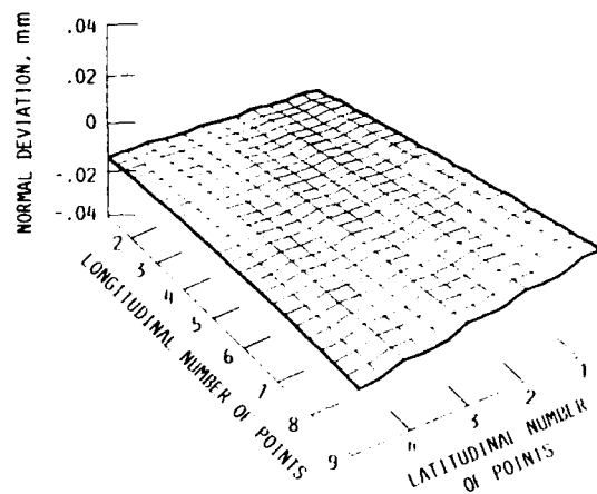
FIGURE 9. - DEVIATION OF FITTED IMAGE SURFACE \Sigma_t .
