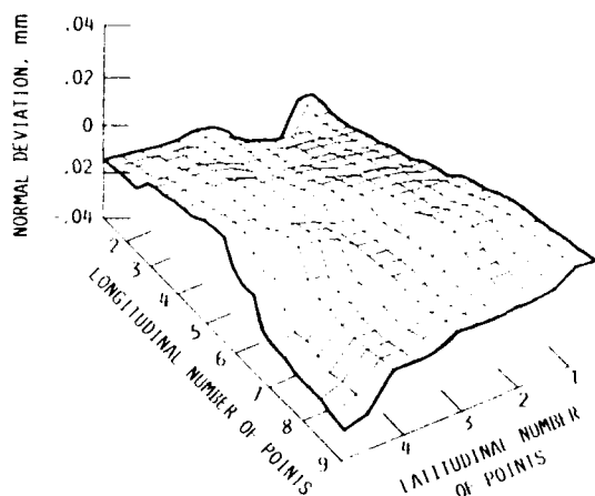
FIGURE 7. - DEVIATION OF IMAGE SURFACE \Sigma_f .
