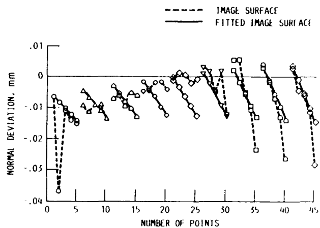
FIGURE 8. - PLOT OF DEVIATIONS OF IMAGE SURFACE \Sigma_f AND FITTED IMAGE SURFACE \Sigma_t .
