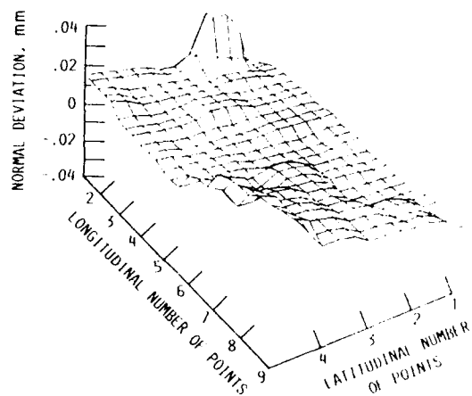
FIGURE 5. - DEVIATION OF REAL SURFACE \Sigma_r .
