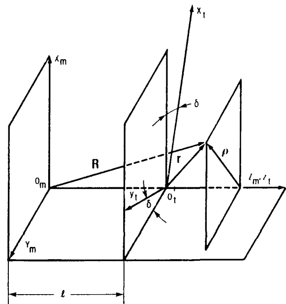
FIGURE 2. - COORDINATE TRANSFORMATION.
