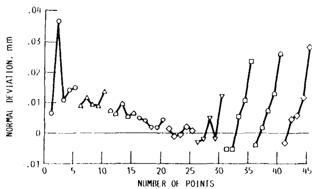
FIGURE 6. - PLOT OF DEVIATION OF REAL SURFACE \Sigma_r .
