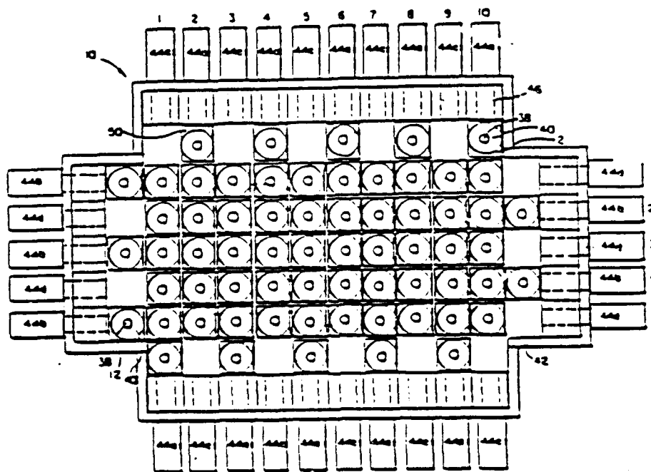
FIGURE 1. Loom Schematic
