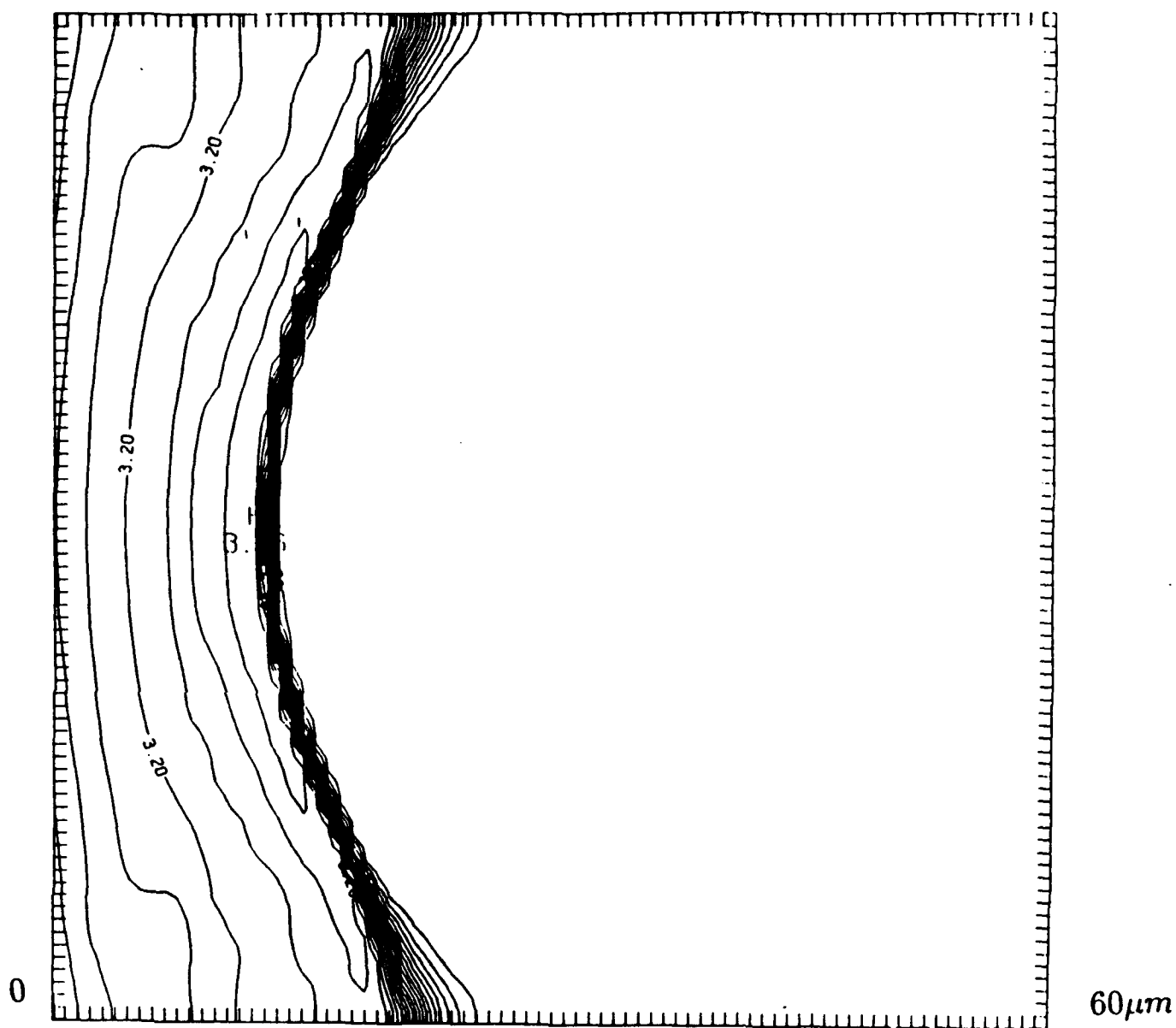
5. Isodensity contours of an 80 \mu m thick CH target impacted with a laser with an imposed 4:1 sinusoidal asymmetry. The time is 9.5 ns, the transverse dimension is 160 \mu m and the horizontal dimension is 60 \mu m .
