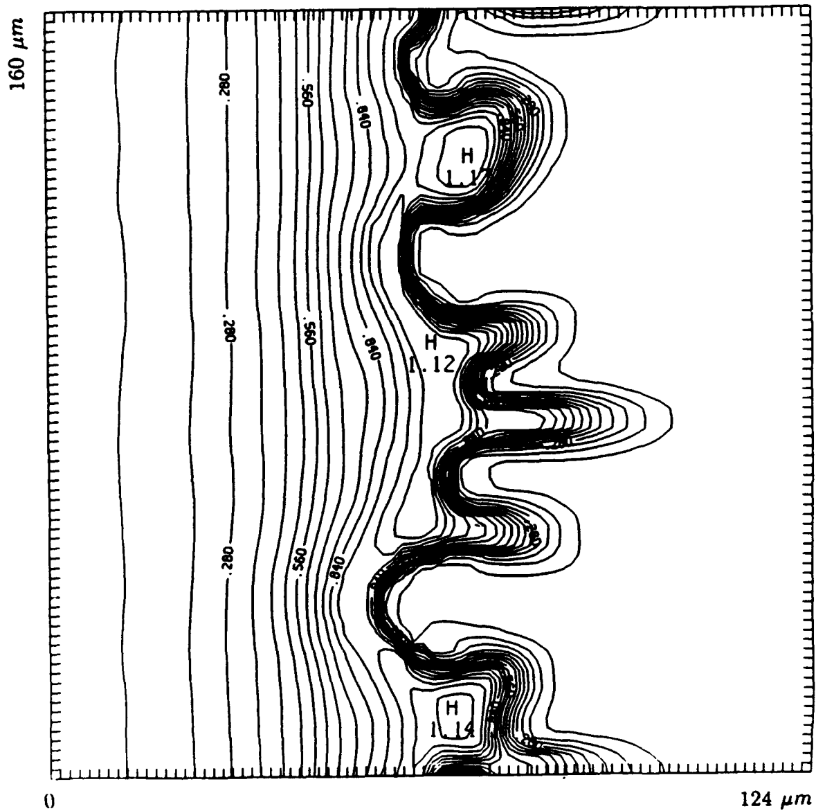
12. Isodensity contours at 12 ns for a 330 \mu m thick DT target illuminated with a 0.264 \mu m ISI laser beam with a power law time dependence. The horizontal dimension is 124 \mu m and the transverse dimension is 160 \mu m .
