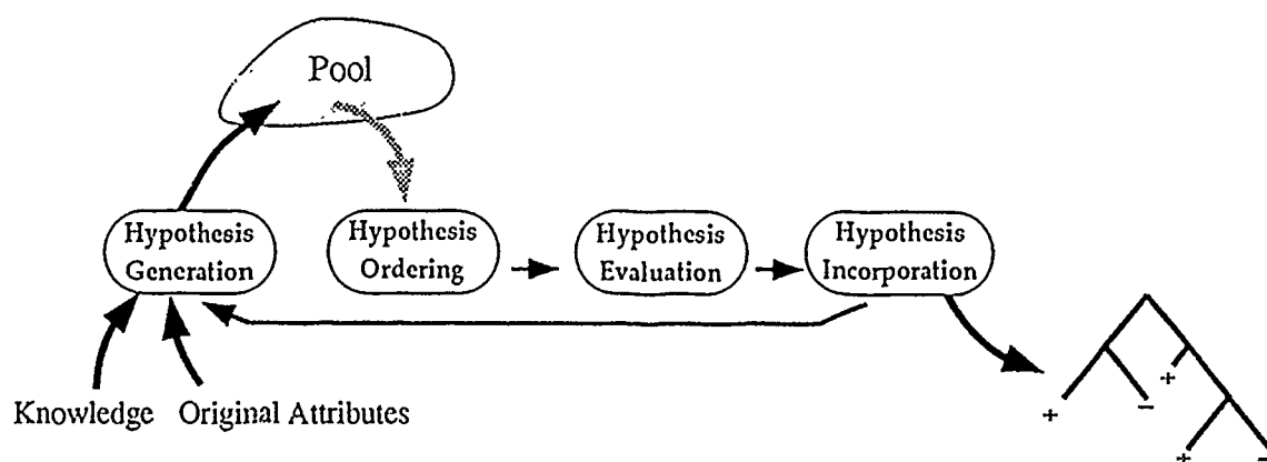
Figure 2.3 Opportunistic Constructive Induction of Decision-Trees.
