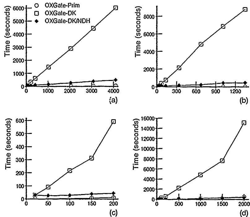
Figure 5.40 Processing Times. Key: (a) Boolean 4-term 3*DNF, (b) Nominal Concept B, (c) Breast Cancer Concept, (d) NetTalk Silent Concept.
