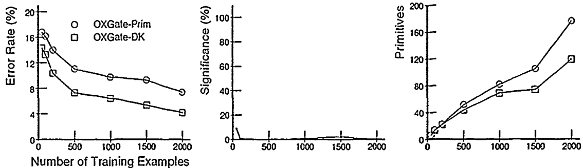
Figure 5.9 Application of Constructed Hypotheses. The inclusion of constructed hypotheses based on domain knowledge (DK) provides a pronounced improvement over the original (Prim) description language.
