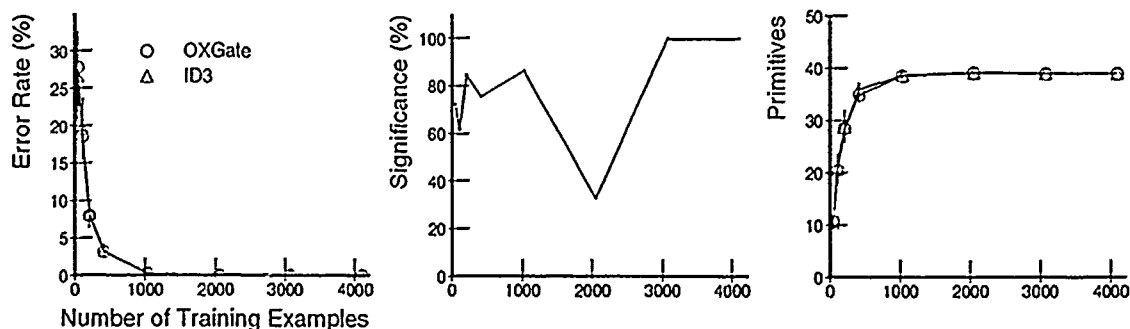
Figure 5.2 Representation Baseline: Boolean 3-Term 3DNF (Unordered). Unordered hypotheses in OXGate cause different decision-trees to be formed than with ID3. The significance curve suggests no preferred representation.
