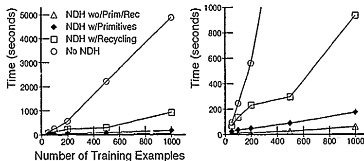
Figure 5.26 Processing Time Comparisons. The left graph shows the relative processing times of hypothesis ordering without the retention of primitive hypotheses or recycling of rejected hypotheses (NDH wo/Prim/Rec), with the retention of primitive hypotheses (NDH w/Primitives), with the recycling of rejected hypotheses (NDH w/Recycling), and using the full set of constructed and primitive hypotheses without ordering (No NDH). The right graph is a closeup of the faster processes. (Note: The number of training examples used is terminated at 1000 due to the large processing time requirements of No NDH.)
