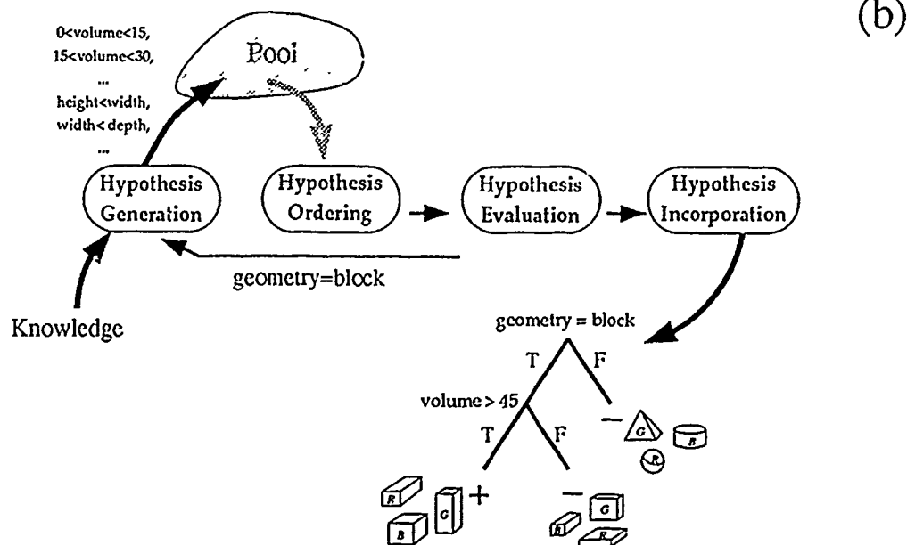
Figure 2.5 Using Knowledge Opportunistically. In part (a), the knowledge about the type of problem is used in conjunction with the original attributes to propose a set of primitive hypotheses to begin induction. One of the hypotheses, ( geometry = block ), is selected to begin the decision-tree. In part (b), this initial selection triggers the proposition of more hypotheses, based on domain knowledge about blocks (e.g., relationships among dimensions, construction of volume , etc.). The opportunistic constructive induction system can then discover the proper description: (( geometry = block ) AND ( volume > 45 )).
