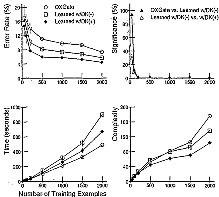
Figure 6.6 Adding Correct Knowledge: NetTalk Silent Concept.
