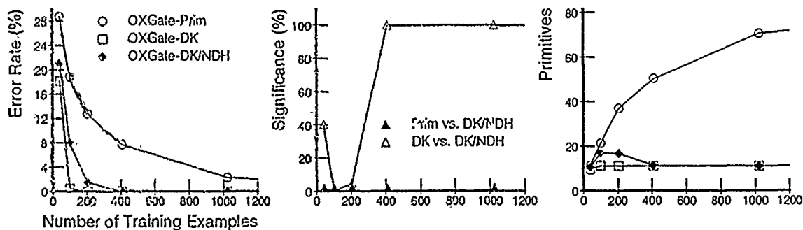
Figure 5.36 Effects of Hypothesis Ordering: Boolean 4-term 3*DNF. The use of constructed hypotheses (DK) exhibits a vast improvement in predictive accuracy and tree conciseness over the use of primitives alone (Prim), indicating that the knowledge applied was proper for this concept. Hypothesis ordering (DK/NDH) rescinded some of the accuracy improvements for the smaller sizes of training data.
