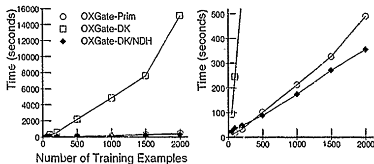
Figure 5.11 Effect of Hypothesis Ordering on Speed. The left-hand graph shows the average processing times of the three approaches. Hypothesis ordering (OXGate-DK/NDH) provides an impressive speed improvement over OXGate-DK, the non-ordered approach (up to 43 times faster). The right hand graph is a closeup of the data. With the NetTalk Silent concept, hypothesis ordering was even faster than using only the primitive hypotheses (OXGate-Prim), significant at \alpha < 0.0035 .
