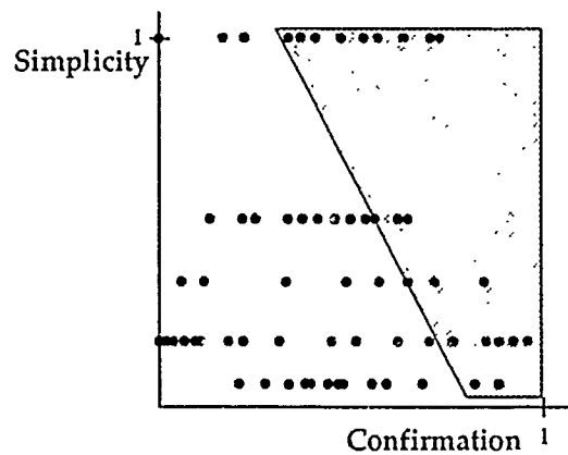
Figure 4.5 Weighted MOE in OXGate. This diagram illustrates the primary partition of hypotheses as applied to the weighted sum of the Quick-Look measure of confirmation and simplicity. (cf. Figure 4.3)
