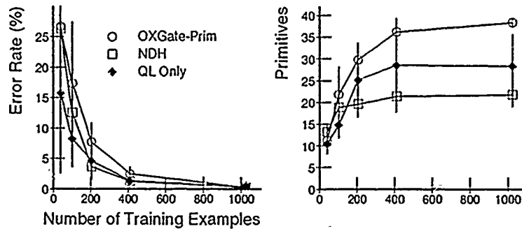
Figure 5.15 MOE vs. SOE: Non-Domination, Boolean 3-term 3DNF. Comparison of the non-domination approach to multiple-objective evaluation using the Quick-Look confirmation measure and simplicity (NDH) versus single-objective evaluation with the Quick-Look confirmation measure alone (QL Only), and single-objective evaluation with simplicity only (OXGate-Prim). This experiment shows marginal improvement in predictive accuracy for NDH over QL Only, but a substantial improvement in tree conciseness when using multiple-objective evaluation for hypothesis ordering. Note also the relative unpredictability (high variance) of the complexity of decision-trees for QL Only as indicated by the error bars.
