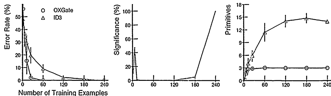
Figure 5.5 Representation Baseline: Nominal Concept C. The performance of OXGate is substantially better than that of ID3 for this concept.
