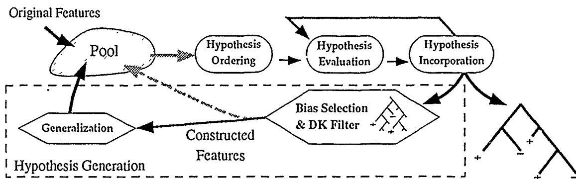
Figure 2.9 Constructive Induction in CITRE.
