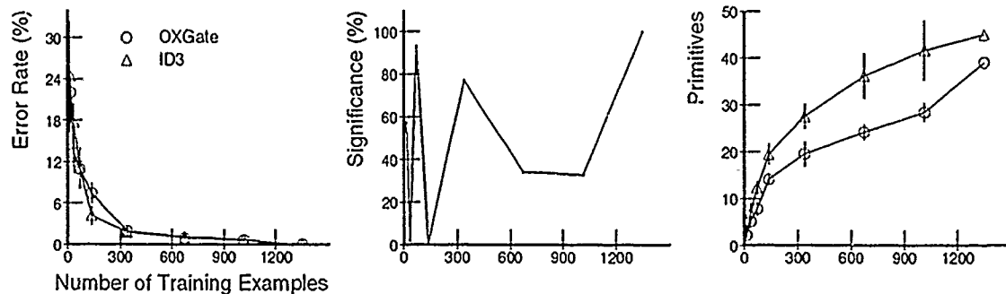
Figure 5.4 Representation Baseline: Nominal Concept B. ID3 is not significantly better than OXGate, because the concept is only partially structured in an n-way decision form.
