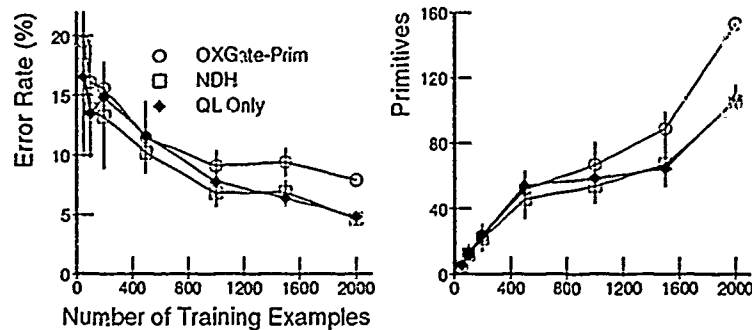
Figure 5.17 MOE vs. SOE: Non-Domination, NetTalk Silent Concept. In this set of experiments, the multiple objective approach (NDH) appears slightly better than both of the single-objective evaluation approaches.
