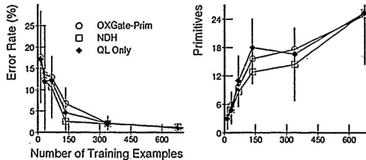
Figure 5.16 MOE vs. SOE: Non-Domination, Nominal Concept B. In this set of experiments, the multiple objective approach (NDH) appears slightly better than both of the single-objective evaluation approaches.
