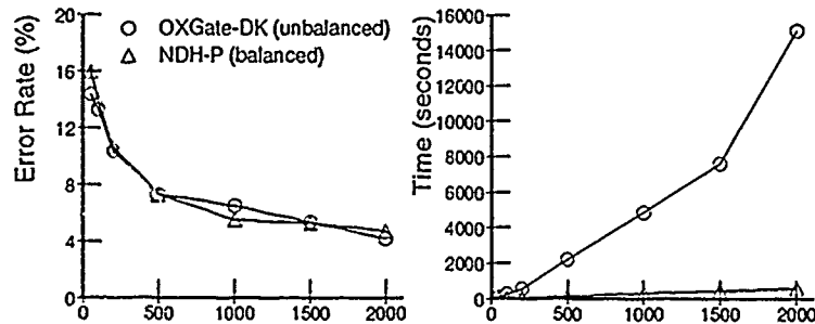
Figure 5.30 Overall Performance Improvement with Balanced Data. When using both the retention of primitive hypotheses and balanced data (NDH-P), hypothesis ordering has a nearly identical predictive accuracy as the non-ordered use of the full set of constructed hypotheses (OXGate-DK) on the original training data. NDH-P (balanced) also nets up to a 25-fold increase in processing speed over OXGate-DK (unbalanced). (Confidence intervals omitted for clarity.)
