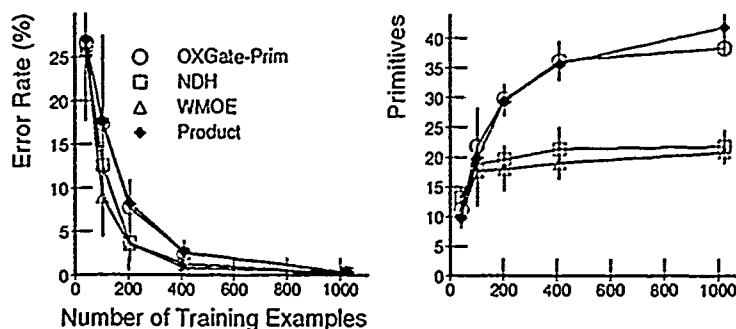
Figure 5.20 Combination Methods: Boolean 3-term 3DNF.
