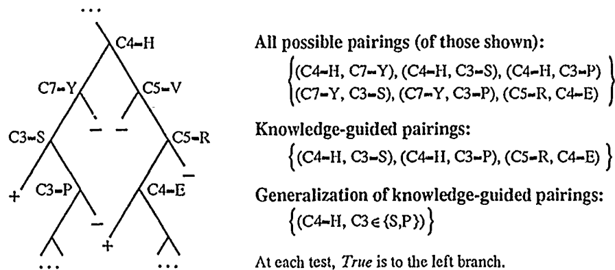
Figure 6.1 Learning from Experience. This example shows a possible portion of a decision-tree for the NetTalk Silent concept to illustrate the search for useful constructs. Positive tests leading to positive leaves are the operands (pairings) for forming binary conjunctions. Domain knowledge can be used to constrain the possible combinations. The effect of applying a domain-independent generalization operator, the merging of disjunctive regions, is also shown. The decision-tree is learned from a collection of seven-character windows (C1 through C7) on a dictionary of words. An example of such a window is from the word “symphony,” with the letter “h” as the center character: s[ym(p(h)ony]. This window corresponds to the pairings (C4=H, C7=Y) , (C4=H, C3=P) , and (C7=Y, C3=P) , and supports the generalization (C4=H, C3 \in \{S, P\}) . A word that provides multiple windows with silent center characters is “haberdashery”: [hab(e)rda] and [ash(e)ry.] both support (C5=R, C4=E) ; and [das(h)ery] supports (C4=H, C7=Y) , (C4=H, C3=S) , (C7=Y, C3=S) , and the generalization (C4=H, C3 \in \{S, P\}) .
