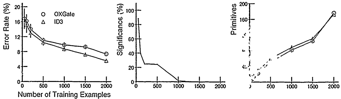
Figure 5.6 Representation Baseline: NetTalk Silent Concept. ID3 appears substantially better than OXGate for this NetTalk concept when using the larger training set sizes.
