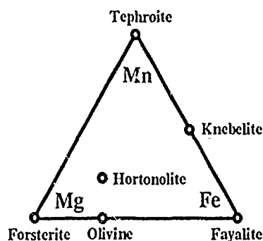
Figure 3.2 Mineralogical Isomorphism. The olivine series of the silicate class of minerals. The triangle depicts the isomorphism caused by the three-way mutual substitution of magnesium (Mg), iron (Fe), and manganese (Mn) in the crystal lattice. The locations of the minerals on the triangle indicate the typical ratios of the three elements. Although the triangle depicts precise locations for the minerals (for example, the composition of olivine has a ratio of Mg to Fe atoms and, therefore, the ratio of ideal forsterite to ideal fayalite, of 63:37), any ratio is possible in nature; hence, the boundaries between minerals in the series are imprecise.
