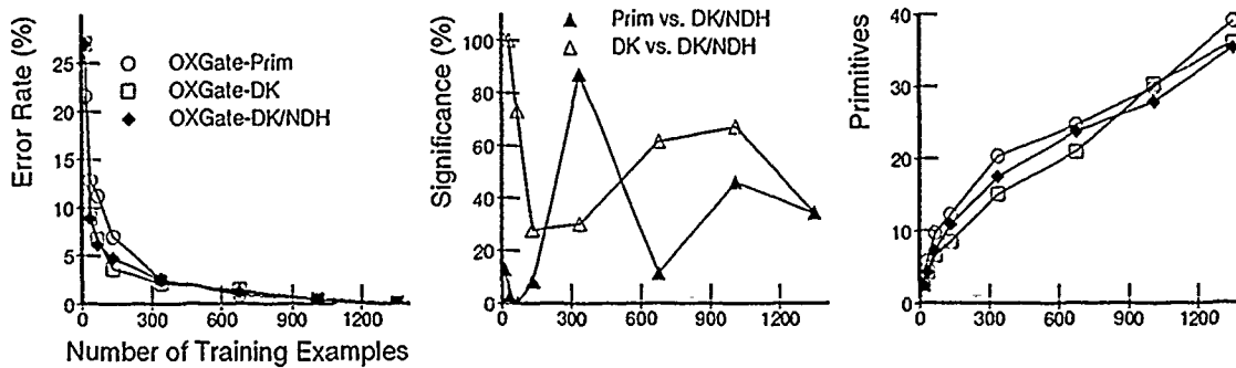
Figure 5.37 Effects of Hypothesis Ordering: Nominal Concept B. The use of constructed hypotheses (DK) exhibits a small, albeit inconsistent, improvement in accuracy and conciseness over the use of primitive hypotheses alone (Prim). Hypothesis ordering (DK/NDH) appears to have little detrimental effect on the predictive accuracy.
