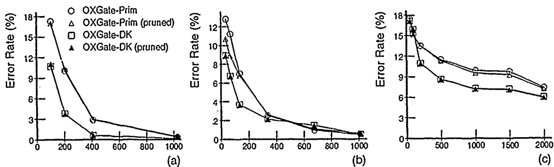
Figure 5.33 Effects of Pruning. The graphs show the effect of post-pruning decision-trees created with the original primitive hypotheses ( OXGate-Prim ) and constructed hypotheses ( OXGate-DK ). Hypothesis ordering was disabled. Key: (a) Boolean 3-Term 3DNF, (b) Nominal Concept B, (c) NetTalk Silent Concept.
