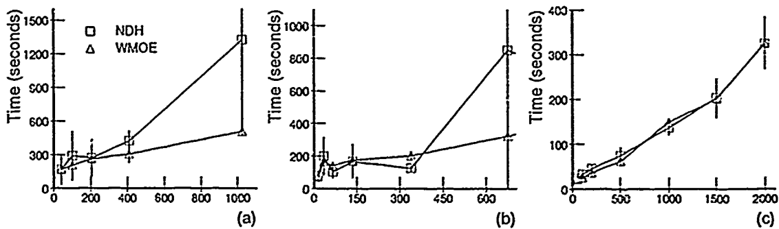
Figure 5.23 Combination Methods: Processing Time Comparison. Key: (a) Boolean 3-term 3DNF, (b) Nominal Concept B, (c) NetTalk Silent Concept.
