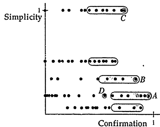
Figure 4.3 Non-Dominated Hypotheses in OXGate. The diagram shows the use of the tolerance band for the primary subset of hypotheses. The tolerance band for the secondary subset is not shown. The tolerance band is applied for the Quick-Look measure of confirmation, but is not necessary for the precisely determinable dimension of simplicity. (Note the discrete nature of the simplicity measure used by OXGate.)
