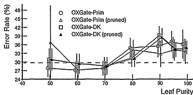
Figure 5.35 Pruning with the Breast Cancer Concept. In these experiments, decision-trees were developed using 200 examples of the Breast Cancer database, and tested on the remaining 86 examples. The graph shows the results for several leaf purities (50%, 60%, 70%, 80%, 90%, 95%, and 99%) used to determine when to stop splitting. The dashed line indicates the error-rate of chance. The four error bars clustered at each chosen leaf purity value are spread apart for clarity of presentation. The 95% confidence intervals are shown to demonstrate the erratic behavior with this domain.
