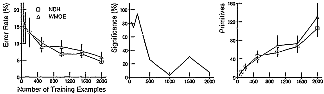
Figure 5.22 Combination Methods: NetTalk Silent Concept.
