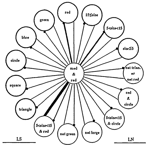
Figure 2.11 Concept Description Support in STAGGER. Pictorial representation of the support for the concept ( medium AND red ). The lines terminated with small dots represent the logical sufficiency (LS), the others represent logical necessity (LN). The thickness of a line is indicative of the degree of logical necessity or sufficiency the associated hypothesis provides for the target concept.
