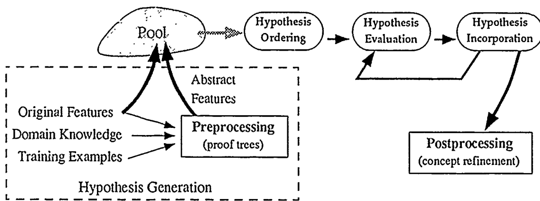
Figure 2.10 Constructive Induction in MIRO.
