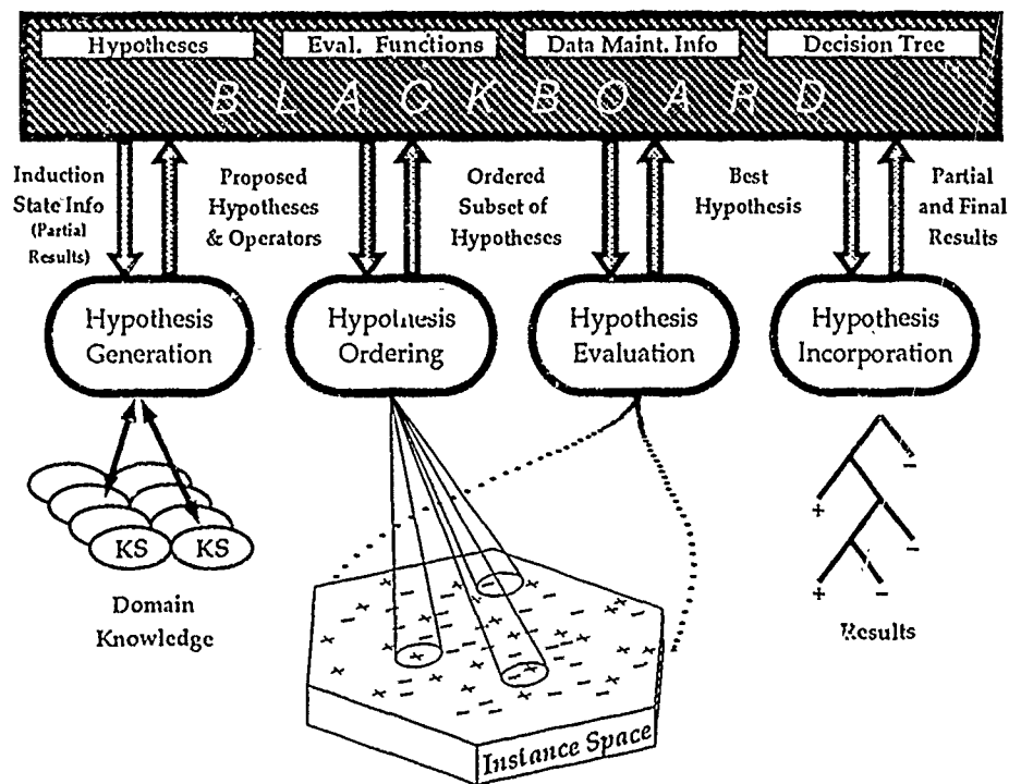
Figure 3.1 The OXGate System Architecture. The four components of the inductive process communicate with each other through the blackboard. The blackboard maintains the set of potentially useful hypotheses, the available evaluation functions, and the bookkeeping information to index hypotheses and instances to the relevant nodes of the developing decision-tree.
