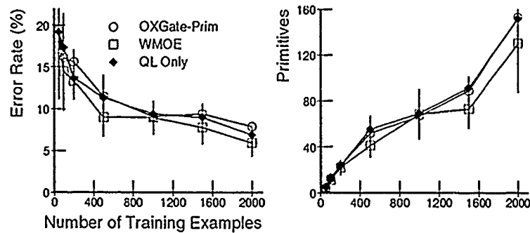
Figure 5.14 MOE vs. SOE: Weighted Combination, NetTalk Silent Concept. Although not as dramatic as in Figure 5.12, the multiple-objective approach (WMOE) is still noticeably superior to both of the single-objective evaluation approaches.
