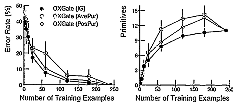
Figure 5.18 Information-Gain versus Purity Measures. Comparison of three confirmation measurement methods on the induction of Nominal Concept A. In each run, the sixteen primitive hypotheses were used as the pool of available hypotheses. Hypothesis ordering was disabled; the comparison is between the measurements used for hypothesis evaluation. Key: Information-Gain (IG), Average Purity (AvePur), Positive Purity (PosPur).
