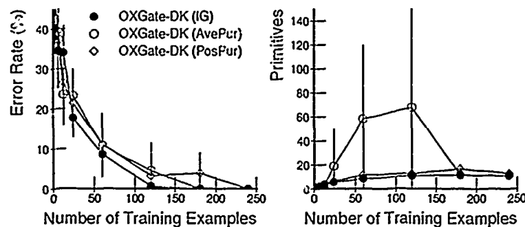
Figure 5.19 Information-Gain versus Purity Measures: With Knowledge. Comparison of three confirmation measures under the same conditions as in Figure 5.18, except the pool of hypotheses includes 1008 constructed hypotheses.
