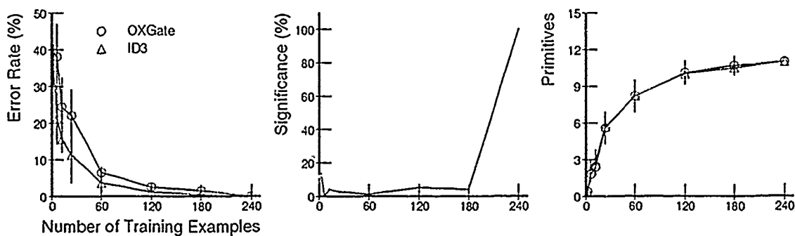
Figure 5.3 Representation Baseline: Nominal Concept A. ID3 is substantially better than OXGate on this concept because it is structured in an n-way decision form.
