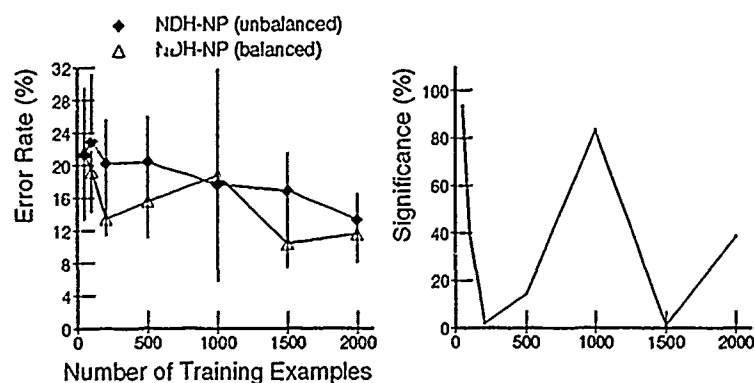
Figure 5.28 Using Balanced Data Without Retaining Primitives. Simply balancing the training data is not enough to stably improve hypothesis ordering as shown by the somewhat better, but still erratic, performance of hypothesis ordering without the retention of primitives.
