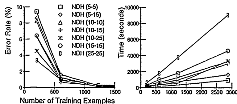
Figure 5.31 Tolerance Band Assessment: Boolean 4-term 3*DNF.
