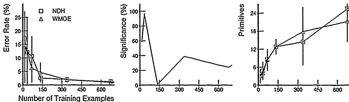
Figure 5.21 Combination Methods: Nominal Concept B.
