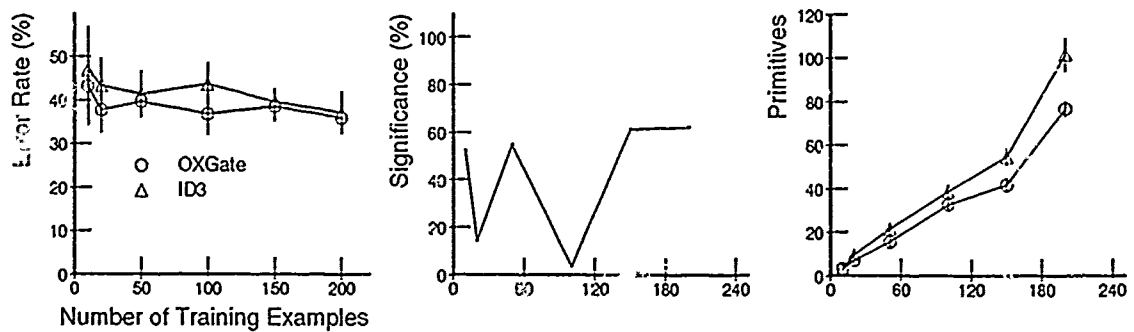
Figure 5.7 Representation Baseline: Breast Cancer Concept. OXGate appears generally better than ID3 for the breast cancer concept.
