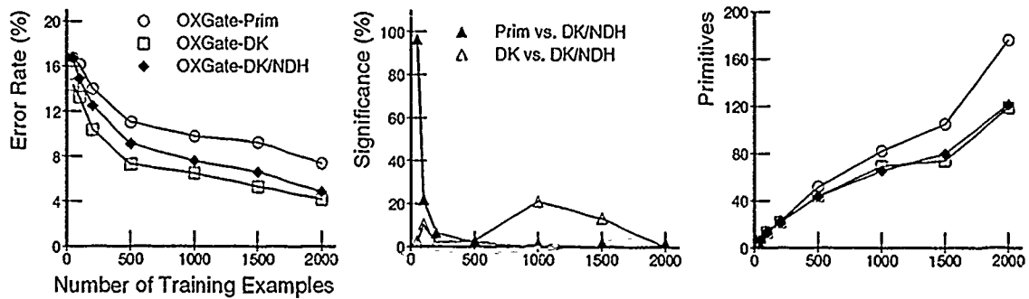
Figure 5.39 Effects of Hypothesis Ordering: NetTalk Silent Concept. Repeat of Figure 5.10, included for completeness. The use of hypothesis ordering (DK/NDH) causes some loss of predictive accuracy over the non-ordered approach (DK), yet is substantially better than using no constructed hypotheses at all (Prim).
