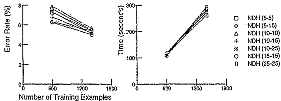
Figure 5.32 Tolerance Band Assessment: NetTalk Silent Concept.
