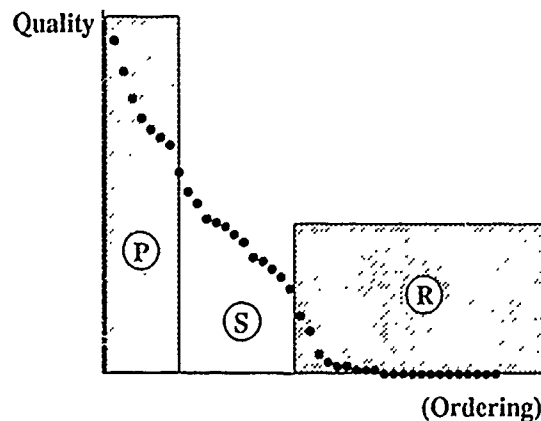
Figure 4.7 The Histogrammatic Approach to Partitioning.
