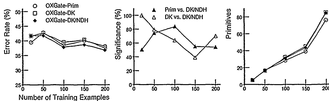
Figure 5.38 Effects of Hypothesis Ordering: Breast Cancer Concept. The significance curves indicate very little support for concluding that one approach is better than another.
