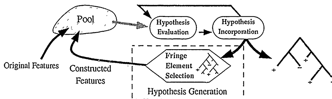
Figure 2.7 Constructive Induction in FRINGE.
