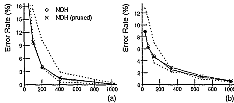
Figure 5.34 Pruning with NDH. Post-pruning had a negligible effect on the decision-trees developed using hypothesis ordering on the sets of constructed hypotheses. Key: (a) Boolean 3-Term 3DNF, (b) Nominal Concept B. The dashed curves represent the envelopes of the corresponding graphs of Figure 5.33, shown for comparison.
