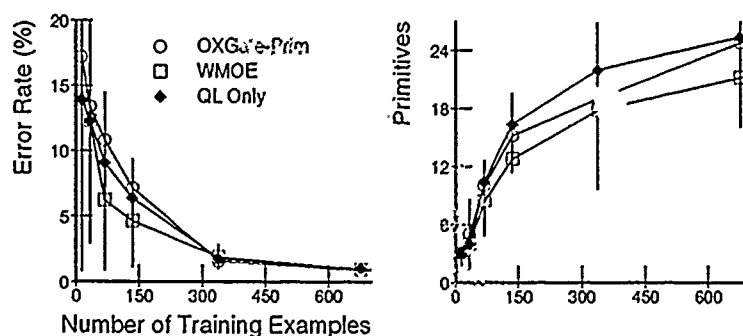
Figure 5.13 MOE vs. SOE: Weighted Combination, Nominal Concept B. Although not as dramatic as in Figure 5.12, the multiple objective approach (WMOE) is still noticeably superior to both of the single-objective evaluation approaches.
