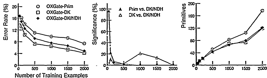
Figure 5.10 Effects of Hypothesis Ordering. With the NetTalk Silent concept, hypothesis ordering (DK/NDH) causes some loss of prediction over the non-ordered approach (DK), yet is better than using no knowledge. The significance curves contrast the use of primitive hypotheses alone (Prim) with the ordered use of the constructed hypotheses (DK/NDH), and the ordered (DK/NDH) with the non-ordered (DK) uses of constructed hypotheses.
