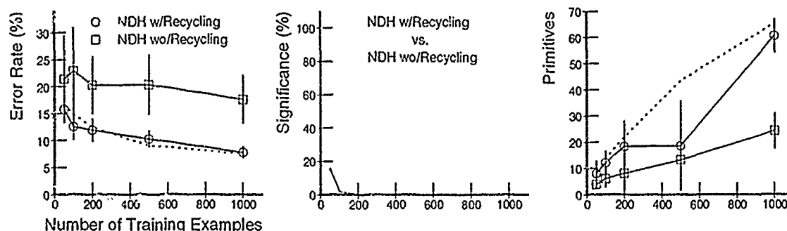
Figure 5.25 The Effect of Recycling Rejected Hypotheses. Reusing previously rejected hypotheses substantially improves the accuracy of hypothesis ordering. The dashed lines represent the behavior of NDH w/Primitives from Figure 5.24. (Note: The number of training examples used is terminated at 1000 due to the large processing time requirements.)
