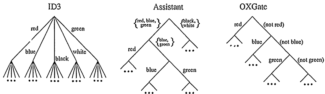
Figure B.1 Contrast of Three Representations. For nominal or discretized numerical scales, such as the attribute color , ID3 performs n-way splitting across an attribute, Assistant performs binarization, and OXGate produces a strictly binary decision-tree representation.
