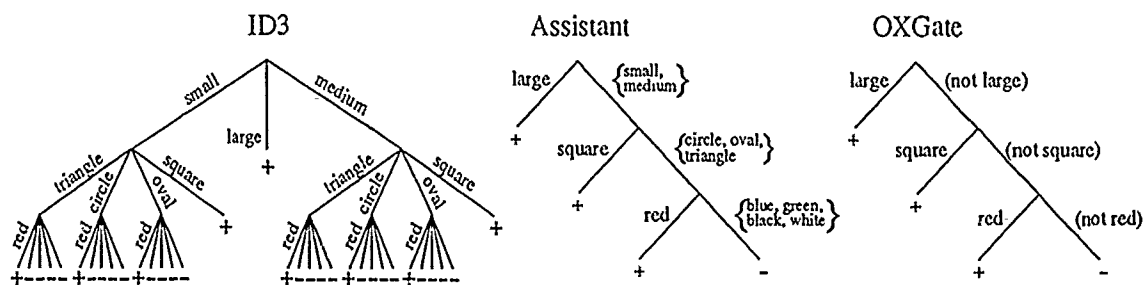
Figure B.2 Comparison of Decision-Trees. The structured splitting method of ID3 (mandatory n-way splitting) puts it at a distinct disadvantage for the concept ((color = red) \text{ OR } (size = large) \text{ OR } (shape = square)) .
