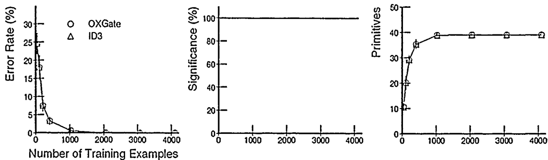
Figure 5.1 Representation Baseline: Boolean 3-Term 3DNF (Ordered). The hypotheses were organized on OXGate's blackboard in the same order in which their equivalents appear internally in ID3. For each set of training data, the decision-trees produced by ID3 and OXGate were identical.
