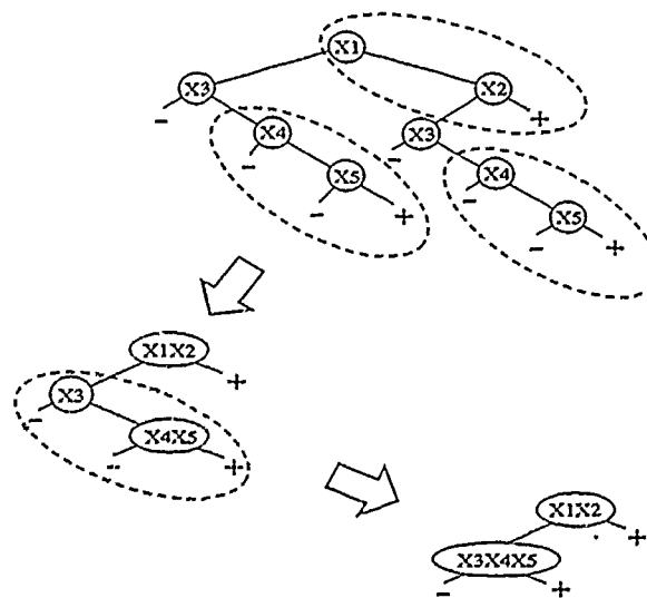
Figure 2.8 Solving the Replication Problem.
