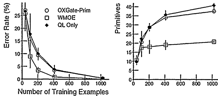
Figure 5.12 MOE vs. SOE: Weighted Combination, Boolean 3-term 3DNF. Comparison of the weighted combination approach to multiple-objective evaluation using the Quick-Look confirmation measure and simplicity (WMOE) versus single-objective evaluation with the Quick-Look confirmation measure alone (QL Only), and single-objective evaluation with simplicity alone (OXGate-Prim). This experiment shows a dramatic improvement in predictive accuracy and tree conciseness when using multiple-objective evaluation for hypothesis ordering.
