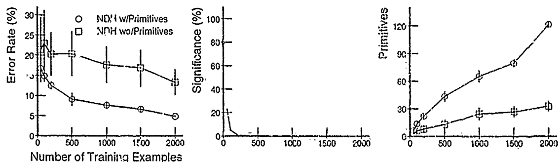
Figure 5.24 The Effect of Retaining the Primitive Hypotheses. Retention of the primitive hypotheses greatly improves both the accuracy and the stability of decision-trees created while using hypothesis ordering: NetTalk Silent Concept, 189 primitive and 1460 constructed hypotheses.
