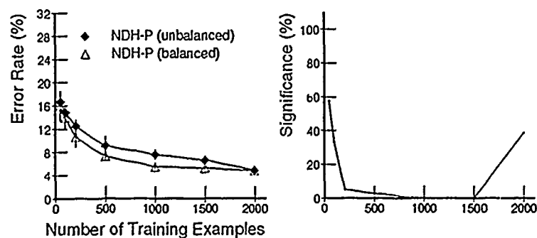
Figure 5.29 Using Balanced Data While Retaining Primitives. When hypothesis ordering retains the primitive hypotheses ( NDH-P ), balancing the training data provides a clear improvement.
