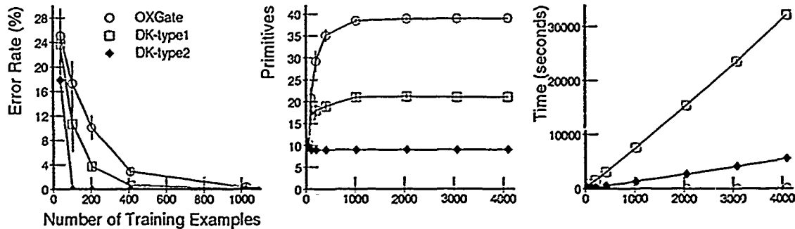
Figure 6.3 Using Correct Knowledge: Boolean 3-term 3DNF. Note: The number of training instances shown for the error-rate is truncated after 1024 examples for clarity of presentation.
