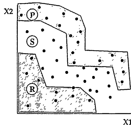
Figure 4.2 Using Tolerance Bands with Non-Domination. The use of tolerance bands avoids overreliance on the quality of estimations X_1 and X_2 . The three bands represent the generally undominated hypotheses (primary subset, P), the heavily dominated hypotheses (rejected subset, R), and the remaining ones (secondary subset, S).
