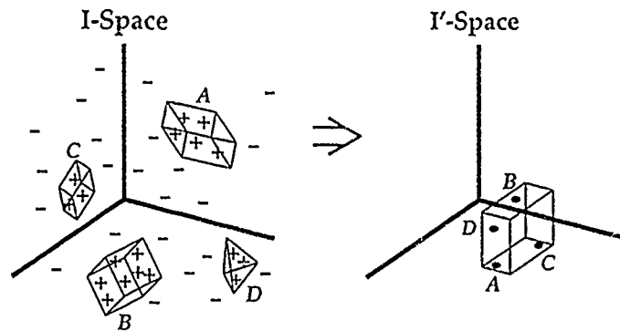
Figure 2.2 Transforming Instance Space. The original instance space (I-Space) is pictured here with a disjunctive collection of islands (conjunctive components or other structures) separating positive from negative instances. Constructive induction transforms I-Space into I'-Space by finding the relationships between the islands and defining new descriptive terms (dimensions in I'-Space), allowing easier concept induction and a more compact description.
