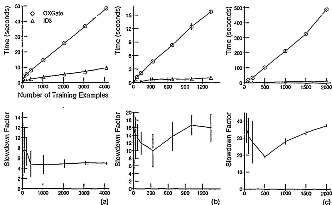
Figure 5.8 Benchmark Speed Comparisons. The overhead of blackboard maintenance and individual hypothesis consideration creates a performance degradation. Key: (a) Boolean 3-term 3DFF Concept, (b) Nominal Concept B, and (c) NetTalk Silent Concept.
