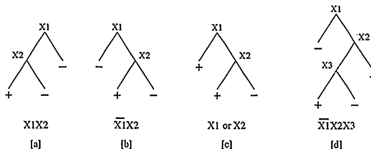
Figure 6.4 Relating Look-Ahead to Hypothesis Construction. Several potential subtrees created with a look-ahead of two ([a], [b] and [c]) and three ([d]) are shown. The equivalent constructed hypotheses are provided below the subtrees.
