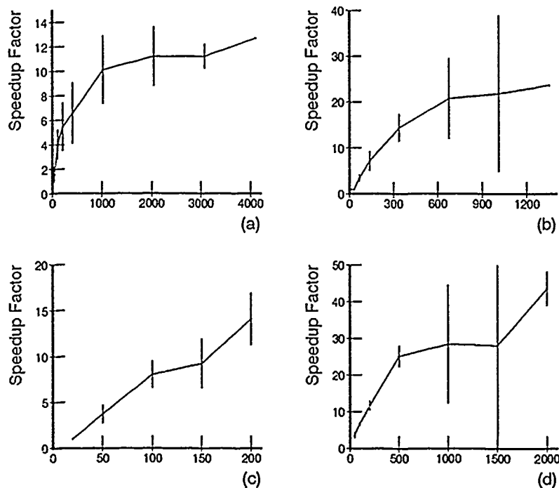
Figure 5.41 Speedup Factors. Comparison of the processing speed improvements provided by hypothesis ordering (OXGate-DK/NDH in Figures 5.36 through 5.40) over the unordered use of the constructed hypotheses (OXGate-DK). Key: (a) Boolean 4-term 3*DNF, (b) Nominal Concept B, (c) Breast Cancer Concept, (d) NetTalk Silent Concept. All data were collected over 10 runs except as noted: (a) used 5 runs with 2048 training examples, 3 runs with 3072, 1 run with 4096; (b) used 5 runs at 675, 3 runs at 1012, 1 run at 1350; (d) used 3 runs at 1000, 2 runs at 1500, 2 runs at 2000. Where fewer than 10 runs were used, the error bars appear abnormally large relative to the rest.
