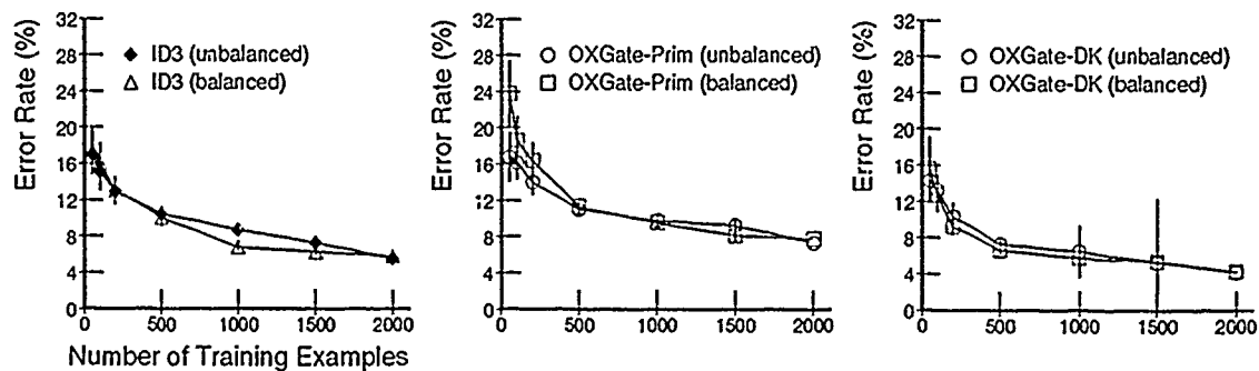
Figure 5.27 Balancing Positive and Negative Examples. The three graphs contrast the use of the original 2000 training examples (unbalanced = 14% positive examples) with the use of the modified training set of 3355 examples (balanced = roughly 50% positive examples). For the "balanced" curves, the Number of Training Examples shown on the abscissa represents the expected number of unique instances used for the decision tree construction; e.g., the set of 3355 actual examples corresponds to the set of 2000 original training instances. 10
