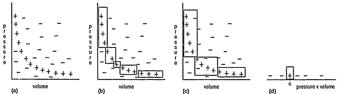
Figure 1.1 Induction of P \times V = C . Example physics problem where pressure times volume is a constant: (a) shows the two-dimensional projection of the examples onto the interesting attributes, (b) illustrates the partitioning for high accuracy, (c) illustrates the partitioning for a concise description, and (d) shows the one-dimensional projection over the constructed attribute, providing both conciseness and accuracy.
