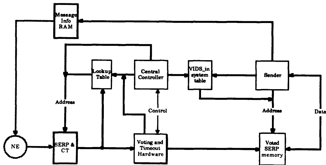
Figure 7-1, High-level Partitions of the Scoreboard
