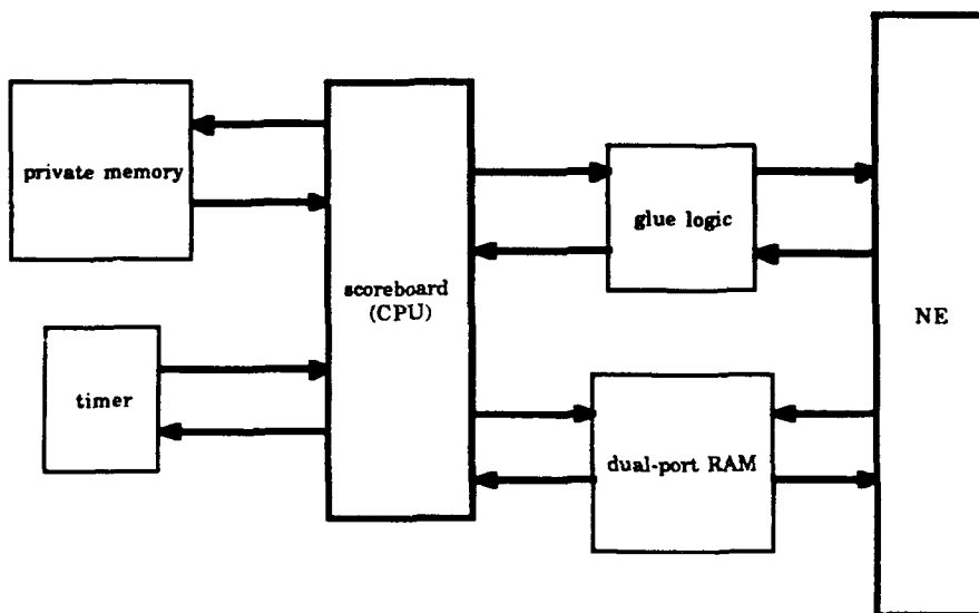
Figure 8-2, RISC scoreboard
