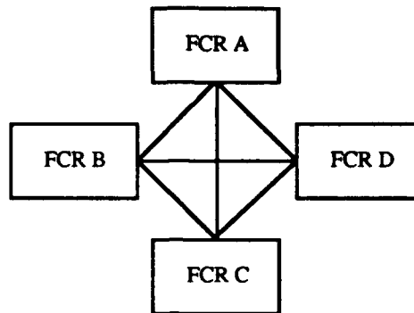
Figure 2-2, Minimal 1-Byzantine Resilient System
