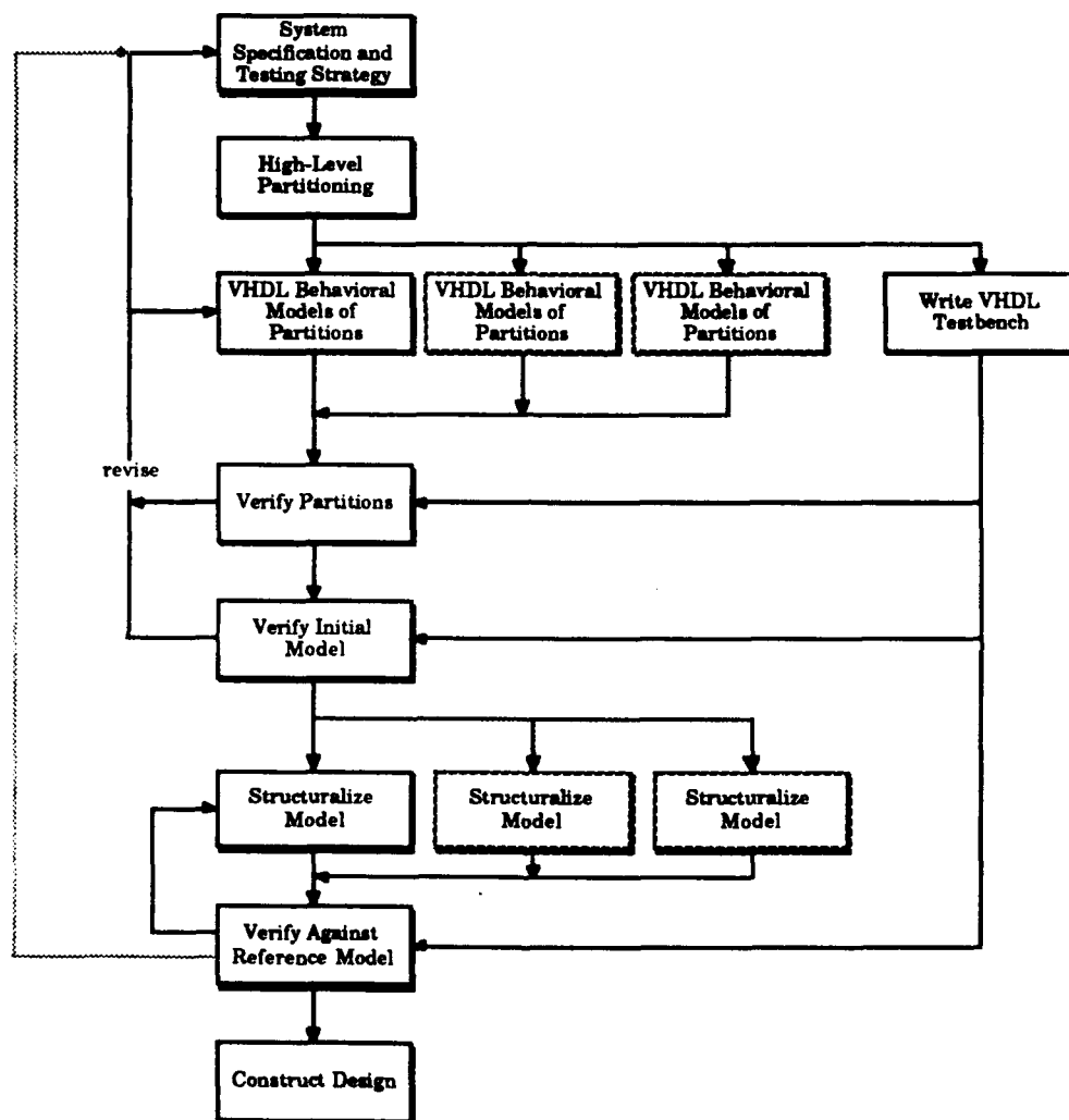
Figure 4-3, Top-Down Design with VHDL
