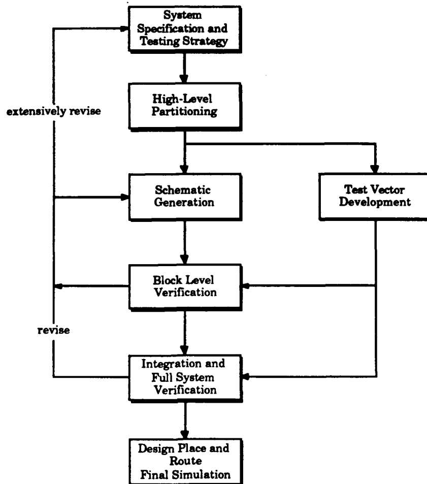
Figure 4-2, Conventional Design
